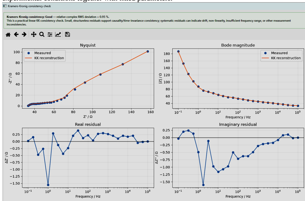
Figure 19: Kramers–Kronig consistency check. The measured data (points) and the KK reconstruction (line) are compared as Nyquist and Bode-magnitude plots, with the corresponding real and imaginary residuals shown below. A small, structureless deviation (here a relative complex RMS deviation of 0.95 %) supports causality and time-invariance, whereas systematic residuals can indicate drift, non-linearity or an insufficient frequency range.
