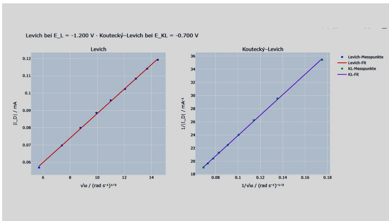
Figure 6: Levich (left) and Koutecký-Levich (right) graphs.
