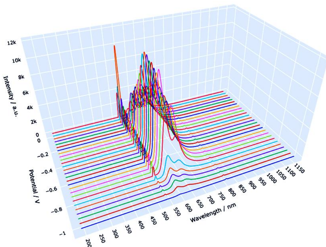
Figure 4: Fluorovoltammogram of rubrene at different potentials.
