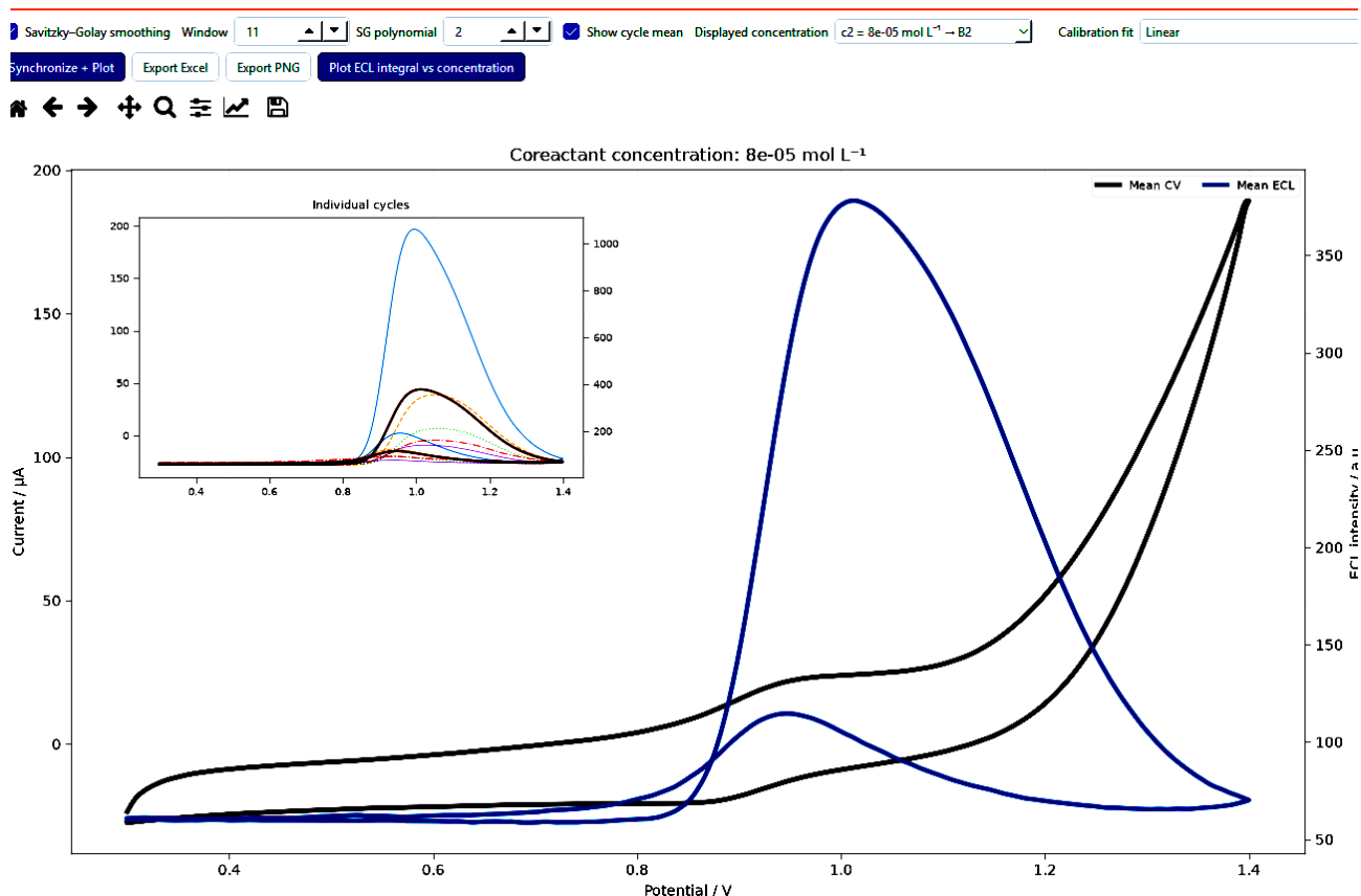
Figure 8: CV (black) and ECL (blue) curves. Average of five scans. Insert: Five individual scans.
