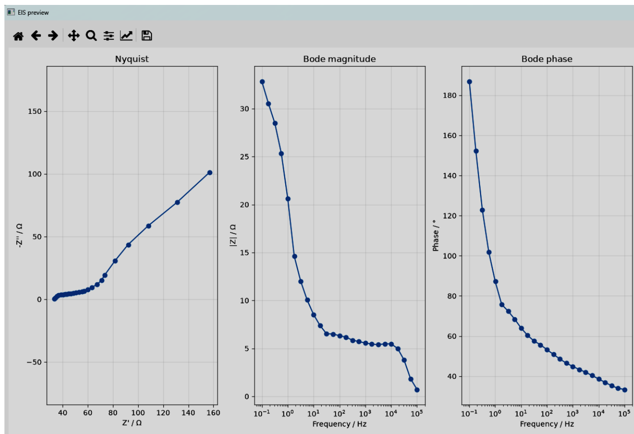
Figure 16: Preview of the imported impedance data before fitting, shown as a Nyquist plot ( -Z'' versus Z' ) together with the Bode magnitude |Z| and the Bode phase \varphi as functions of frequency. Previewing the raw data makes it possible to identify outliers and incomplete frequency regions before an equivalent circuit is applied.
