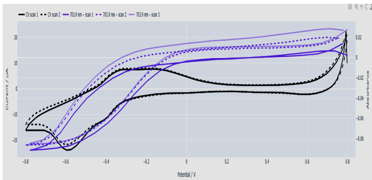
Figure 7: Top: Change in methylene blue absorbance as a function of applied potential. Bottom: Absorptovoltammogram for the selected wavelength (703.9 nm).
