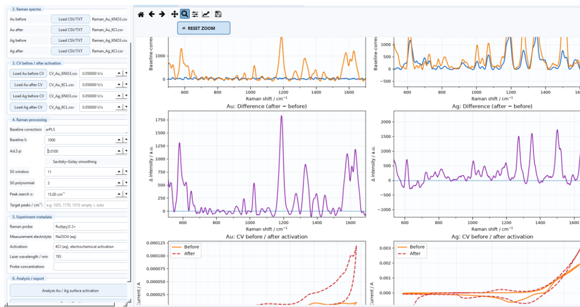
Figure 21: Module 10 overview showing Raman spectra before/after activation, Raman difference spectra and the corresponding Au and Ag cyclic voltammograms.
