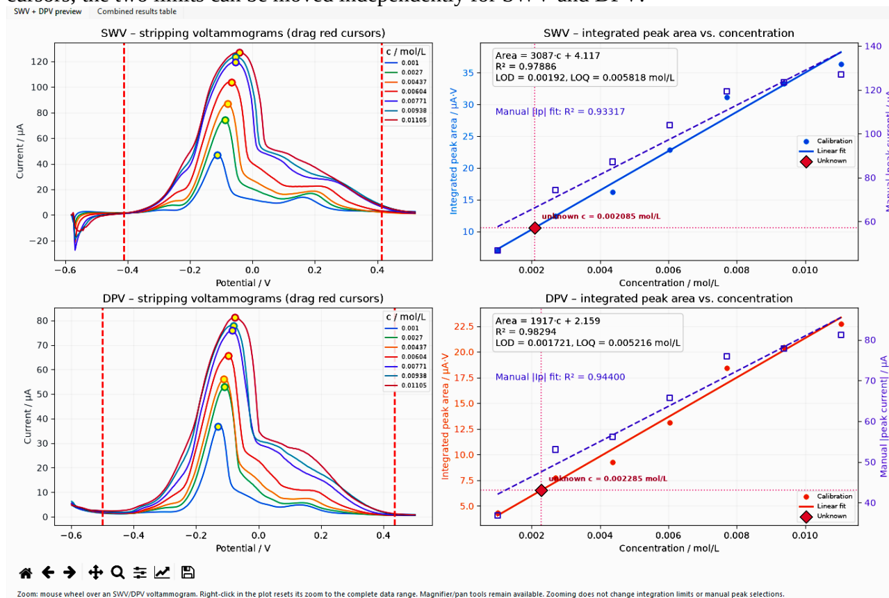
Figure 20: SWV and DPV measurements (left) and integral and peak values as a function of concentration (right). Red square: calculated unknown concentration.
