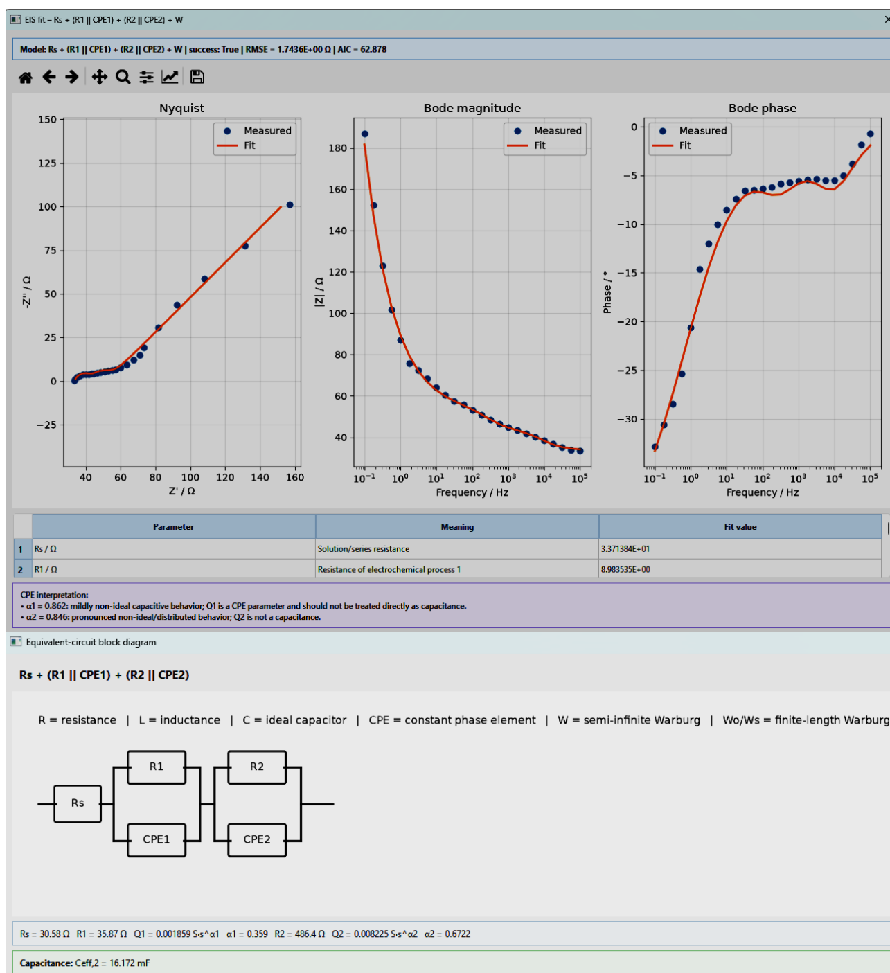
Figure 17: Result of the equivalent-circuit fit. Top: the measured data (points) and the fitted response (line) shown as Nyquist, Bode-magnitude and Bode-phase plots for the model R_s + (R1 \parallel CPE1) + (R2 \parallel CPE2) + W (here RMSE = 1.74 \Omega , AIC = 62.9). Bottom: the block diagram of the fitted equivalent circuit with the corresponding parameter values.
