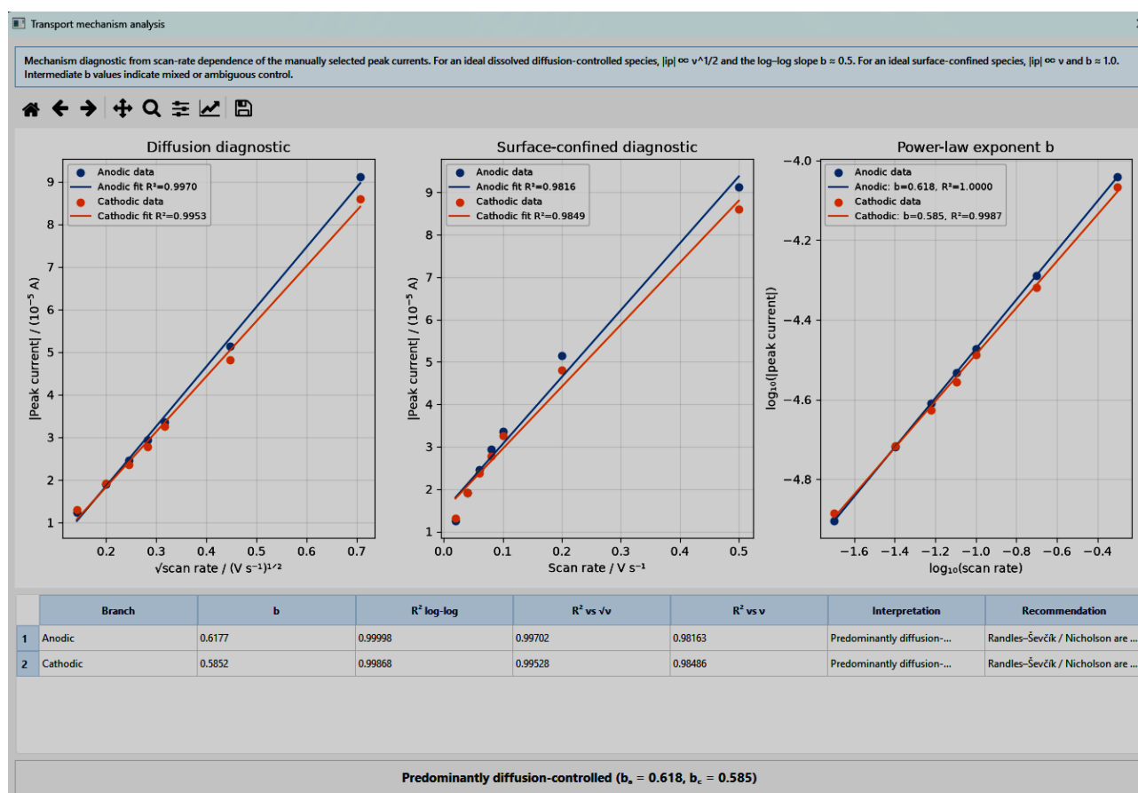
Figure 14: Transport-mechanism diagnostic based on the scan-rate dependence of the selected peak currents. Left: diffusion diagnostic, |i_p| versus \sqrt{\nu} . Centre: surface-confined diagnostic, |i_p| versus \nu . Right: log-log plot giving the power-law exponent b . A value of b \approx 0.5 indicates an ideal dissolved, diffusion-controlled species and b \approx 1.0 a surface-confined species; here b(\text{anodic}) = 0.62 and b(\text{cathodic}) = 0.59 , indicating predominantly diffusion-controlled behaviour.
