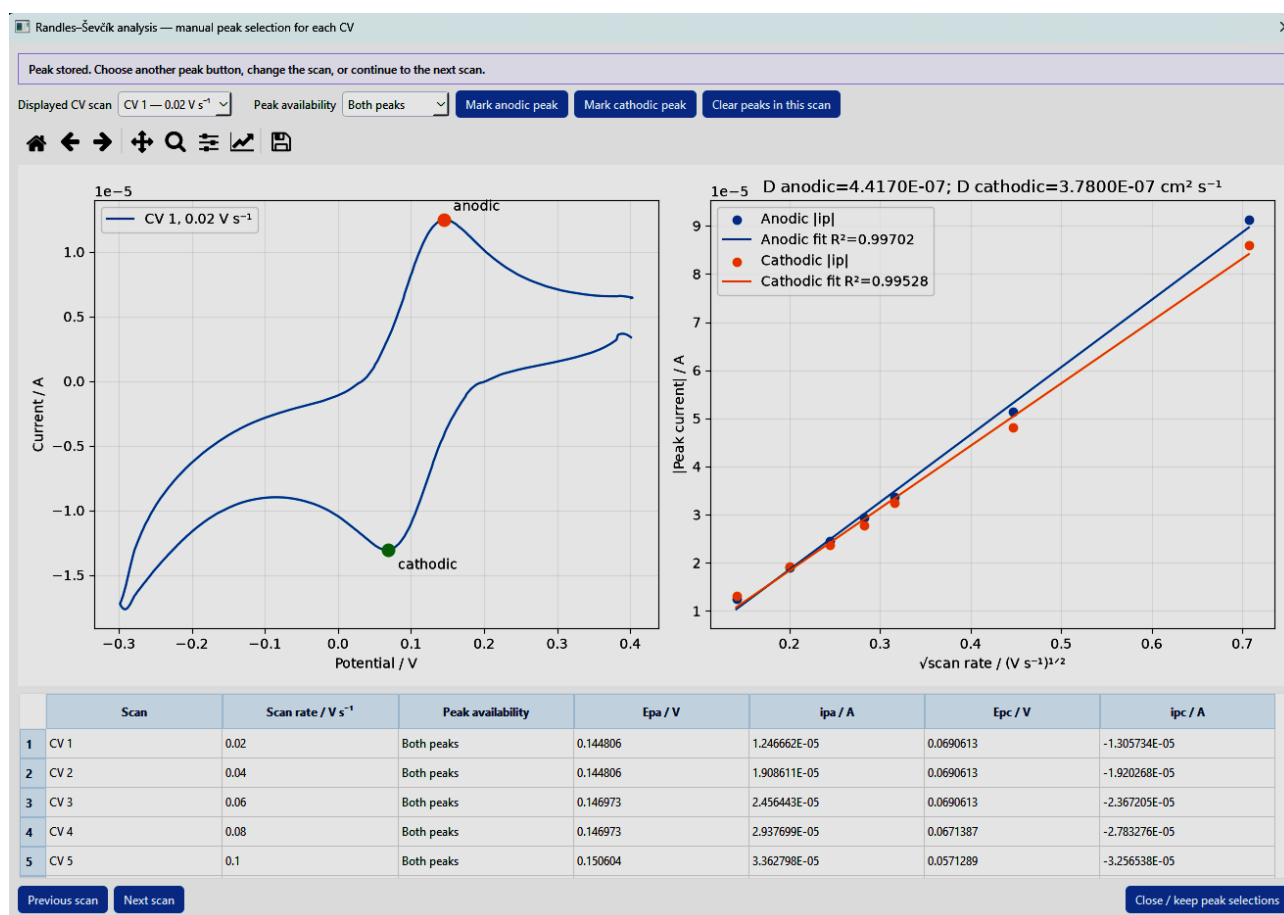
Figure 12: Randles–Ševčík analysis with manual peak selection. Left: a single cyclic voltammogram with the marked anodic (red) and cathodic (green) peaks. Right: the absolute peak current |i_p| versus the square root of the scan rate for both branches, with linear regressions yielding separate anodic and cathodic diffusion coefficients (here D(\text{anodic}) = 4.42 \times 10^{-7} \text{ cm}^2 \text{ s}^{-1} and D(\text{cathodic}) = 3.78 \times 10^{-7} \text{ cm}^2 \text{ s}^{-1} ). The table lists the peak potentials and currents for each scan.
