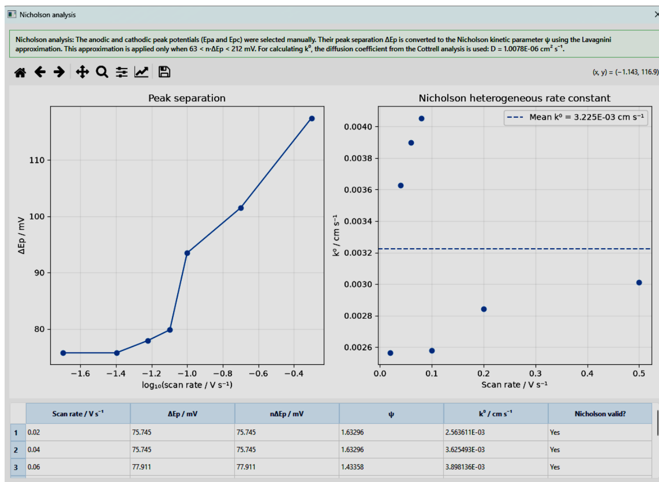
Figure 13: Nicholson analysis of the electron-transfer kinetics. Left: the anodic–cathodic peak separation \Delta E_p as a function of \log_{10}(\text{scan rate}) . Right: the heterogeneous rate constant k^0 derived from \Delta E_p , together with its mean value (here k^0 = 3.23 \times 10^{-3} cm s -1 ). The diffusion coefficient from the Cottrell analysis is used as input, and the approximation is applied only where 63 \text{ mV} < n\Delta E_p < 212 \text{ mV} .
