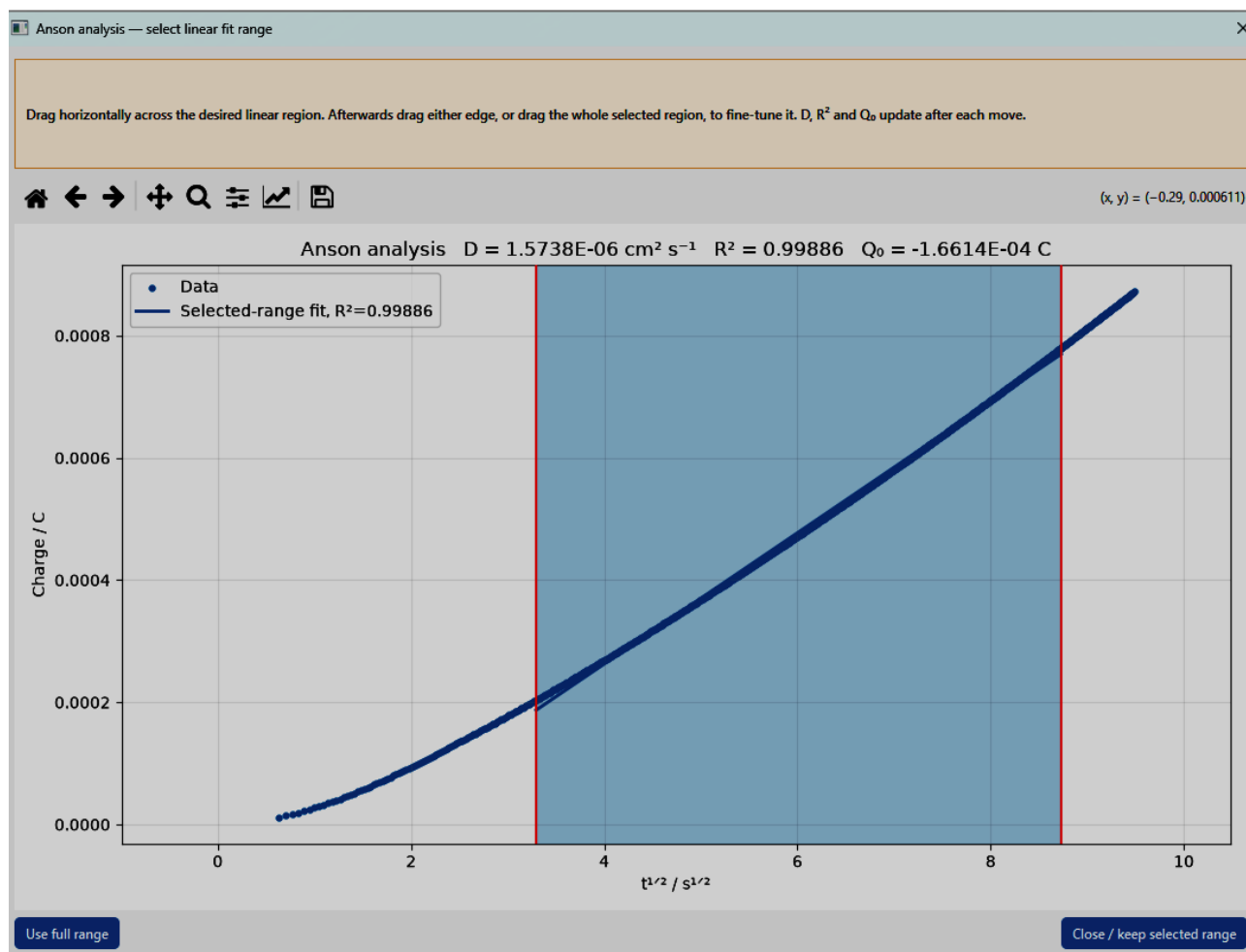
Figure 11: Anson analysis. The charge Q is plotted against t^{1/2} with the linear fit interval selected interactively (shaded band). The diffusion coefficient follows from the slope (here D = 1.57 \times 10^{-6} \text{ cm}^2 \text{ s}^{-1} , R^2 = 0.9989 ); the intercept Q_0 collects the double-layer charging and any adsorption contribution.
