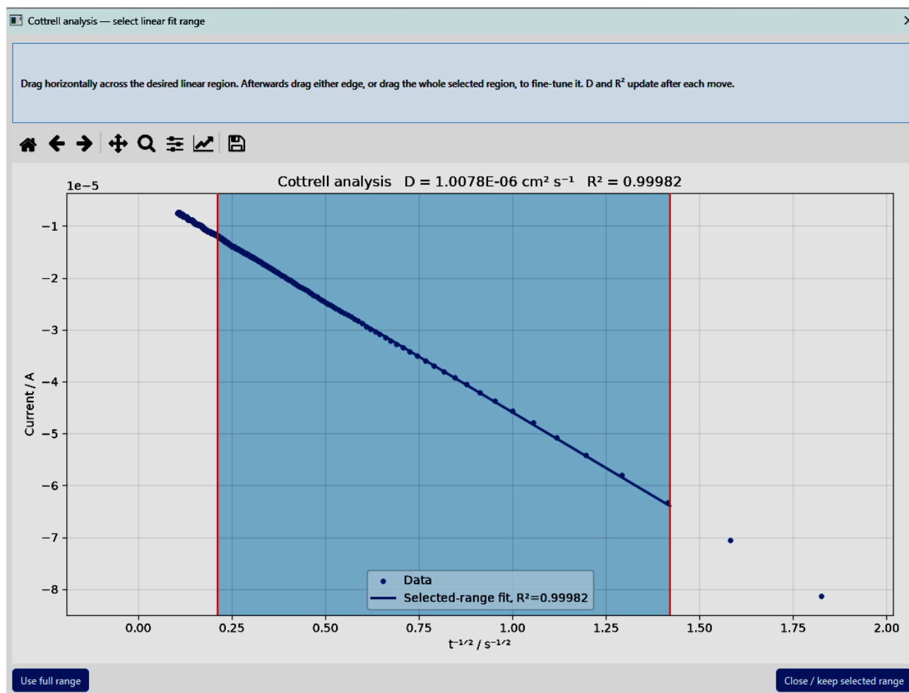
Figure 10: Cottrell analysis. The current I is plotted against t^{-1/2} , and the linear fit interval is selected interactively (shaded band). The diffusion coefficient is obtained from the slope (here D = 1.01 \times 10^{-6} \text{ cm}^2 \text{ s}^{-1} , R^2 = 0.9998 ). Points affected by double-layer charging at very short times fall outside the selected range.
