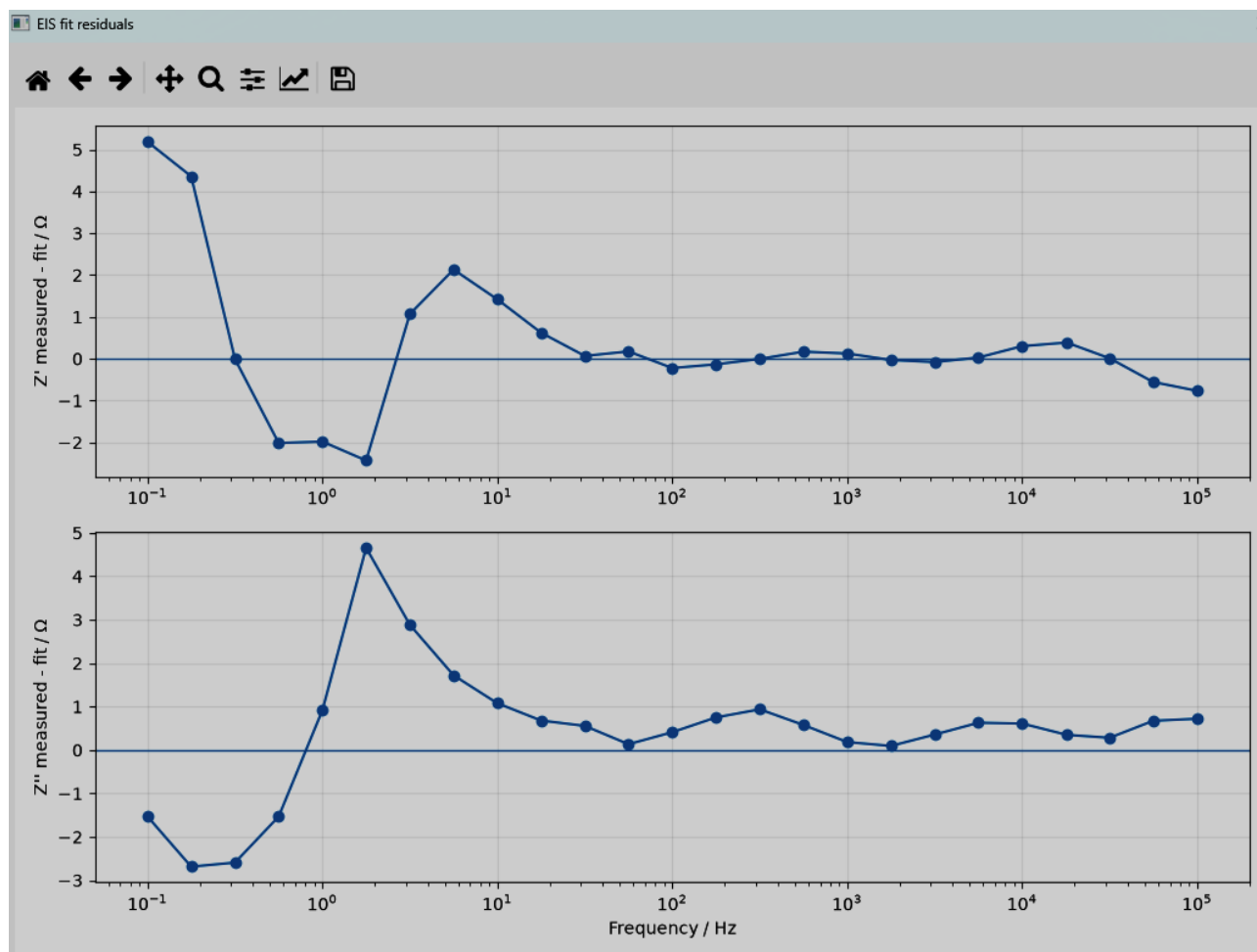
Figure 18: Residuals of the equivalent-circuit fit, shown as the difference between measured and fitted values for the real part Z' (top) and the imaginary part Z'' (bottom) as a function of frequency. Small, randomly distributed residuals support the selected model, whereas structured residuals indicate that the model, the weighting or the data quality should be reconsidered.
