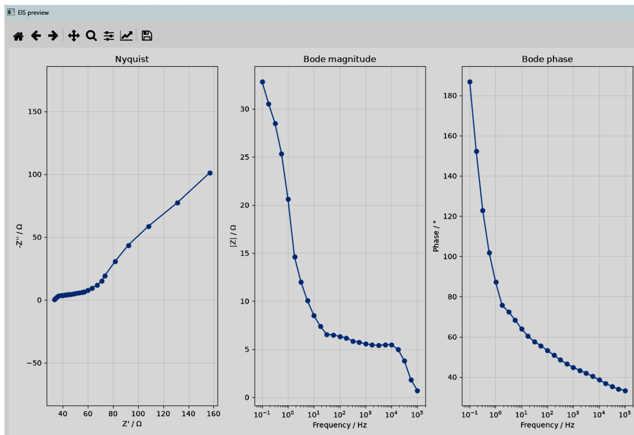
Figure 16: Preview of the imported impedance data before fitting, shown as a Nyquist plot ( -Z'' versus Z' ) together with the Bode magnitude |Z| and the Bode phase \phi as functions of frequency. Previewing the raw data makes it possible to identify outliers and incomplete frequency regions before an equivalent circuit is applied.
