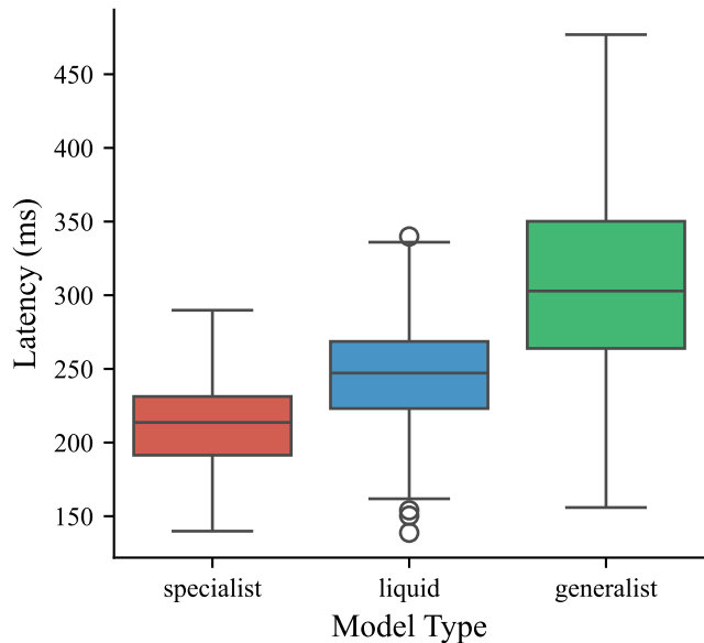
(b) Latency by Model Type
