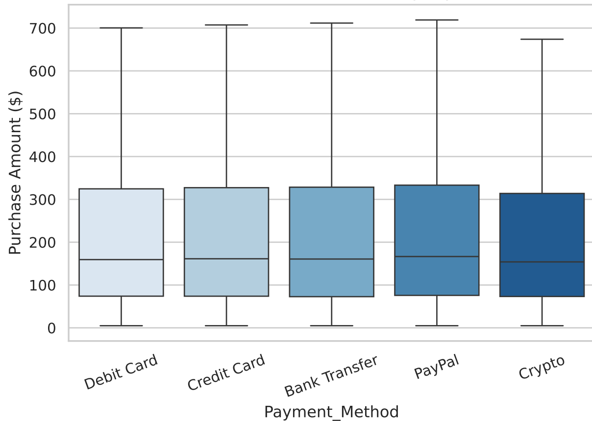
RQ3 — Purchase Amount Distribution by Payment Method
