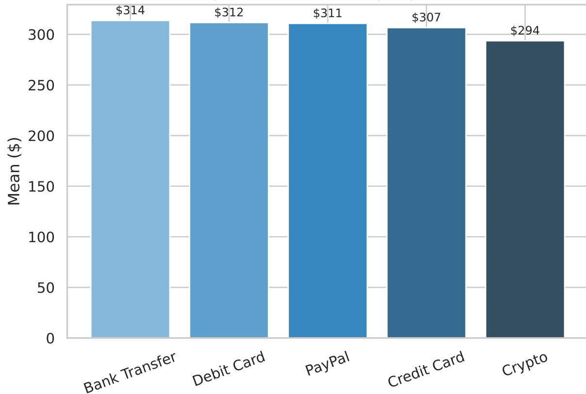
RQ3 — Avg Purchase Amount by Payment Method
