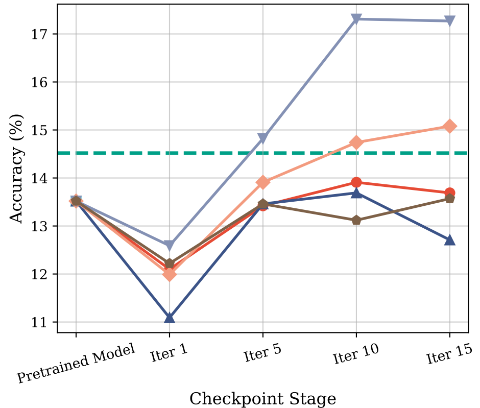
Evaluation on SUPERGPQA
