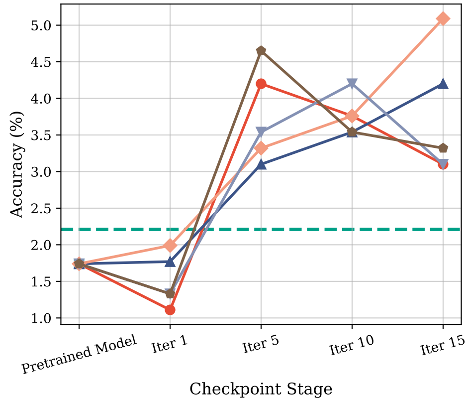
Evaluation on BBEH
