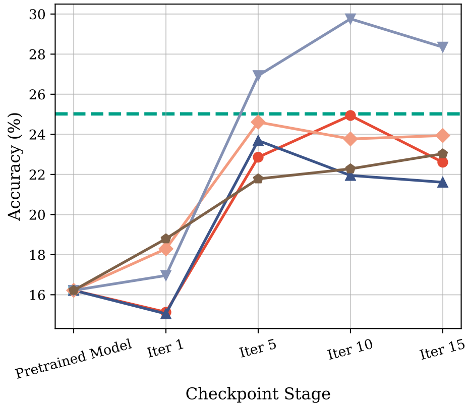
Evaluation on MMLUPRO
