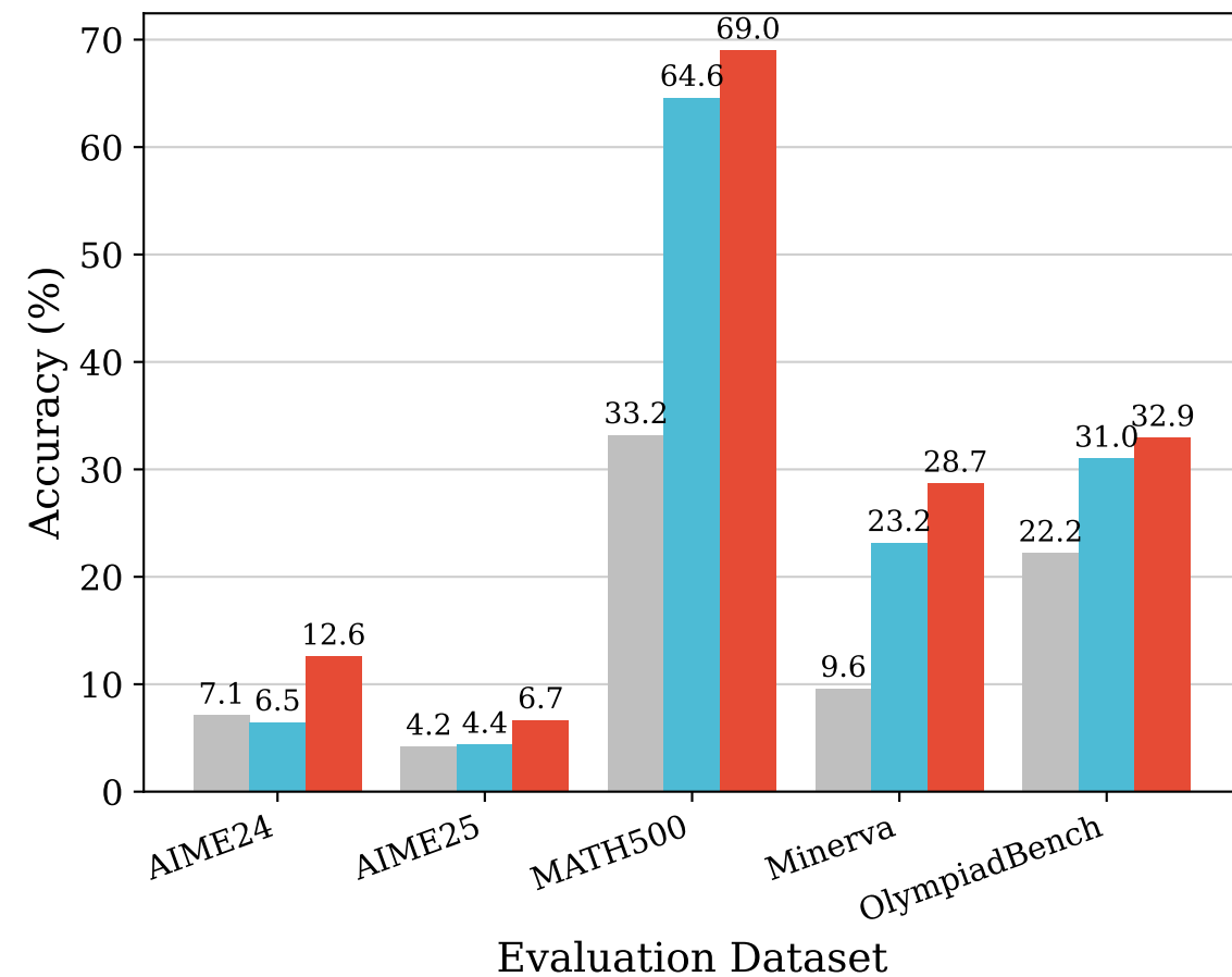
Trained on AMC23
