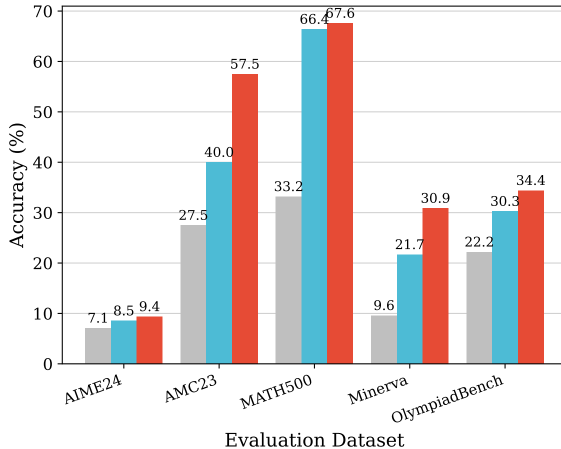
Trained on AIME25
