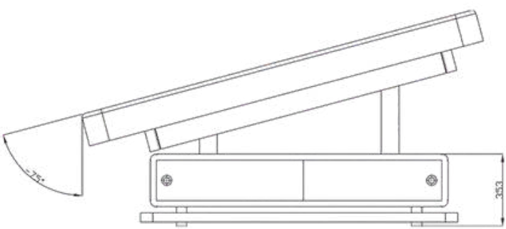
TRENDELENBURG (HEAD SIDE DOWN)
