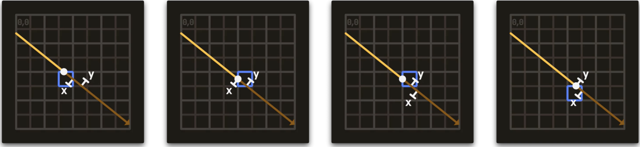
Figure 4: DDA algorithm stepping through voxels. Each step advances the axis with the smallest t_{\max} .
