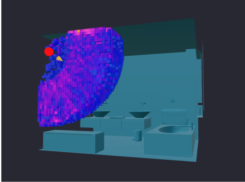
Figure 6: Voxels Heatmap
