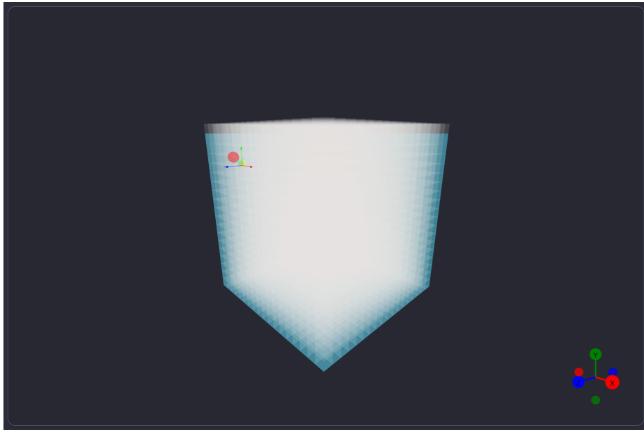
Figure 5: Scene Example
