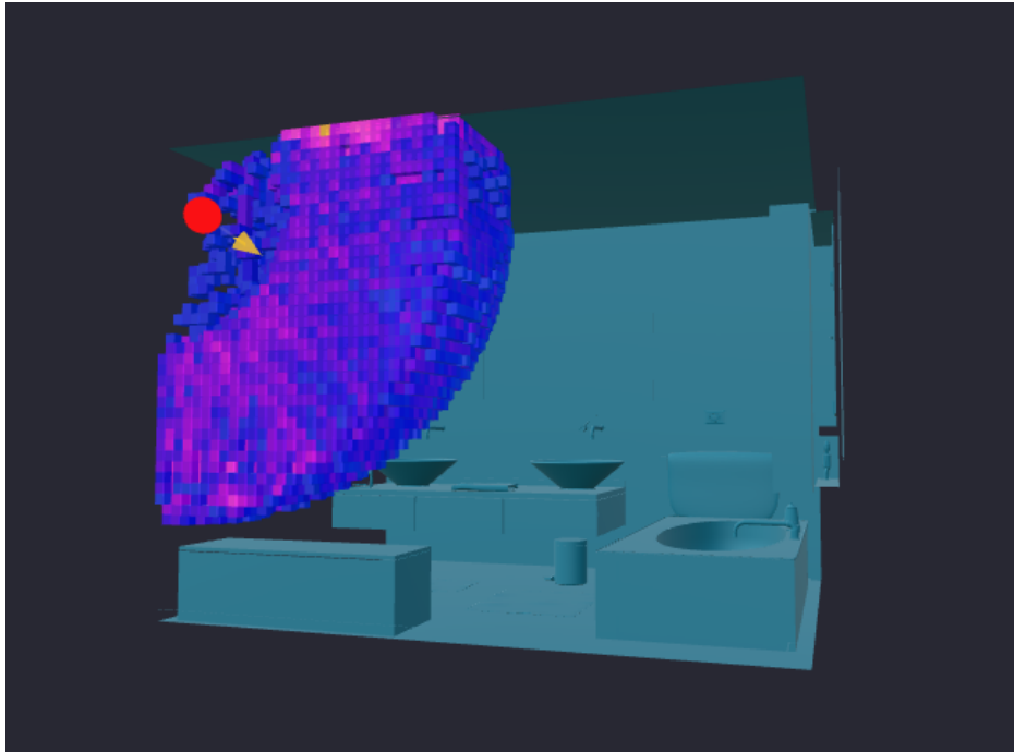
Figure 6: Voxels Heatmap
