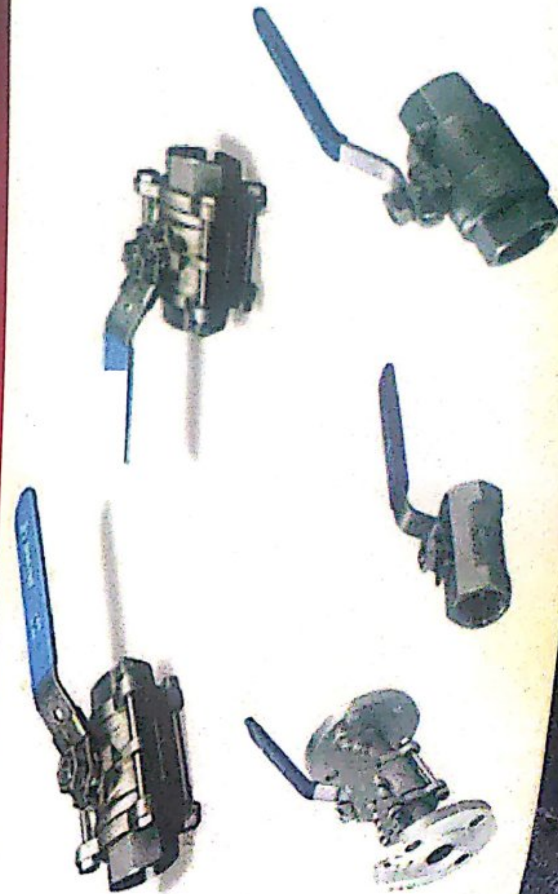
SS BALL VALVES 316 THREADED AND FLANGE TYPE, 1/2" - 4" Threaded and Flap
