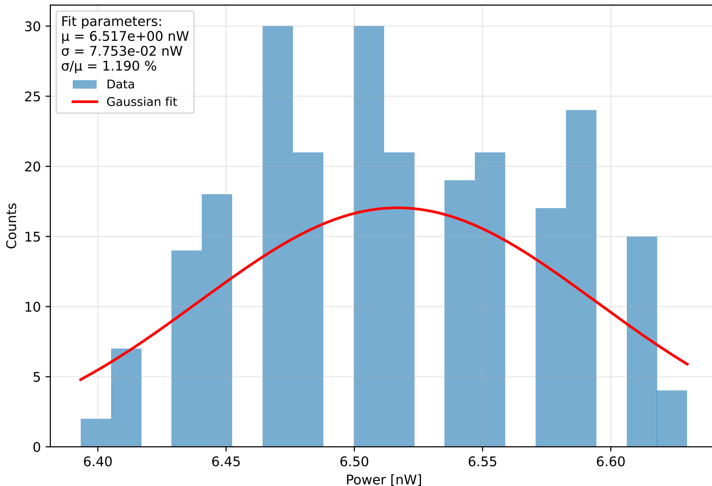
Histogram of power Run 5 (meas. 17) - \lambda=401.0 nm, pulse width=780 ps, PD current = 7.489 pA Start: 2025-11-28 11:29:31, \Delta t=0.1 s, N=243, T=24.2 s
