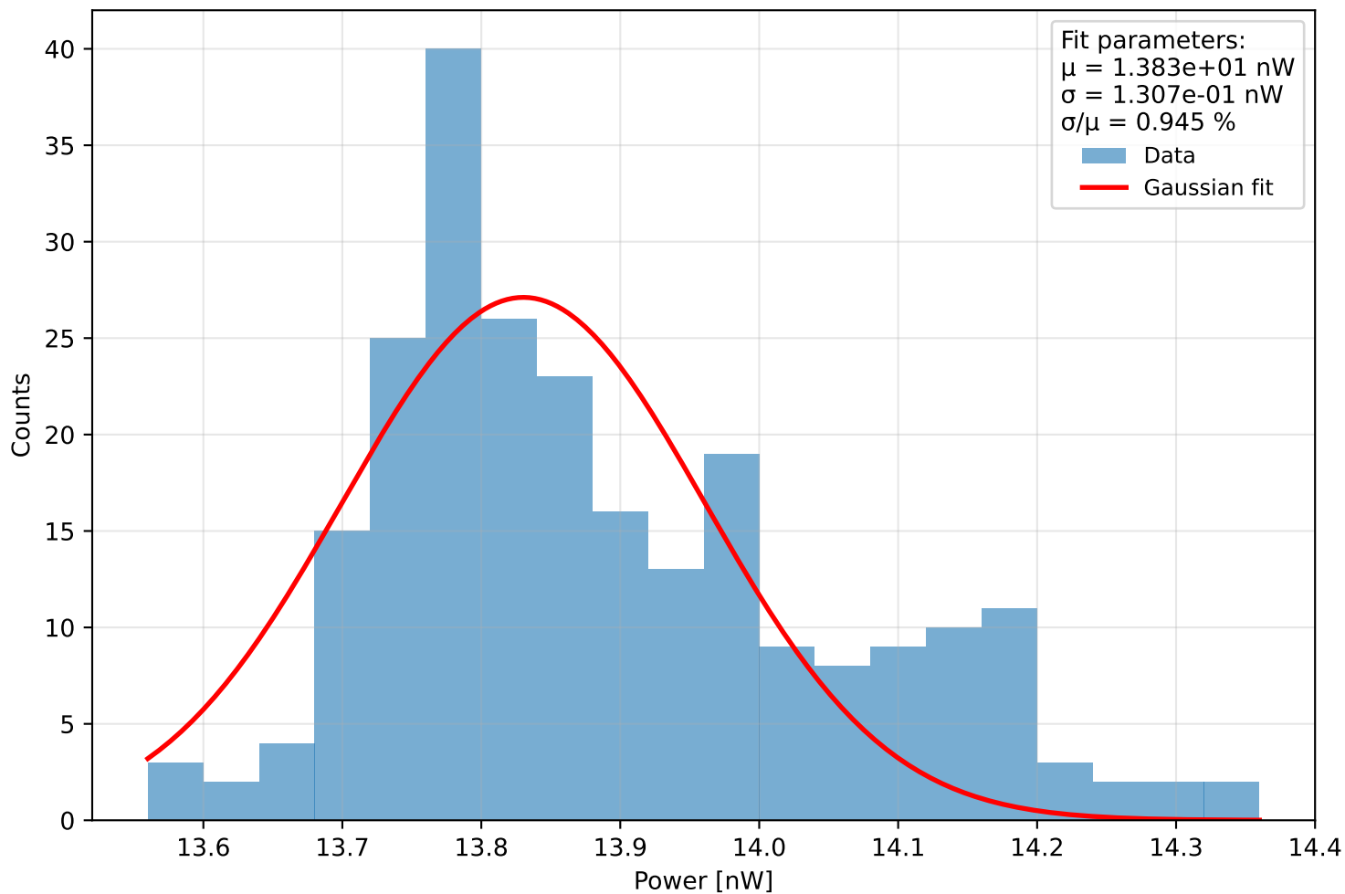
Histogram of power Run 2 (meas. 14) - \lambda=401.0 nm, pulse width=810 ps, PD current = 7.591 pA Start: 2025-11-27 18:03:05, \Delta t=0.1 s, N=242, T=24.1 s
