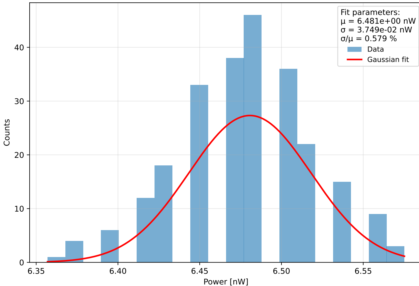
Histogram of power Run 4 (meas. 17) - \lambda=401.0 nm, pulse width=780 ps, PD current = 7.489 pA Start: 2025-11-28 11:28:53, \Delta t=0.1 s, N=243, T=24.2 s
