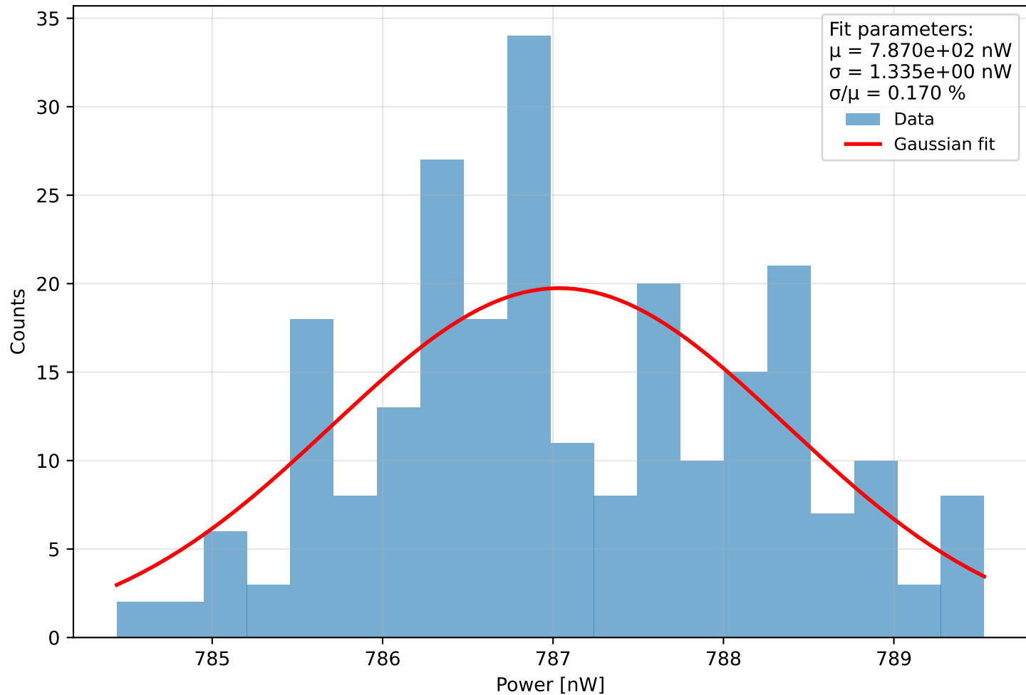
Histogram of power Run 0 (meas. 10) - \lambda=401.0 nm, pulse width=850 ps, PD current = 8.63 pA Start: 2025-11-27 17:43:12, \Delta t=0.1 s, N=244, T=24.3 s
