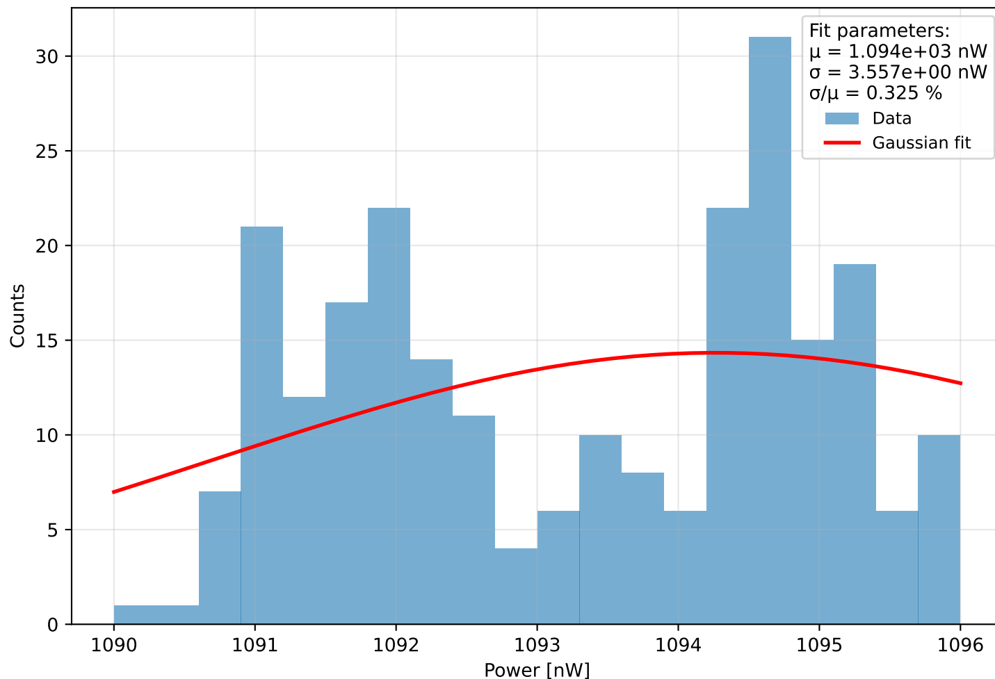
Histogram of power Run 2 (meas. 8) - \lambda=401.0 nm, pulse width=870 ps, PD current = 8.926 pA Start: 2025-11-27 17:33:55, \Delta t=0.1 s, N=243, T=24.2 s
