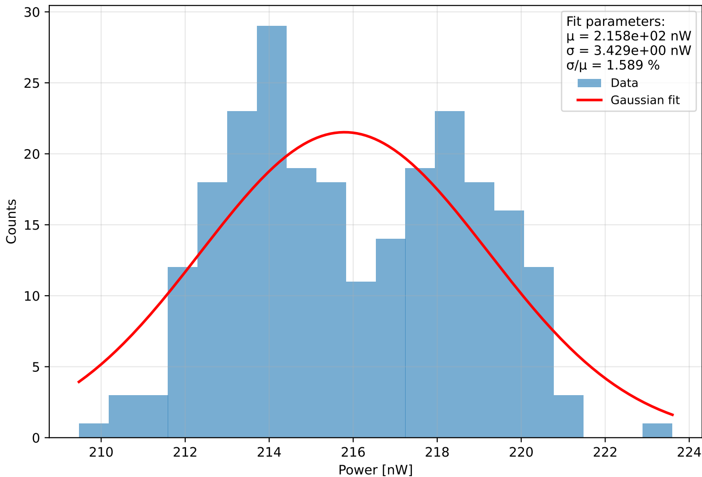
Histogram of power Run 0 (meas. 13) - \lambda=401.0 nm, pulse width=820 ps, PD current = 7.958 pA Start: 2025-11-27 17:54:15, \Delta t=0.1 s, N=243, T=24.2 s
