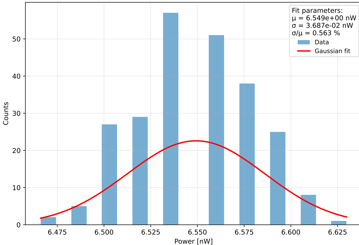
Histogram of power Run 0 (meas. 17) - \lambda=401.0 nm, pulse width=780 ps, PD current = 7.489 pA Start: 2025-11-28 11:23:12, \Delta t=0.1 s, N=243, T=24.2 s
