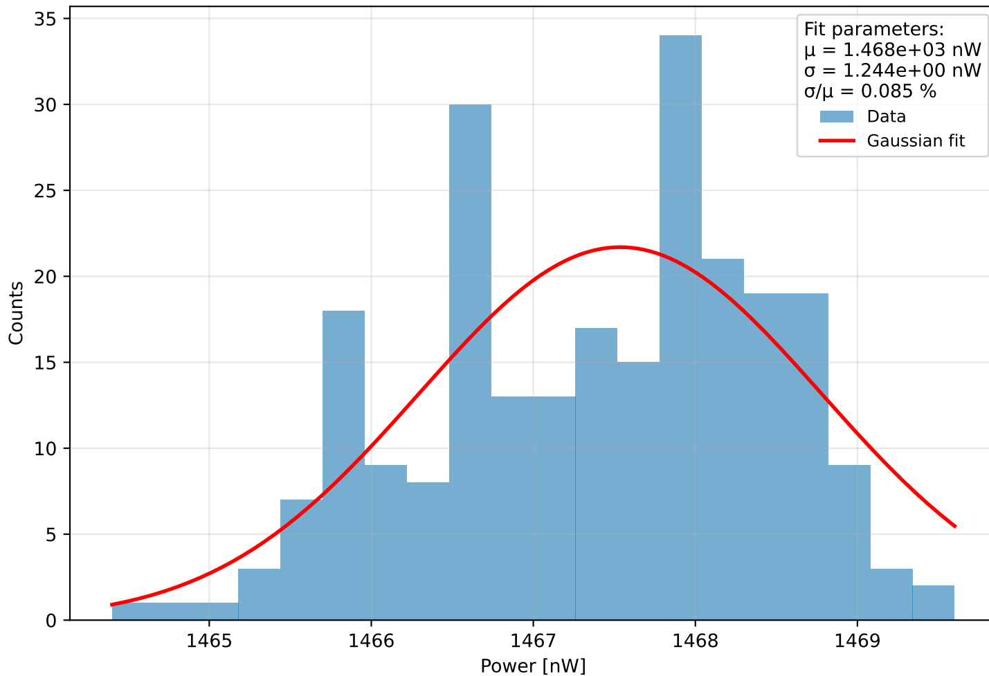
Histogram of power Run 0 (meas. 39) - \lambda=392.0 nm, pulse width=900 ps, PD current = 9.171 pA Start: 2025-11-28 14:40:10, \Delta t=0.1 s, N=243, T=24.2 s
