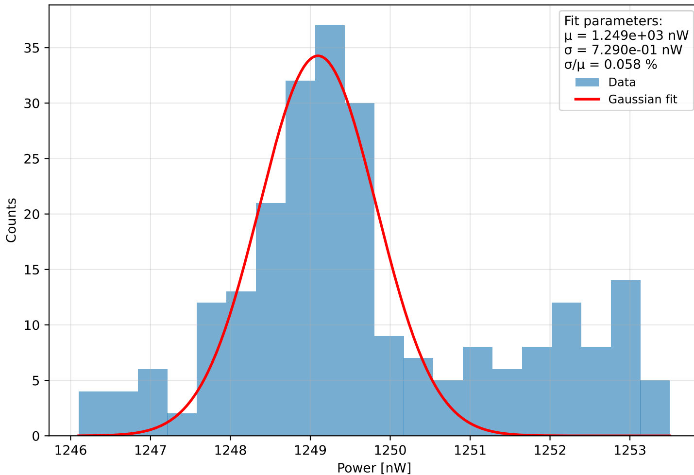
Histogram of power Run 0 (meas. 22) - \lambda=401.0 nm, pulse width=900 ps, PD current = 9.171 pA Start: 2025-11-28 14:07:00, \Delta t=0.1 s, N=243, T=24.2 s
