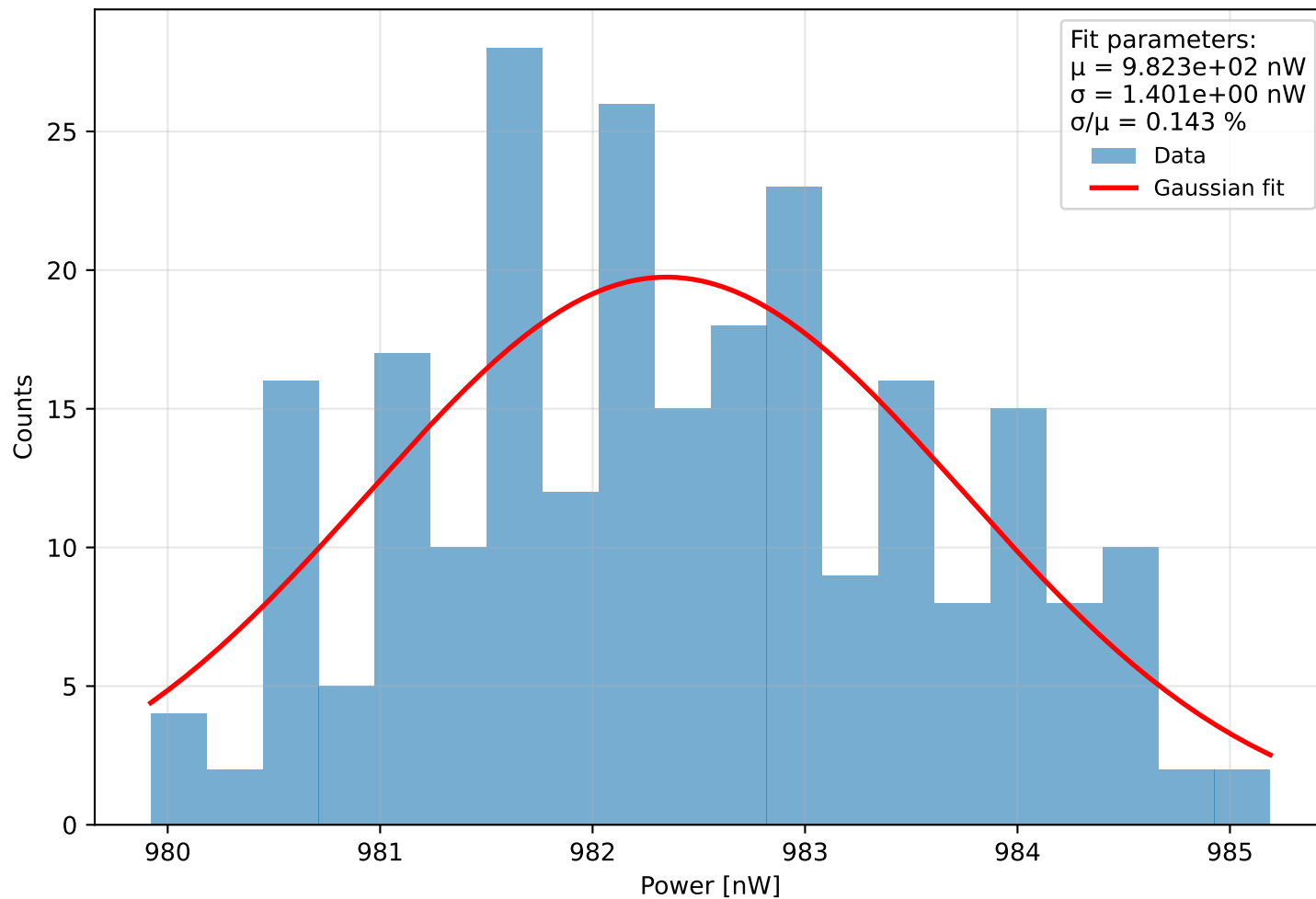
Histogram of power Run 0 (meas. 9) - \lambda=401.0 nm, pulse width=860 ps, PD current = 8.806 pA Start: 2025-11-27 17:39:55, \Delta t=0.1 s, N=246, T=24.5 s
