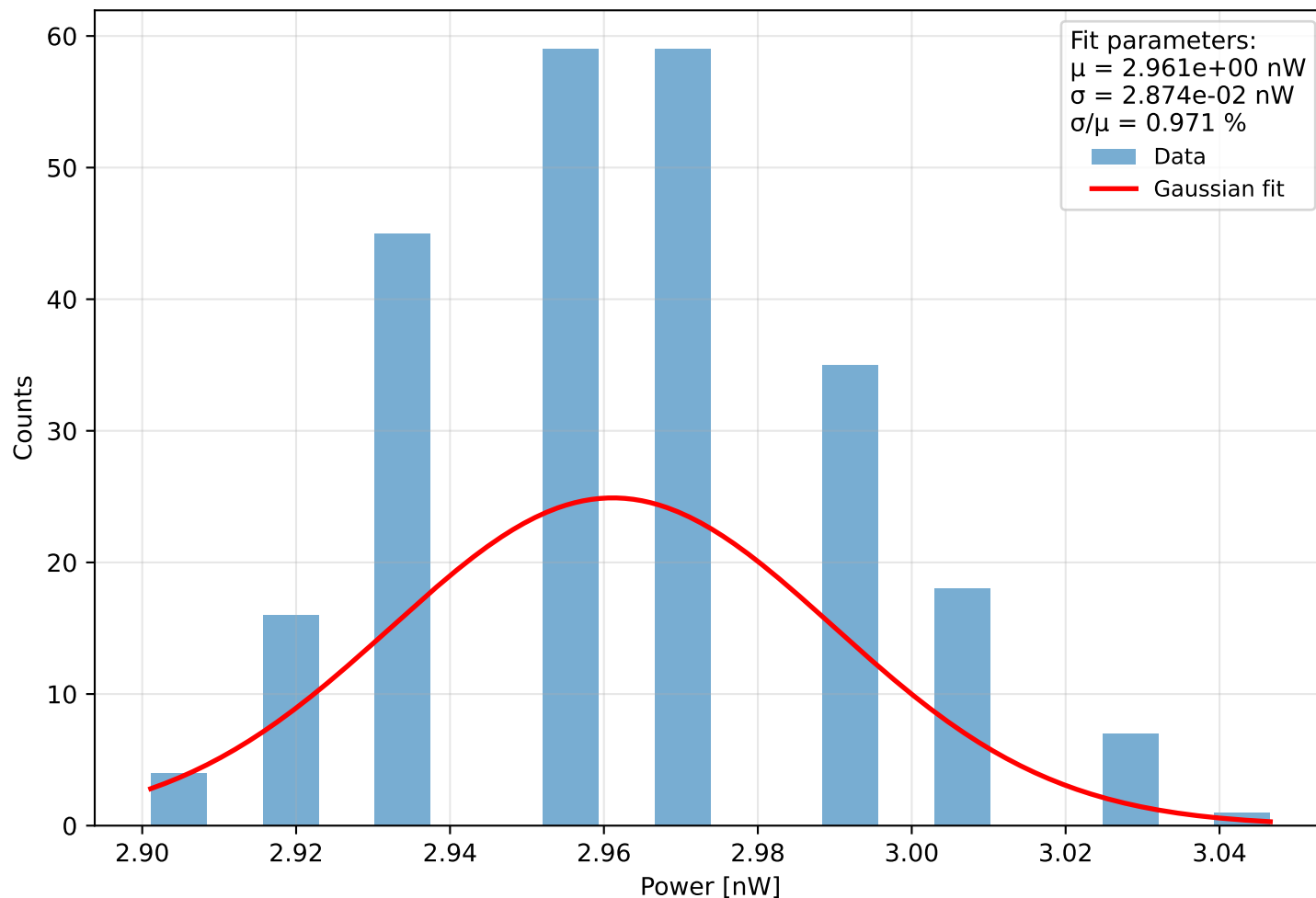
Histogram of power Run 0 (meas. 19) - \lambda=401.0 nm, pulse width=760 ps, PD current = 7.29 pA Start: 2025-11-28 11:43:41, \Delta t=0.1 s, N=244, T=24.3 s
