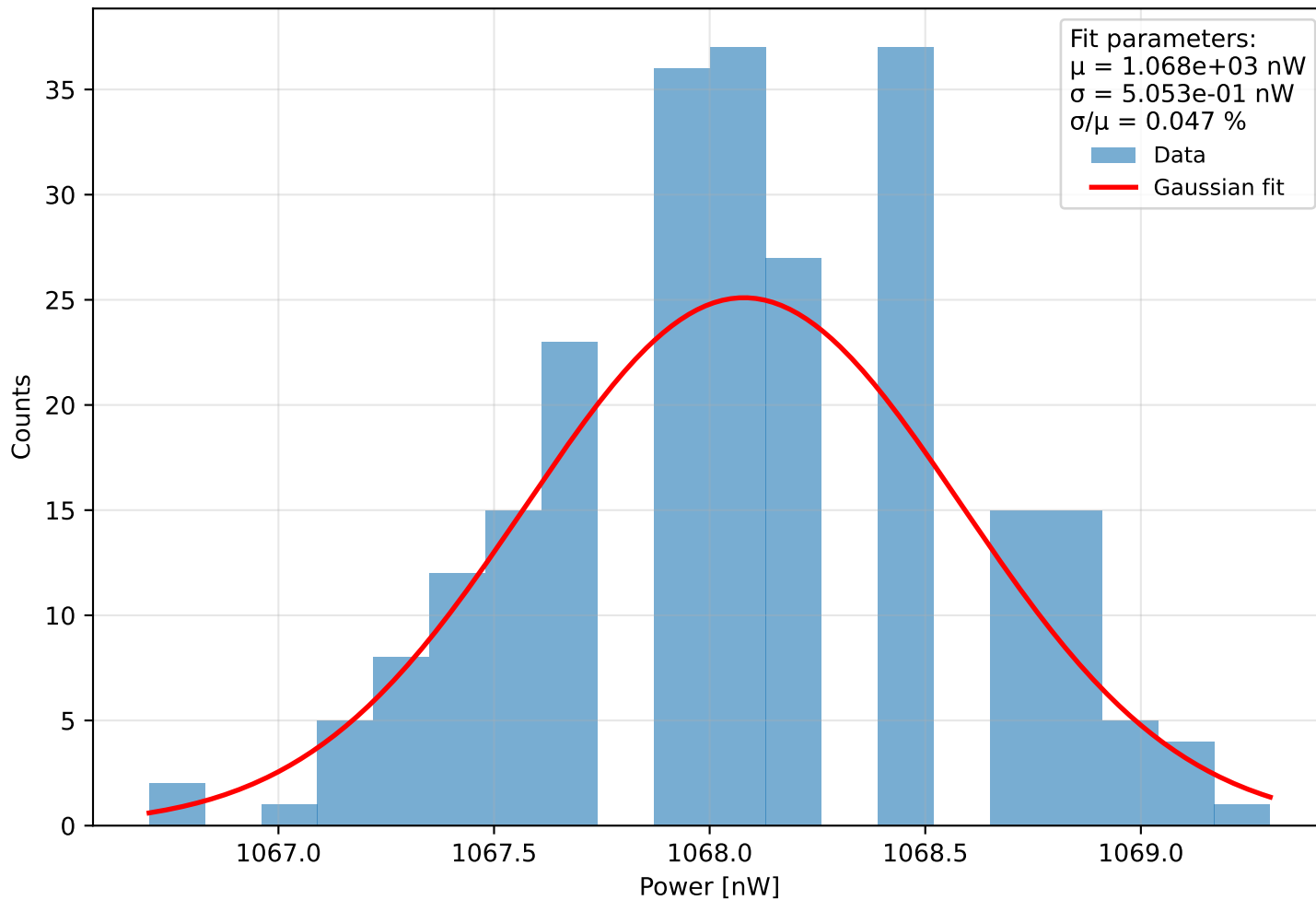
Histogram of power Run 0 (meas. 34) - \lambda=413.0 nm, pulse width=900 ps, PD current = 9.171 pA Start: 2025-11-28 14:32:36, \Delta t=0.1 s, N=243, T=24.2 s
