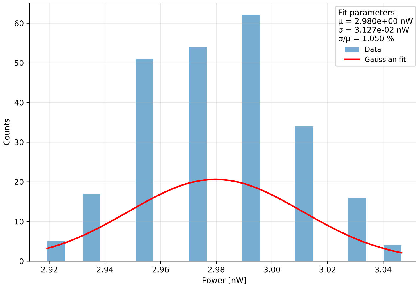
Histogram of power Run 1 (meas. 19) - \lambda=401.0 nm, pulse width=760 ps, PD current = 7.29 pA Start: 2025-11-28 11:47:19, \Delta t=0.1 s, N=243, T=24.2 s
