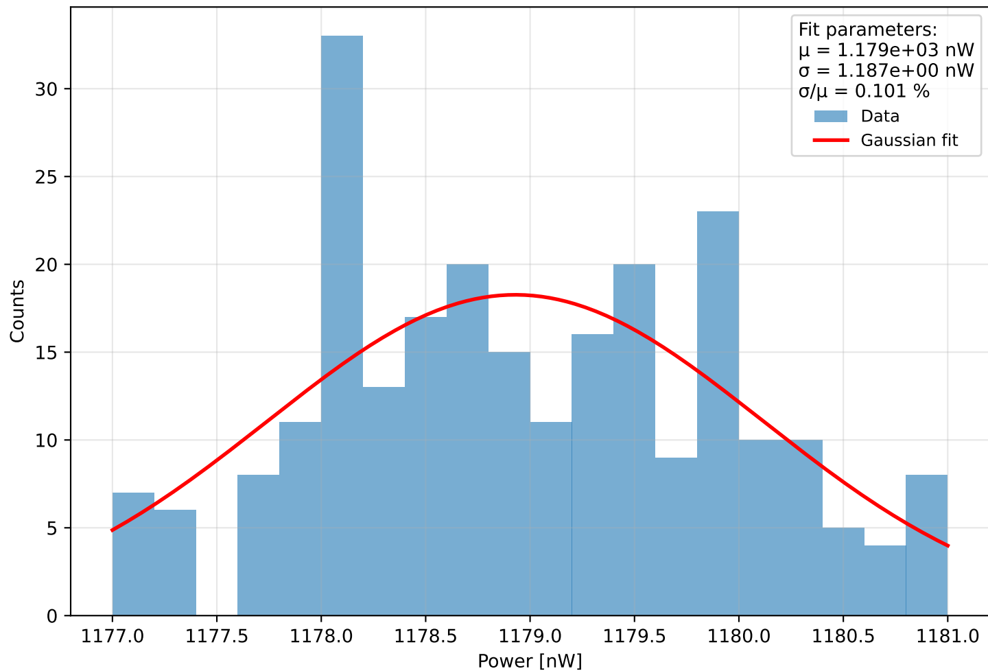
Histogram of power Run 2 (meas. 6) - \lambda=401.0 nm, pulse width=890 ps, PD current = 9.048 pA Start: 2025-11-27 17:28:18, \Delta t=0.1 s, N=246, T=24.5 s
