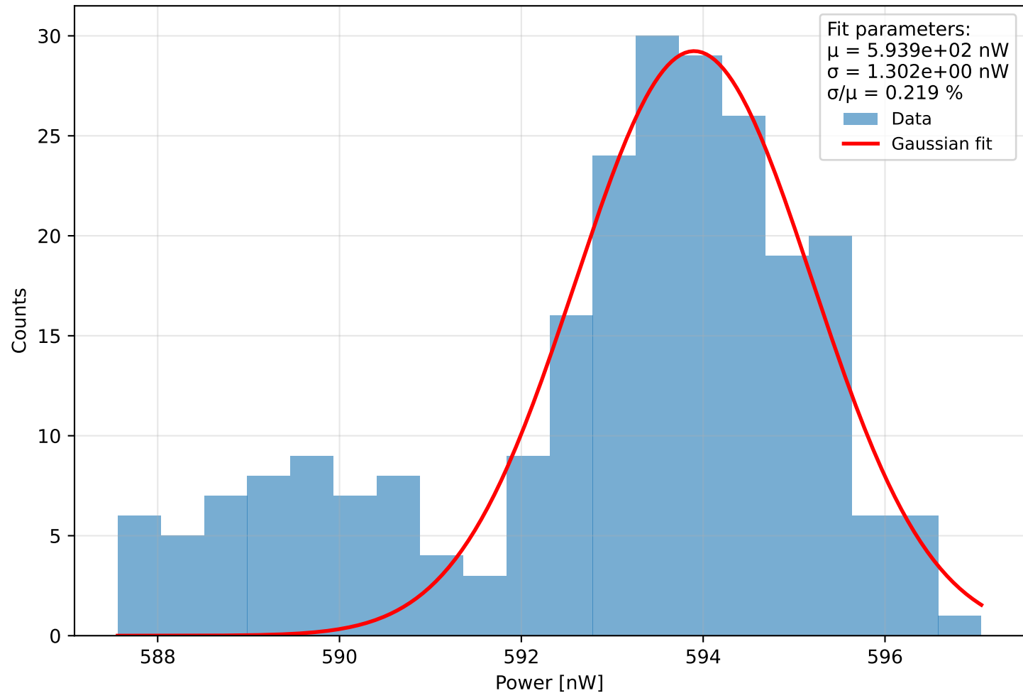
Histogram of power Run 0 (meas. 11) - \lambda=401.0 nm, pulse width=840 ps, PD current = 8.4 pA Start: 2025-11-27 17:46:29, \Delta t=0.1 s, N=243, T=24.2 s
