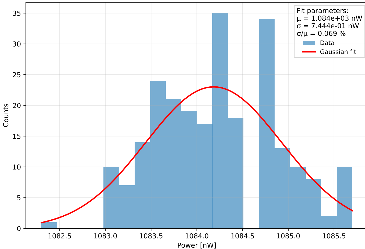
Histogram of power Run 0 (meas. 33) - \lambda=412.0 nm, pulse width=900 ps, PD current = 9.171 pA Start: 2025-11-28 14:29:07, \Delta t=0.1 s, N=243, T=24.2 s
