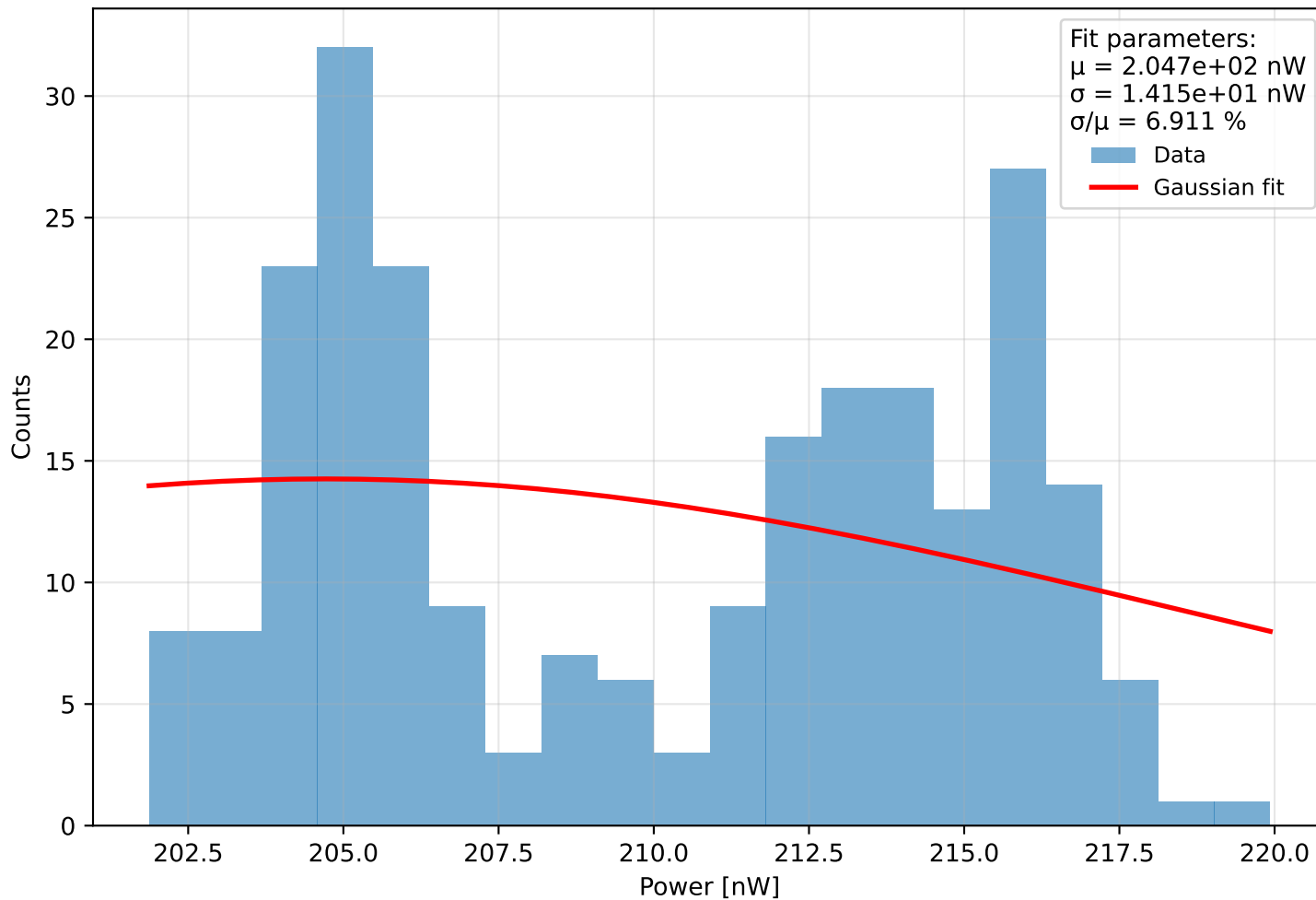
Histogram of power Run 2 (meas. 13) - \lambda=401.0 nm, pulse width=820 ps, PD current = 7.958 pA Start: 2025-11-27 17:56:35, \Delta t=0.1 s, N=245, T=24.4 s
