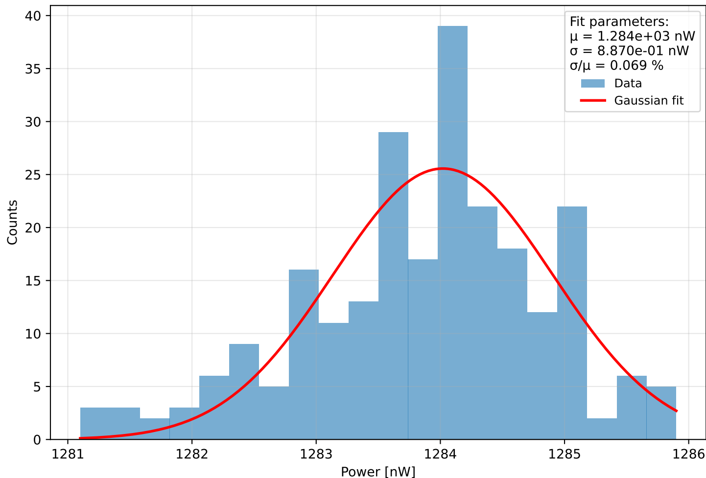
Histogram of power Run 2 (meas. 21) - \lambda=401.0 nm, pulse width=900 ps, PD current = 9.171 pA Start: 2025-11-28 12:01:06, \Delta t=0.1 s, N=243, T=24.2 s
