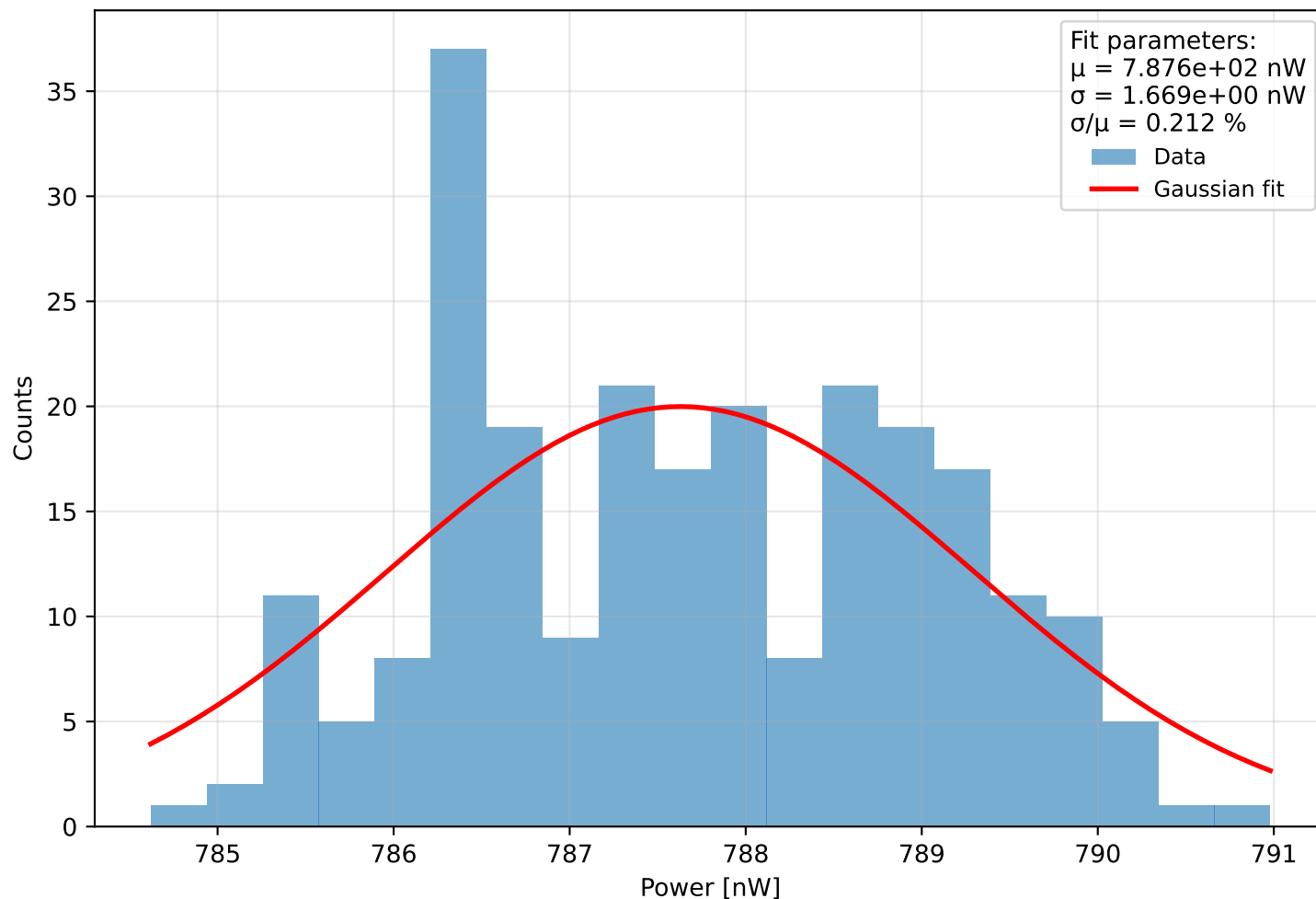
Histogram of power Run 2 (meas. 10) - \lambda=401.0 nm, pulse width=850 ps, PD current = 8.63 pA Start: 2025-11-27 17:45:06, \Delta t=0.1 s, N=243, T=24.2 s
