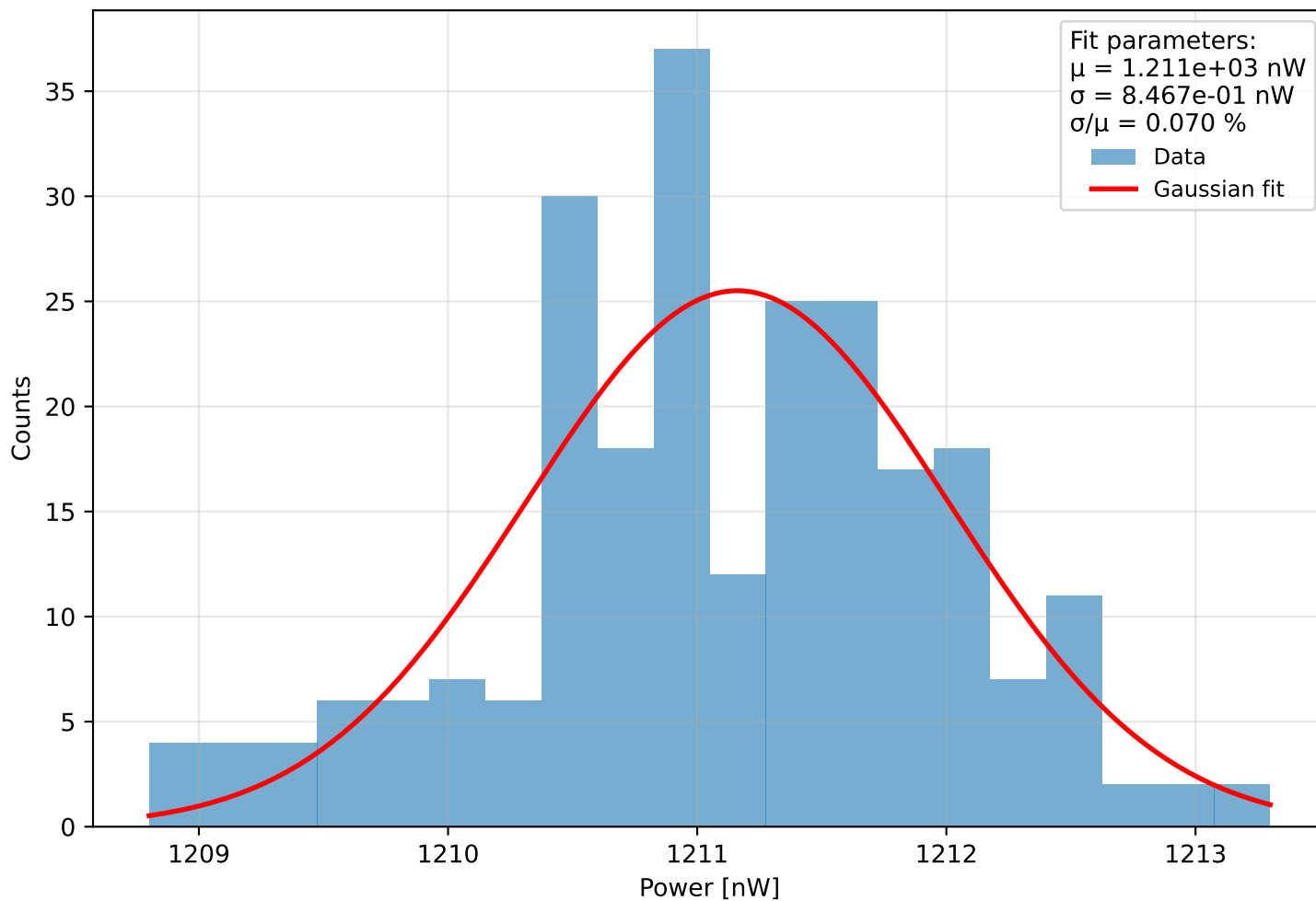
Histogram of power Run 0 (meas. 25) - \lambda=404.0 nm, pulse width=900 ps, PD current = 9.171 pA Start: 2025-11-28 14:11:06, \Delta t=0.1 s, N=243, T=24.2 s
