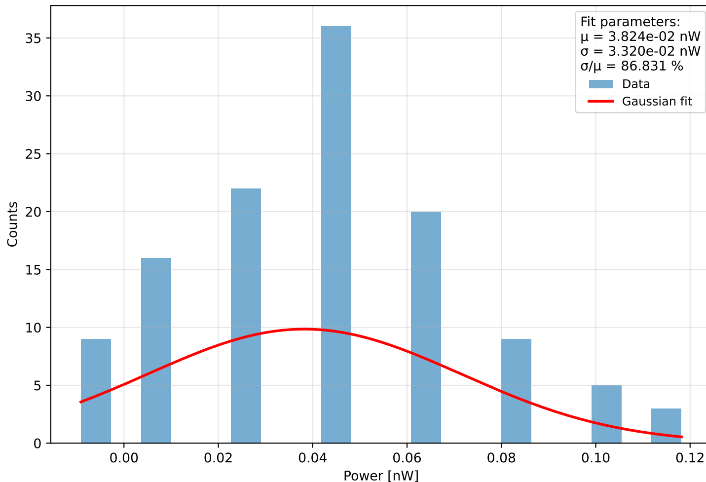
Histogram of power Run 0 (meas. 1) - \lambda=401.0 nm, pulse width=900 ps, PD current = 9.171 pA Start: 2025-11-27 16:03:19, \Delta t=0.5 s, N=120, T=59.5 s
