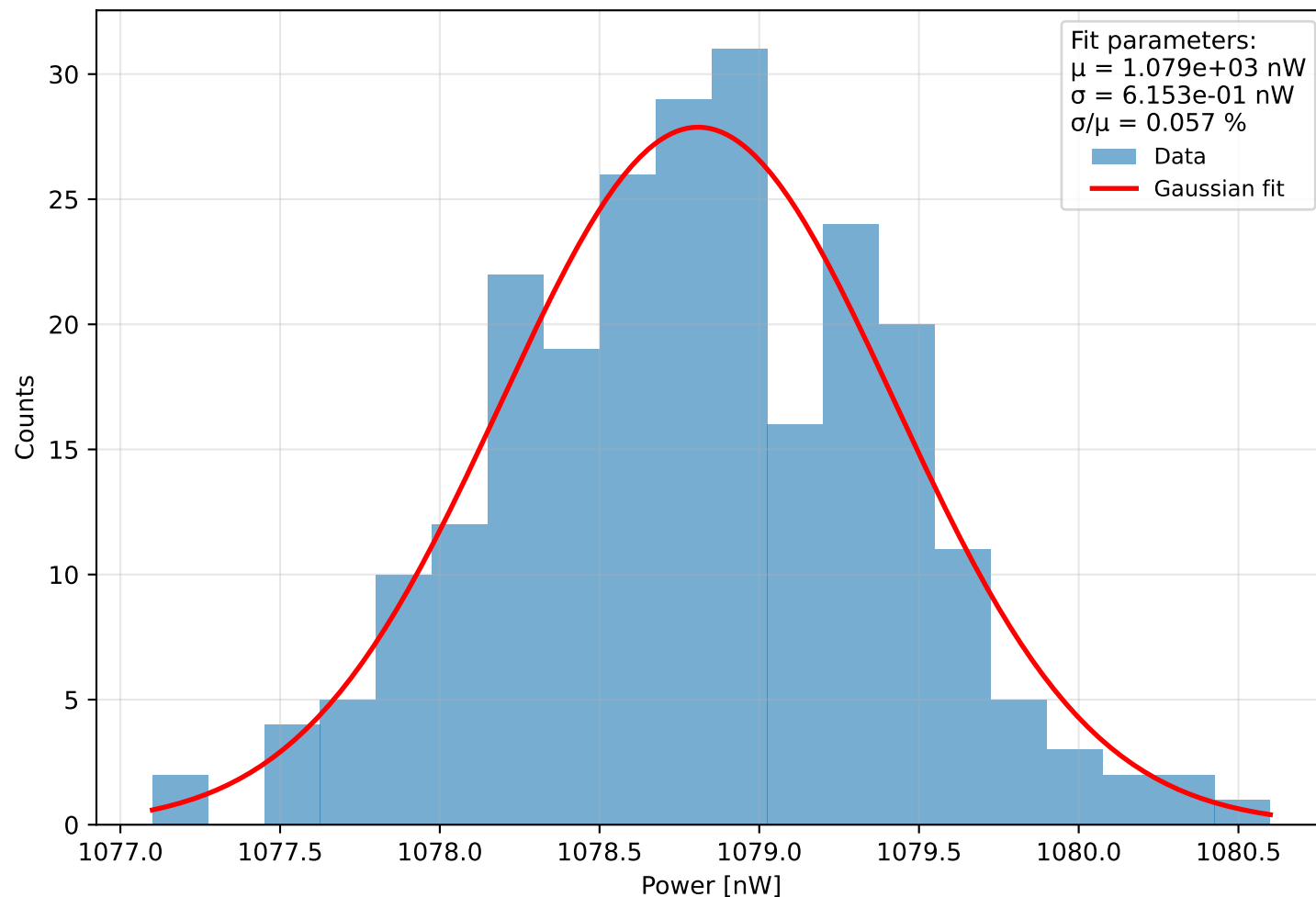
Histogram of power Run 2 (meas. 7) - \lambda=401.0 nm, pulse width=880 ps, PD current = 8.926 pA Start: 2025-11-27 17:31:51, \Delta t=0.1 s, N=244, T=24.3 s
