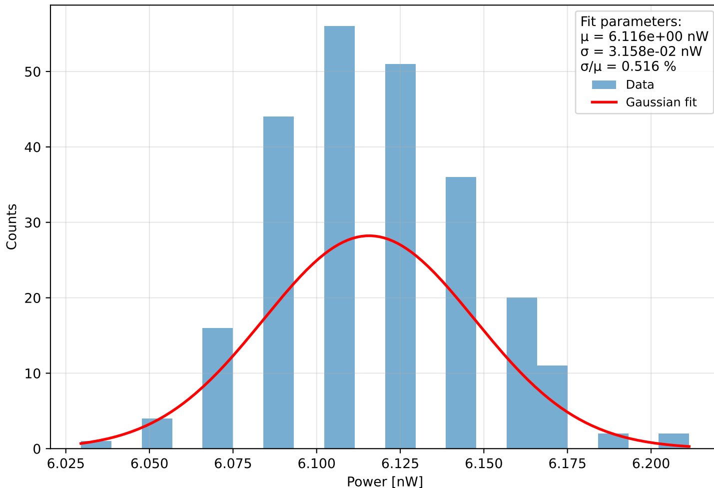
Histogram of power Run 1 (meas. 15) - \lambda=401.0 nm, pulse width=800 ps, PD current = 7.489 pA Start: 2025-11-28 11:02:49, \Delta t=0.1 s, N=243, T=24.2 s
