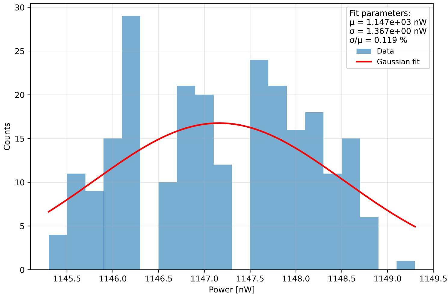
Histogram of power Run 0 (meas. 29) - \lambda=408.0 nm, pulse width=900 ps, PD current = 9.171 pA Start: 2025-11-28 14:22:38, \Delta t=0.1 s, N=243, T=24.2 s
