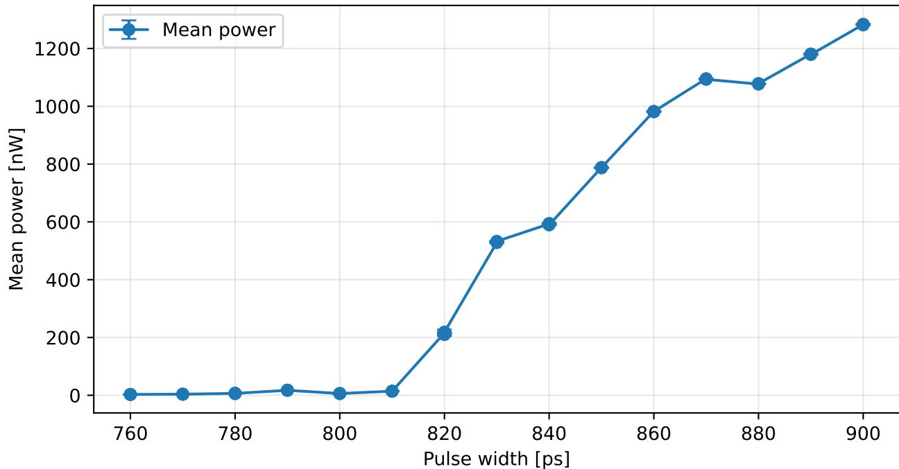
Mean power vs pulse width
