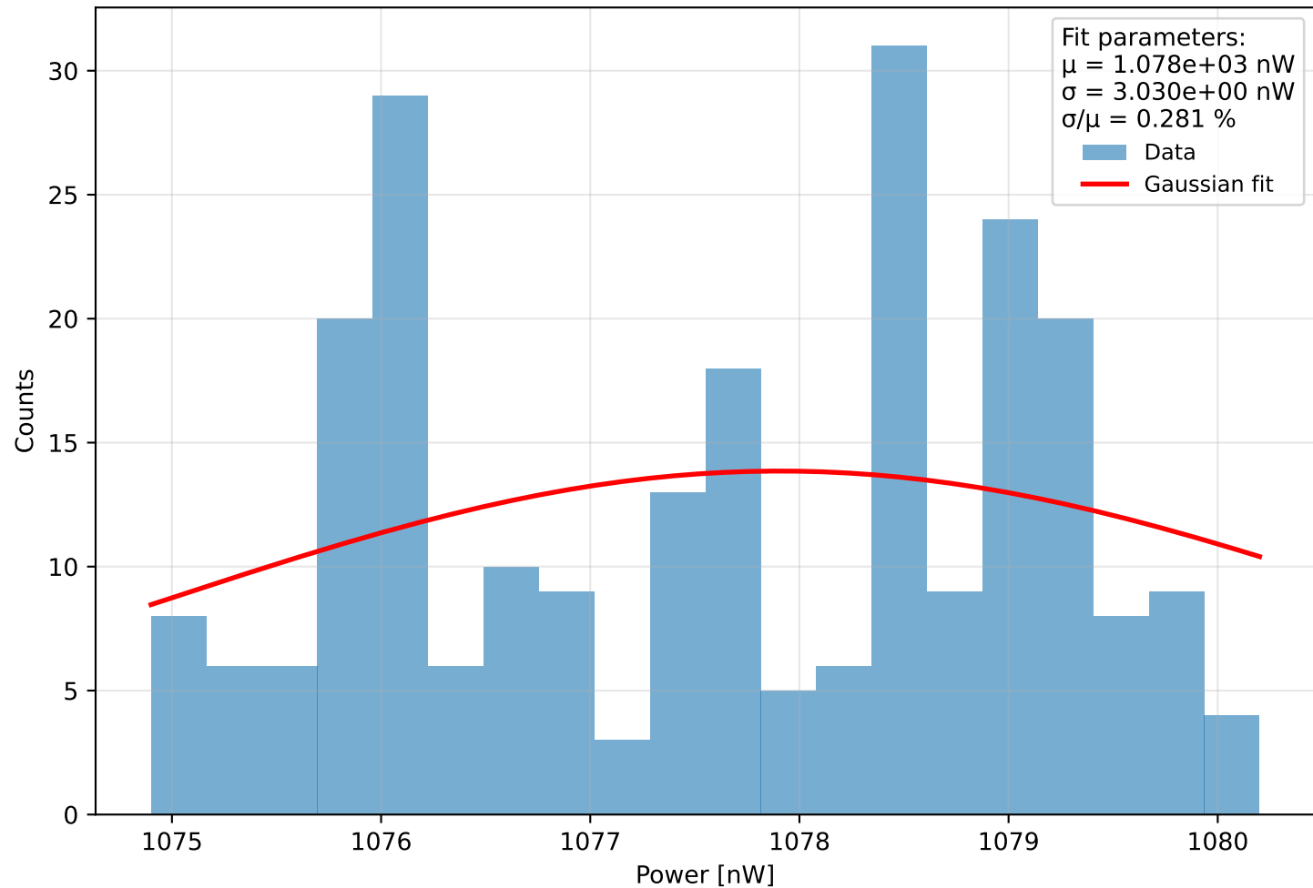
Histogram of power Run 1 (meas. 7) - \lambda=401.0 nm, pulse width=880 ps, PD current = 8.926 pA Start: 2025-11-27 17:31:15, \Delta t=0.1 s, N=244, T=24.3 s
