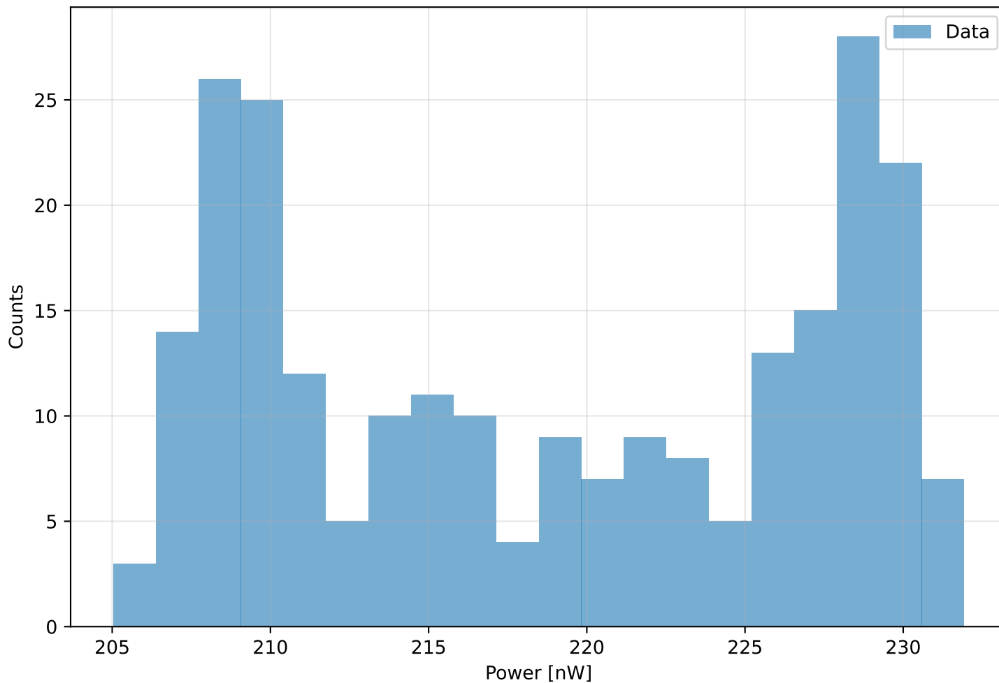
Histogram of power Run 1 (meas. 13) - \lambda=401.0 nm, pulse width=820 ps, PD current = 7.958 pA Start: 2025-11-27 17:55:42, \Delta t=0.1 s, N=243, T=24.2 s
