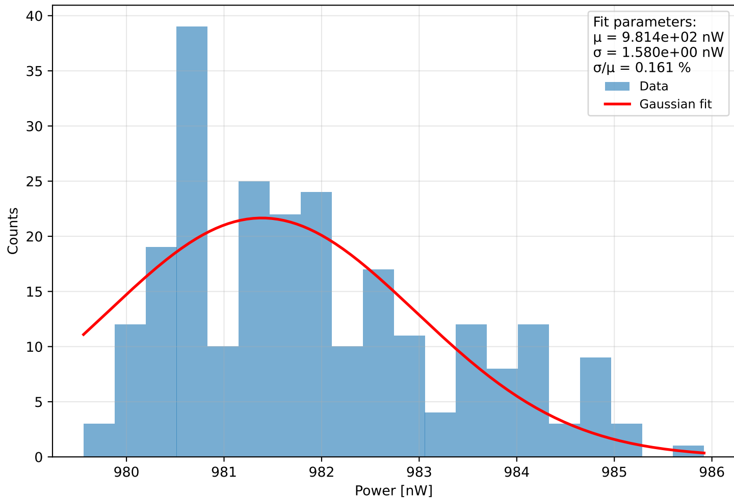
Histogram of power Run 1 (meas. 9) - \lambda=401.0 nm, pulse width=860 ps, PD current = 8.806 pA Start: 2025-11-27 17:41:07, \Delta t=0.1 s, N=244, T=24.3 s
