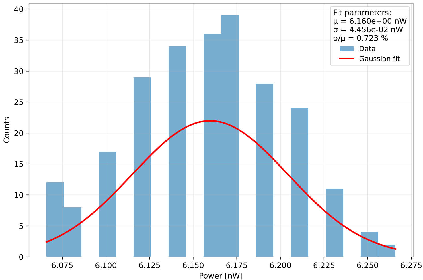
Histogram of power Run 2 (meas. 15) - \lambda=401.0 nm, pulse width=800 ps, PD current = 7.489 pA Start: 2025-11-28 11:03:25, \Delta t=0.1 s, N=244, T=24.3 s
