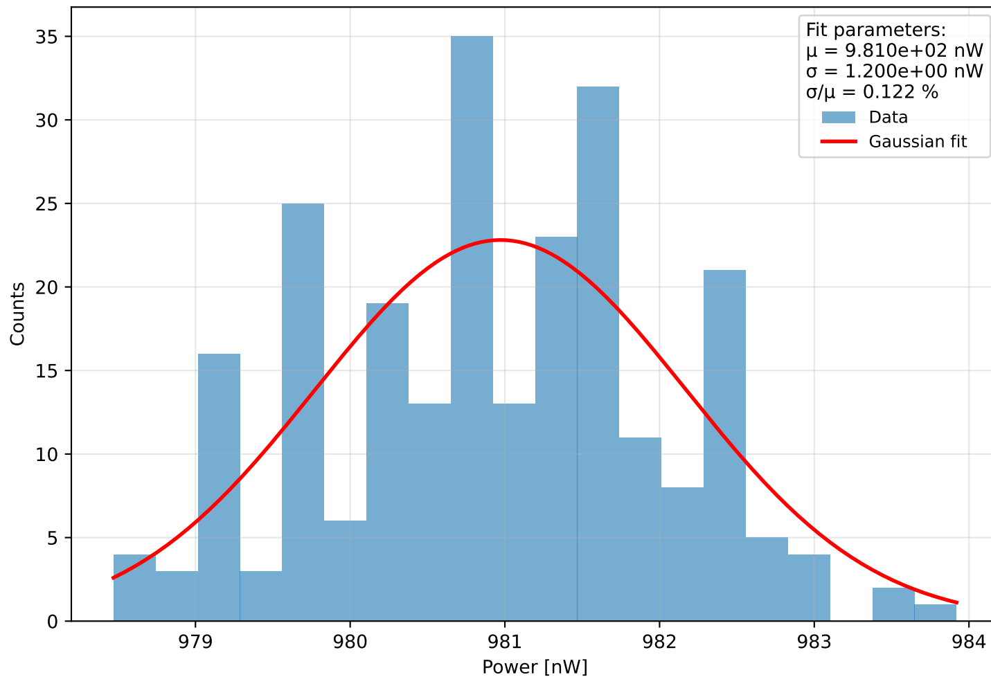
Histogram of power Run 2 (meas. 9) - \lambda=401.0 nm, pulse width=860 ps, PD current = 8.806 pA Start: 2025-11-27 17:41:45, \Delta t=0.1 s, N=244, T=24.3 s
