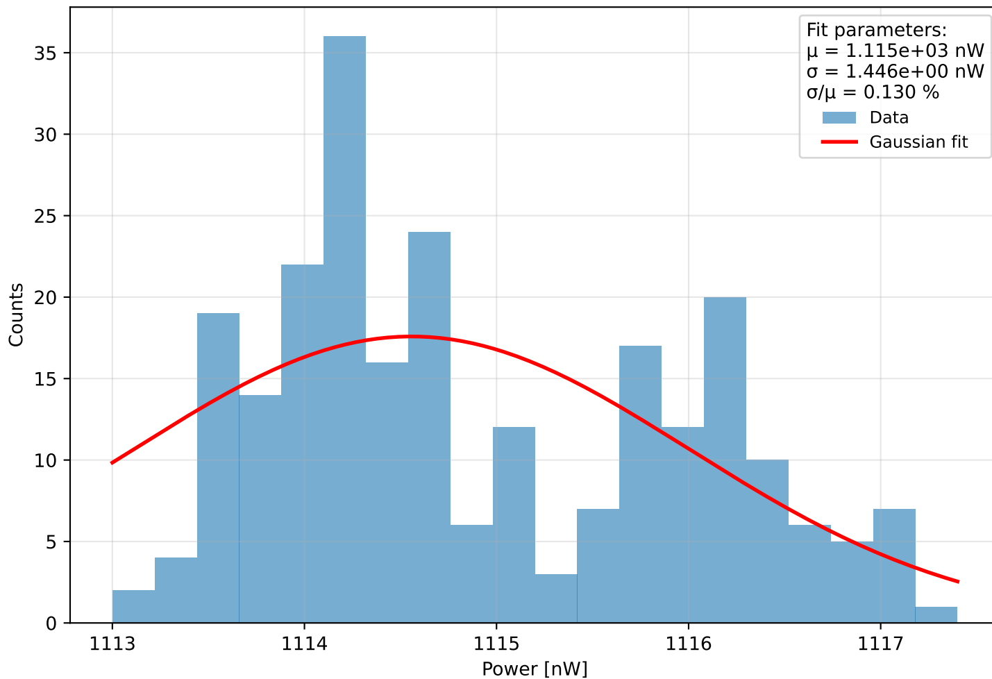
Histogram of power Run 0 (meas. 31) - \lambda=410.0 nm, pulse width=900 ps, PD current = 9.171 pA Start: 2025-11-28 14:25:30, \Delta t=0.1 s, N=243, T=24.2 s
