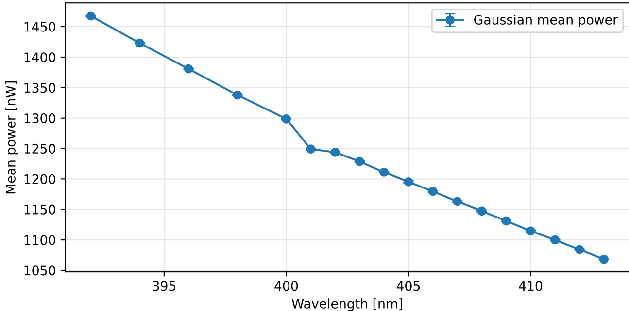
Mean power vs wavelength Pulse width = 900 ps, PD current = 9.171 pA
