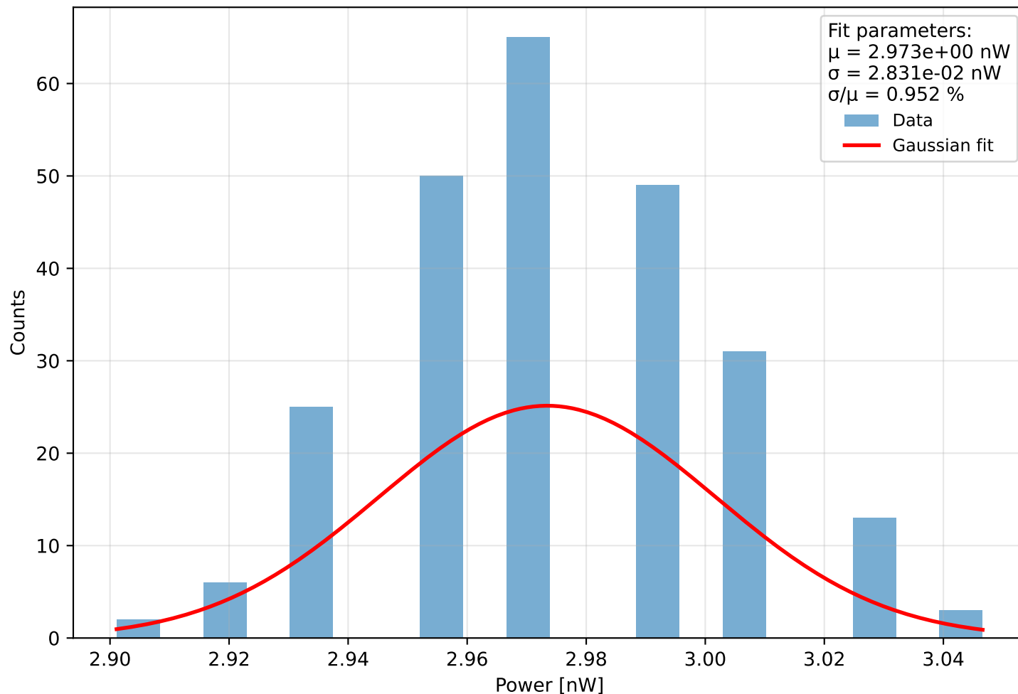
Histogram of power Run 2 (meas. 19) - \lambda=401.0 nm, pulse width=760 ps, PD current = 7.29 pA Start: 2025-11-28 11:48:12, \Delta t=0.1 s, N=244, T=24.3 s
