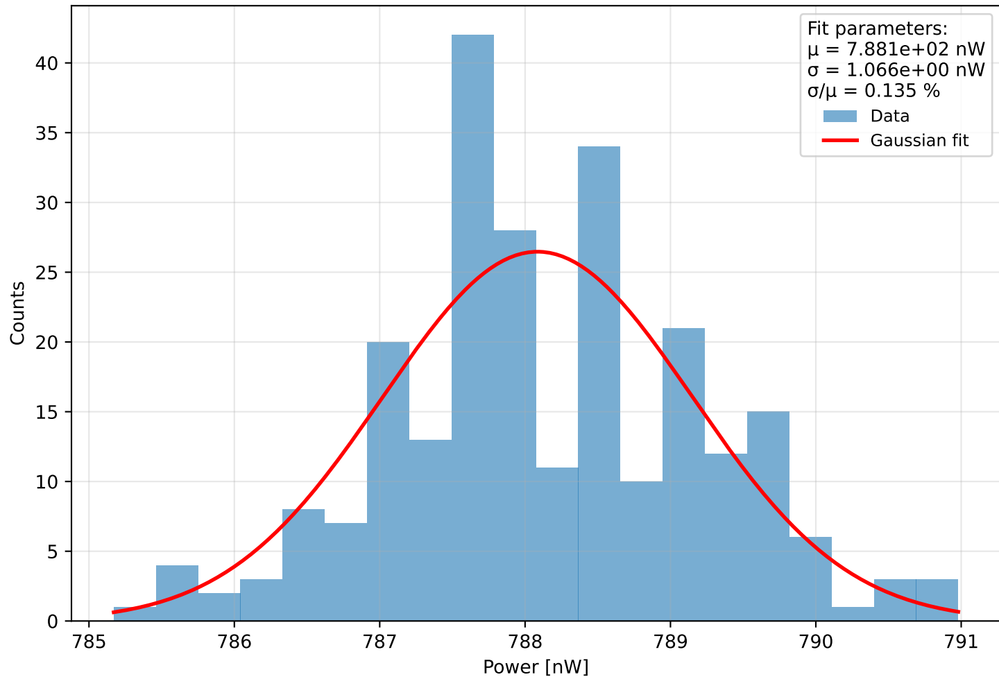
Histogram of power Run 1 (meas. 10) - \lambda=401.0 nm, pulse width=850 ps, PD current = 8.63 pA Start: 2025-11-27 17:44:11, \Delta t=0.1 s, N=244, T=24.3 s
