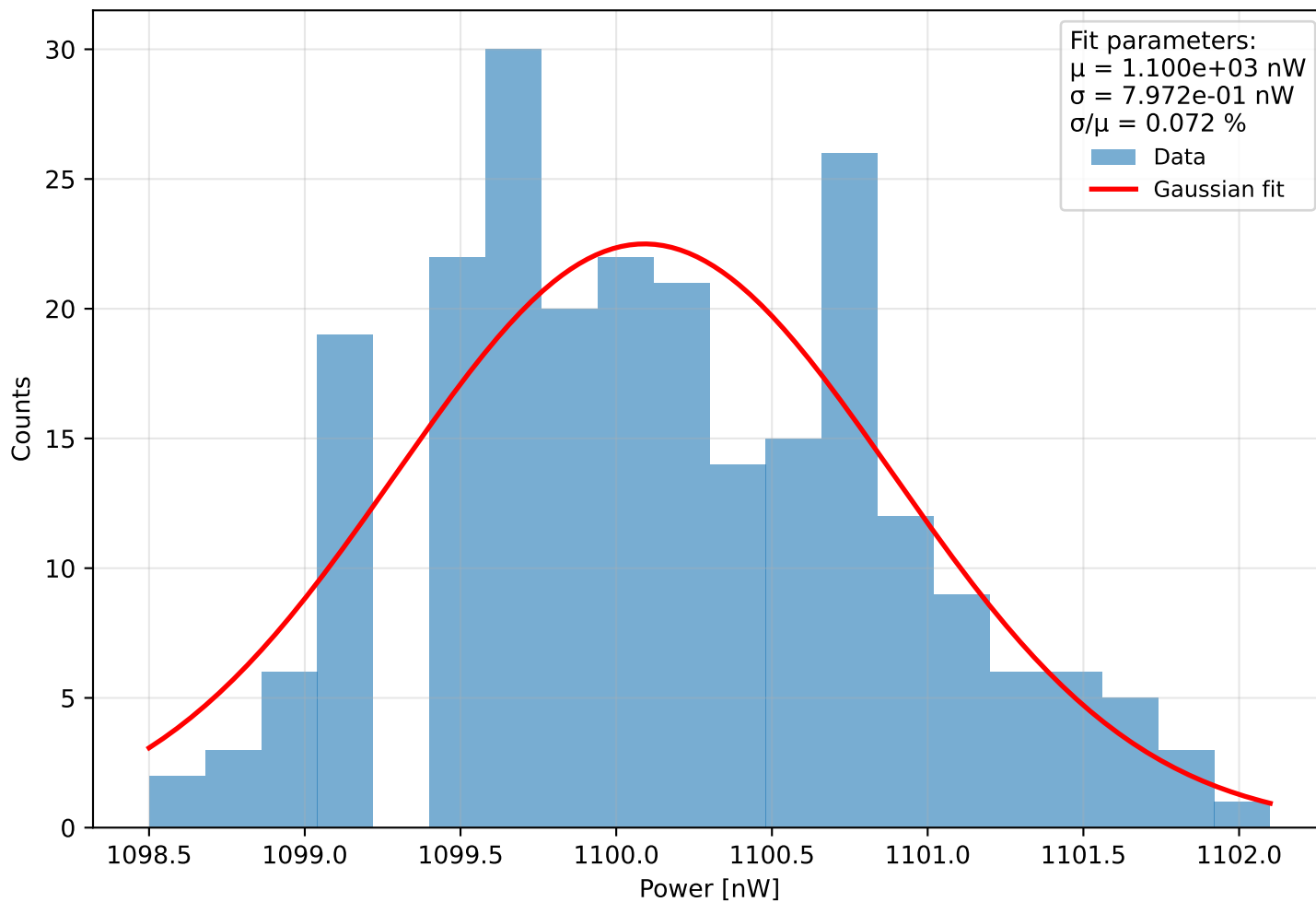
Histogram of power Run 0 (meas. 32) - \lambda=411.0 nm, pulse width=900 ps, PD current = 9.171 pA Start: 2025-11-28 14:27:23, \Delta t=0.1 s, N=242, T=24.1 s
