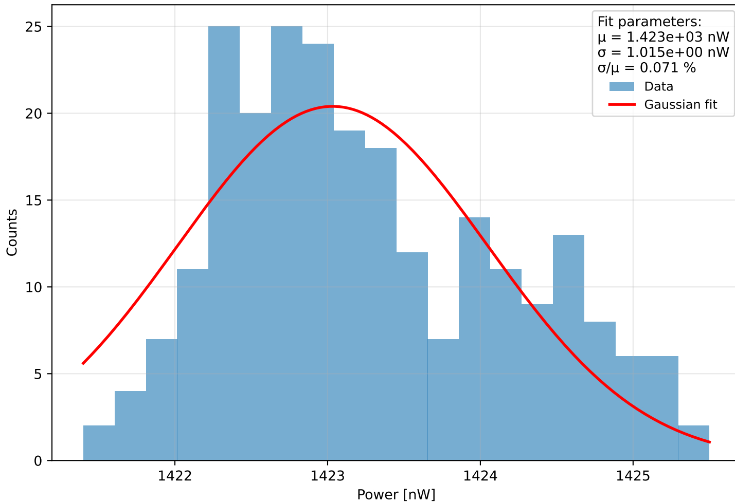
Histogram of power Run 0 (meas. 38) - \lambda=394.0 nm, pulse width=900 ps, PD current = 9.171 pA Start: 2025-11-28 14:37:05, \Delta t=0.1 s, N=243, T=24.2 s
