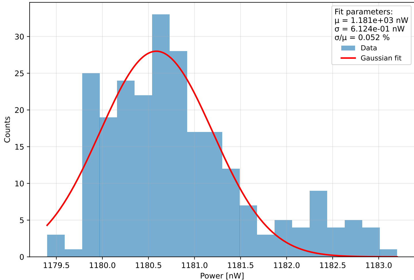
Histogram of power Run 0 (meas. 6) - \lambda=401.0 nm, pulse width=890 ps, PD current = 9.048 pA Start: 2025-11-27 17:07:46, \Delta t=0.1 s, N=243, T=24.2 s
