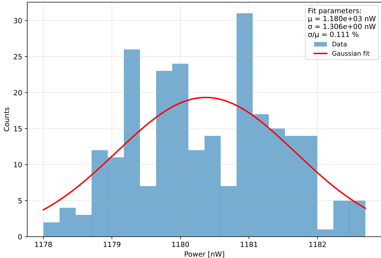
Histogram of power Run 1 (meas. 6) - \lambda=401.0 nm, pulse width=890 ps, PD current = 9.048 pA Start: 2025-11-27 17:12:59, \Delta t=0.1 s, N=247, T=24.6 s
