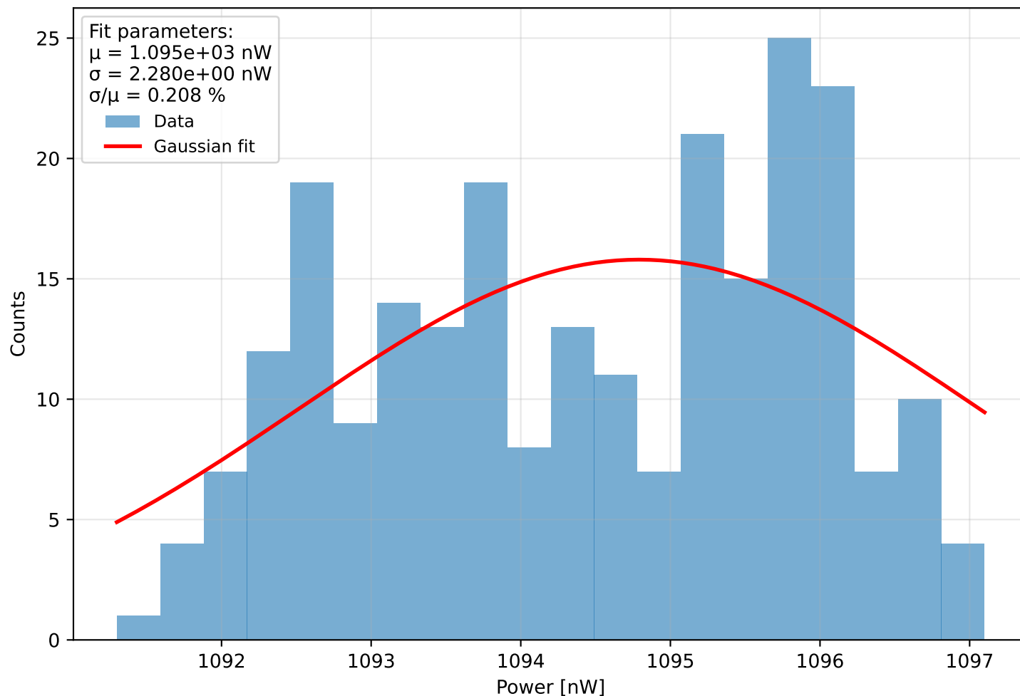
Histogram of power Run 0 (meas. 8) - \lambda=401.0 nm, pulse width=870 ps, PD current = 8.926 pA Start: 2025-11-27 17:32:41, \Delta t=0.1 s, N=242, T=24.1 s
