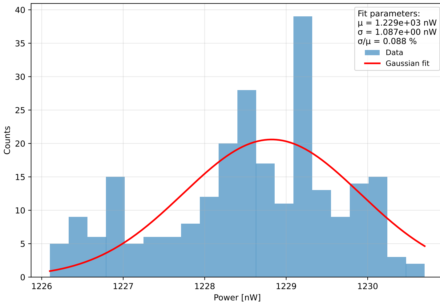
Histogram of power Run 0 (meas. 24) - \lambda=403.0 nm, pulse width=900 ps, PD current = 9.171 pA Start: 2025-11-28 14:10:11, \Delta t=0.1 s, N=243, T=24.2 s
