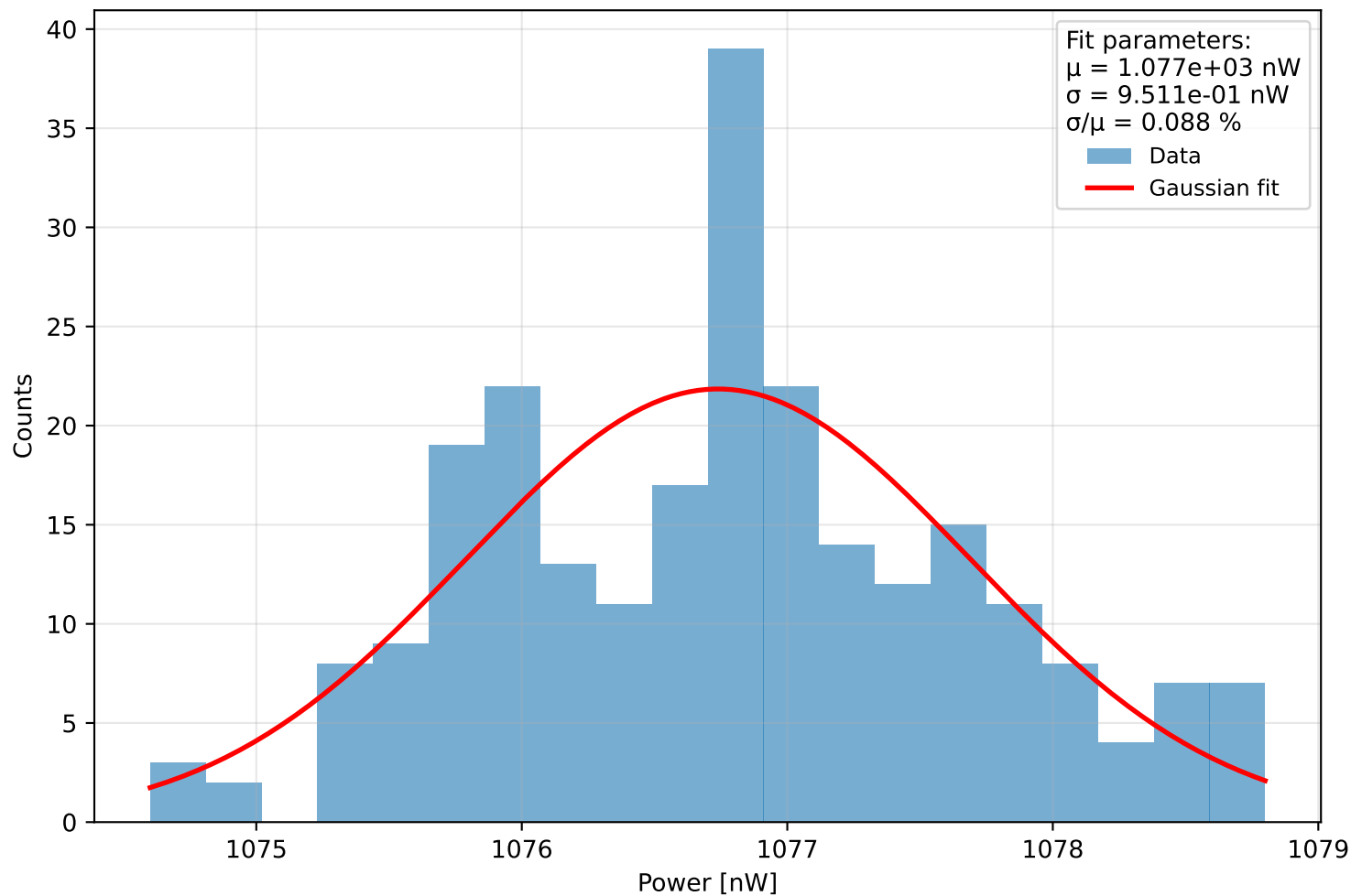
Histogram of power Run 0 (meas. 7) - \lambda=401.0 nm, pulse width=880 ps, PD current = 8.926 pA Start: 2025-11-27 17:30:38, \Delta t=0.1 s, N=243, T=24.2 s
