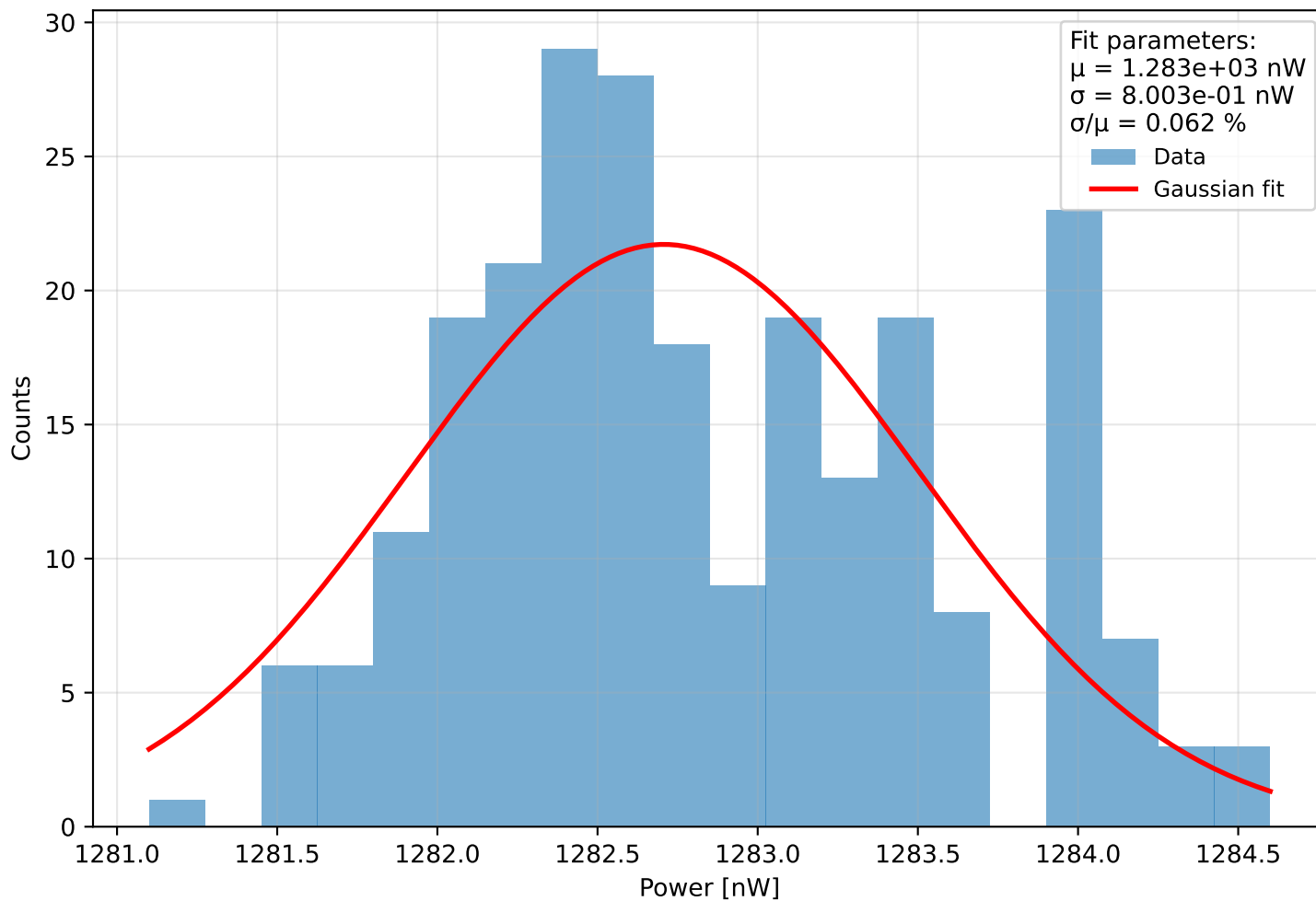
Histogram of power Run 1 (meas. 21) - \lambda=401.0 nm, pulse width=900 ps, PD current = 9.171 pA Start: 2025-11-28 12:00:23, \Delta t=0.1 s, N=243, T=24.2 s
