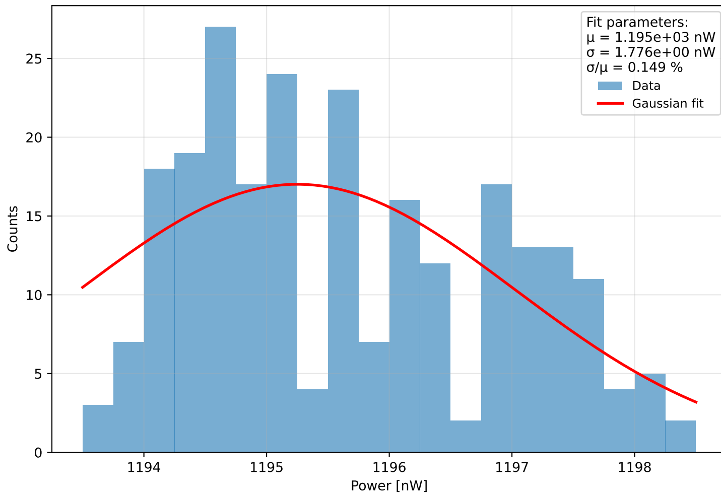
Histogram of power Run 0 (meas. 26) - \lambda=405.0 nm, pulse width=900 ps, PD current = 9.171 pA Start: 2025-11-28 14:12:56, \Delta t=0.1 s, N=244, T=24.3 s
