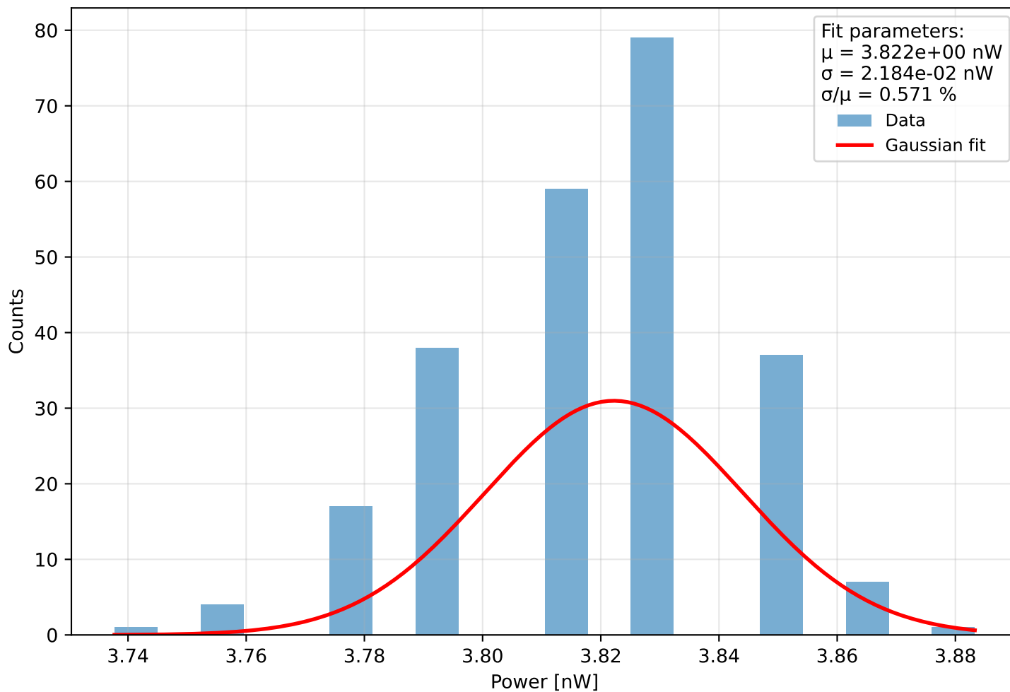
Histogram of power Run 0 (meas. 18) - \lambda=401.0 nm, pulse width=770 ps, PD current = 7.389 pA Start: 2025-11-28 11:38:52, \Delta t=0.1 s, N=243, T=24.2 s
