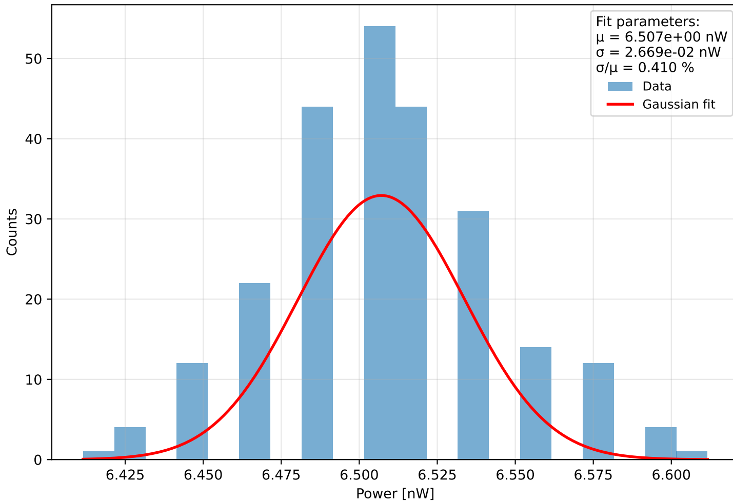
Histogram of power Run 3 (meas. 17) - \lambda=401.0 nm, pulse width=780 ps, PD current = 7.489 pA Start: 2025-11-28 11:26:44, \Delta t=0.1 s, N=243, T=24.2 s
