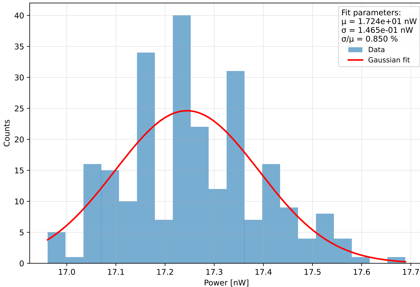
Histogram of power Run 0 (meas. 16) - \lambda=401.0 nm, pulse width=790 ps, PD current = 7.591 pA Start: 2025-11-28 11:05:16, \Delta t=0.1 s, N=243, T=24.2 s
