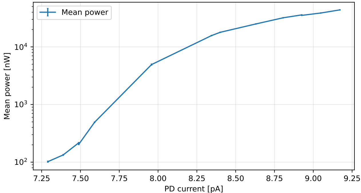
Mean power vs PD current
