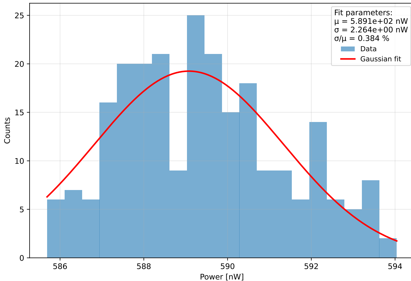
Histogram of power Run 2 (meas. 11) - \lambda=401.0 nm, pulse width=840 ps, PD current = 8.4 pA Start: 2025-11-27 17:48:16, \Delta t=0.1 s, N=243, T=24.2 s
