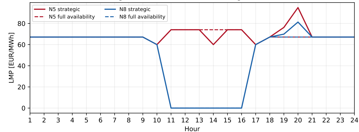
Congested load node N5 and storage node N8
