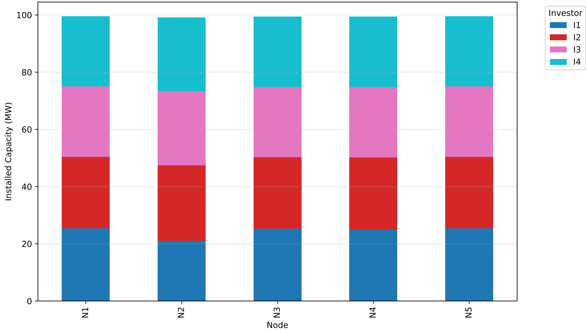
Output: Installed BESS Power Capacity by Node and Investor
