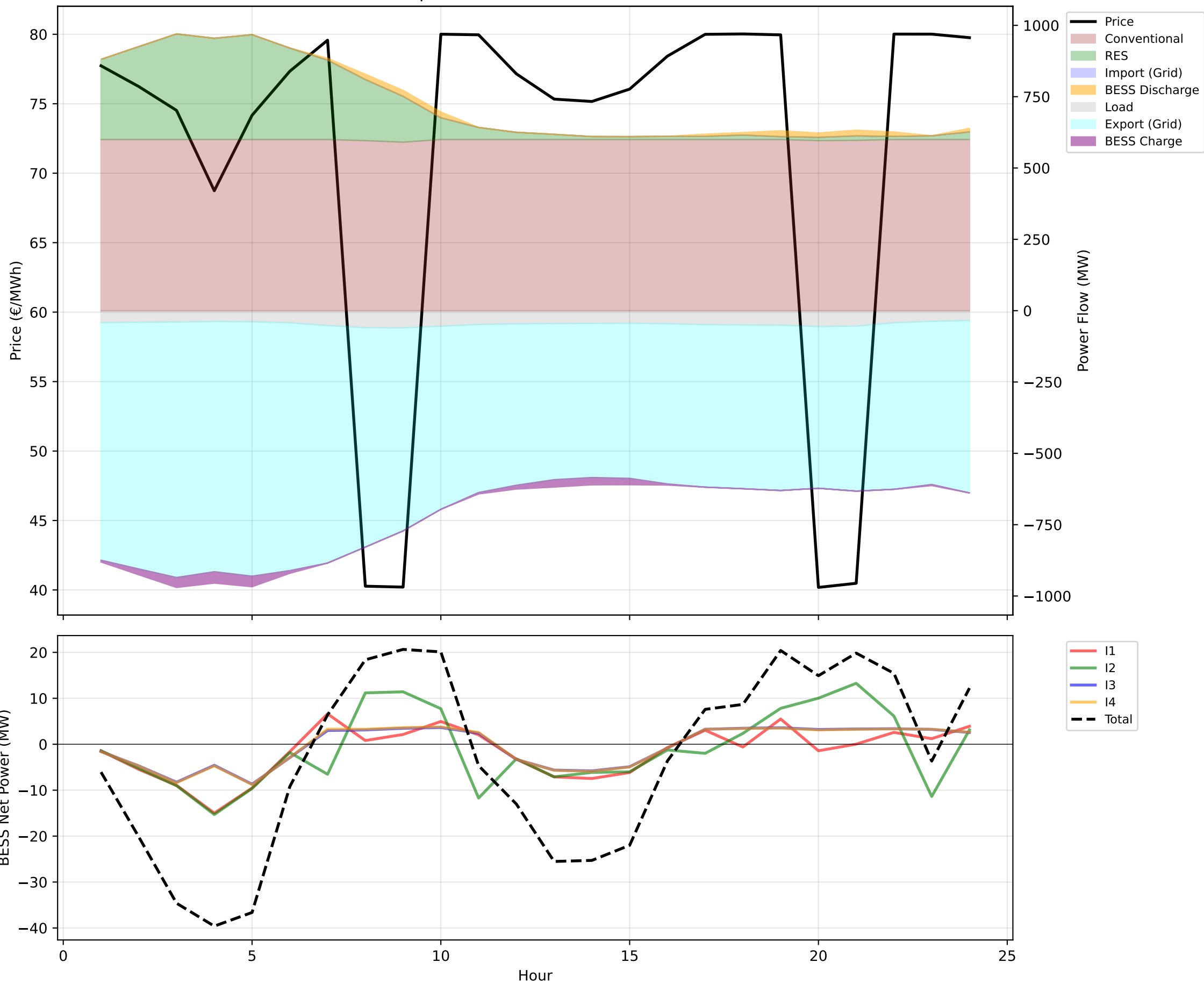
Output: Node N1 Balance & Prices
