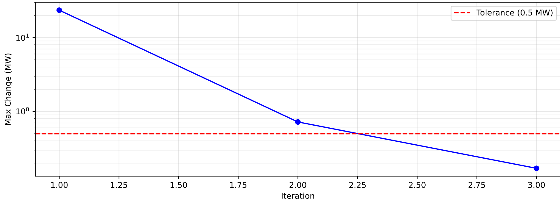
Output: Convergence History (Max Delta per Iteration)
