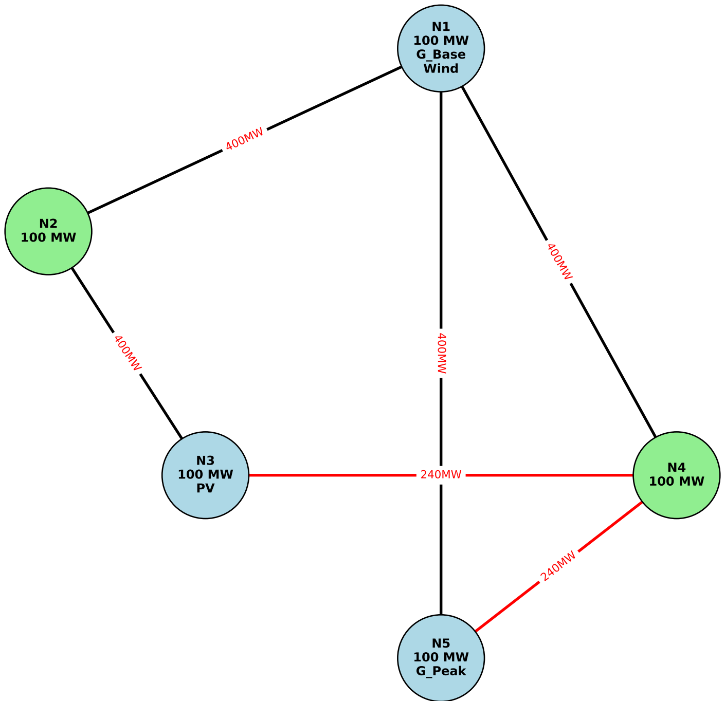
Grid topology: Node and line limits
