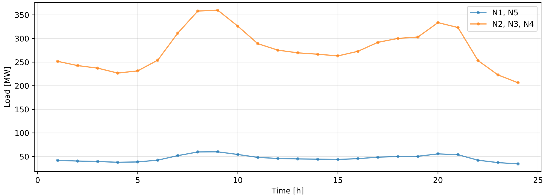
Input: Load Profiles
