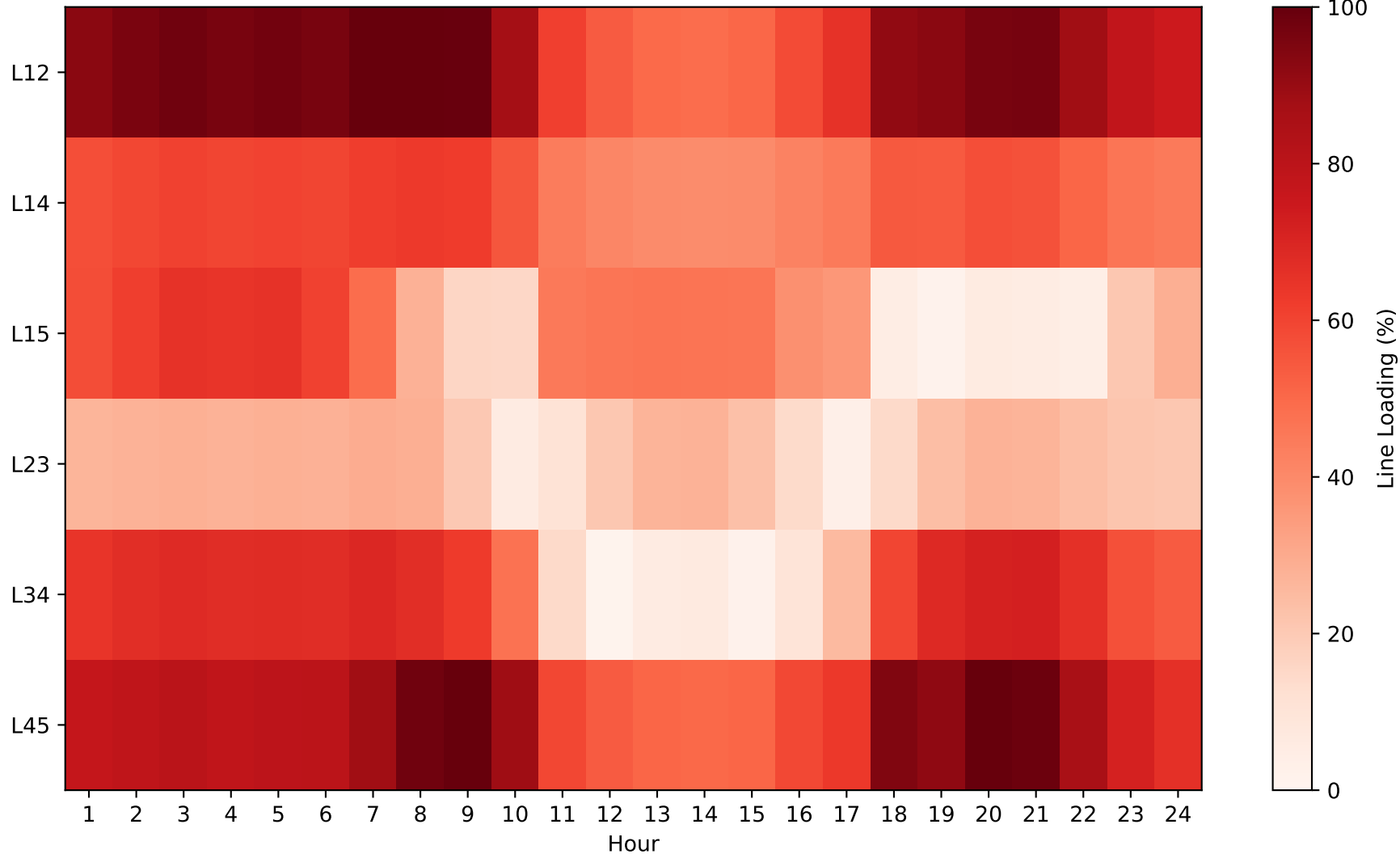
Output: Line Congestion Heatmap
