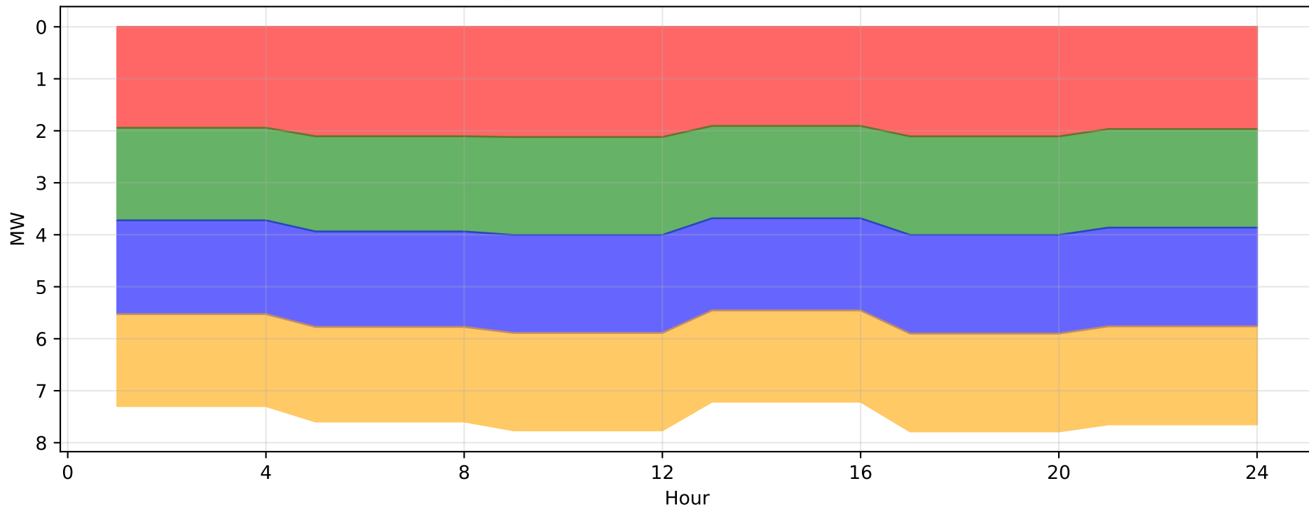
Output: Node N2 aFRR Provision DOWN
