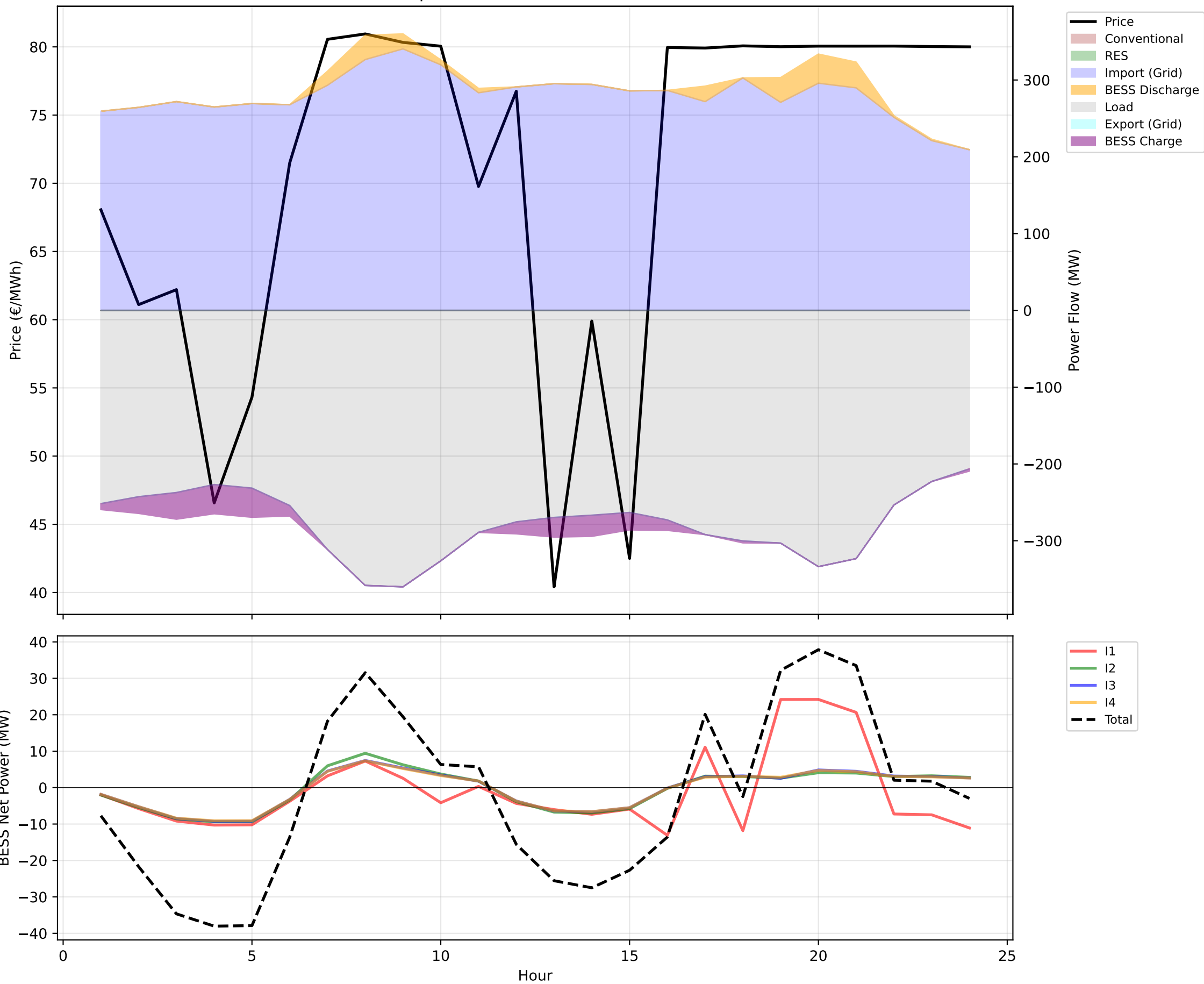
Output: Node N4 Balance & Prices
