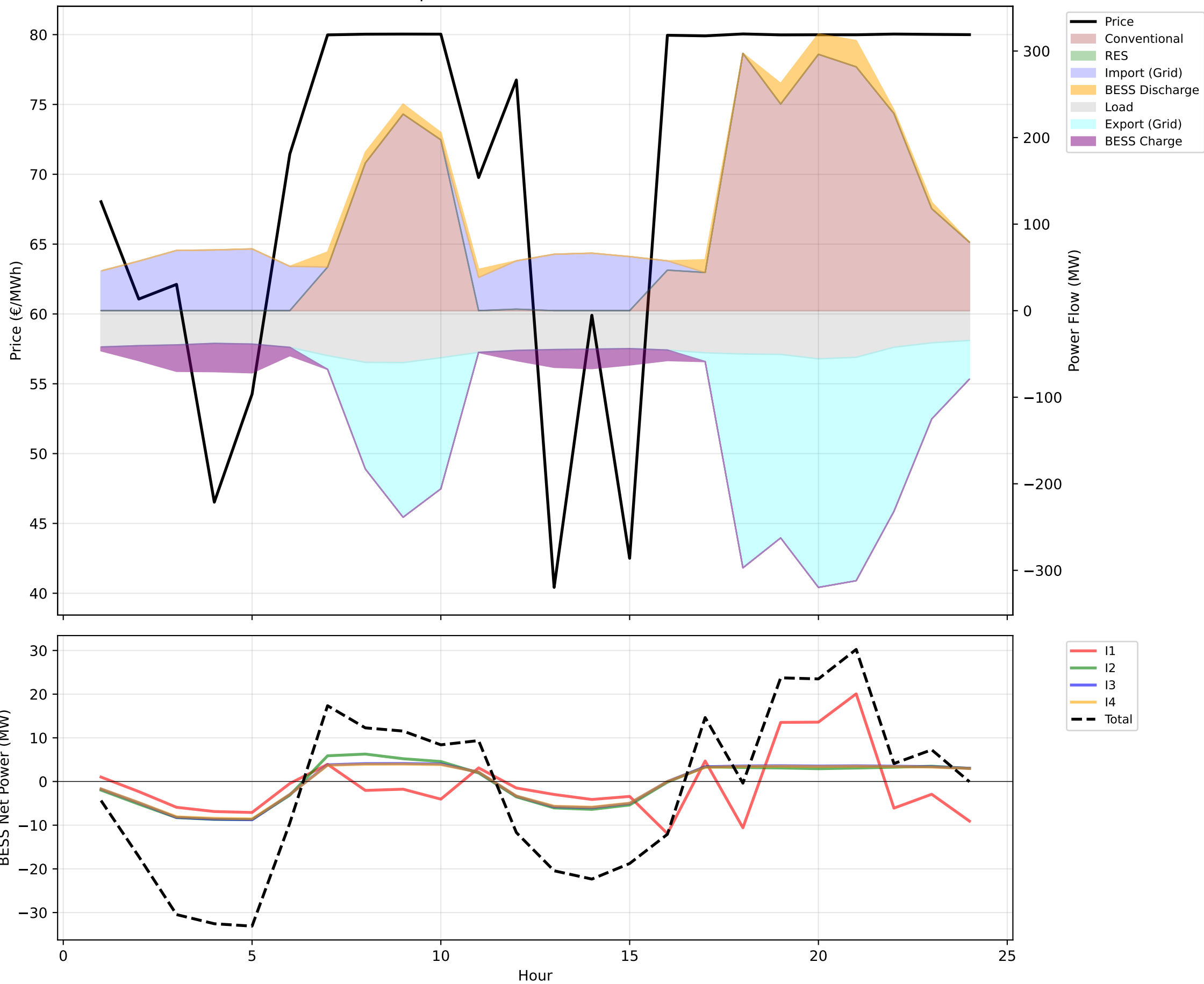
Output: Node N5 Balance & Prices
