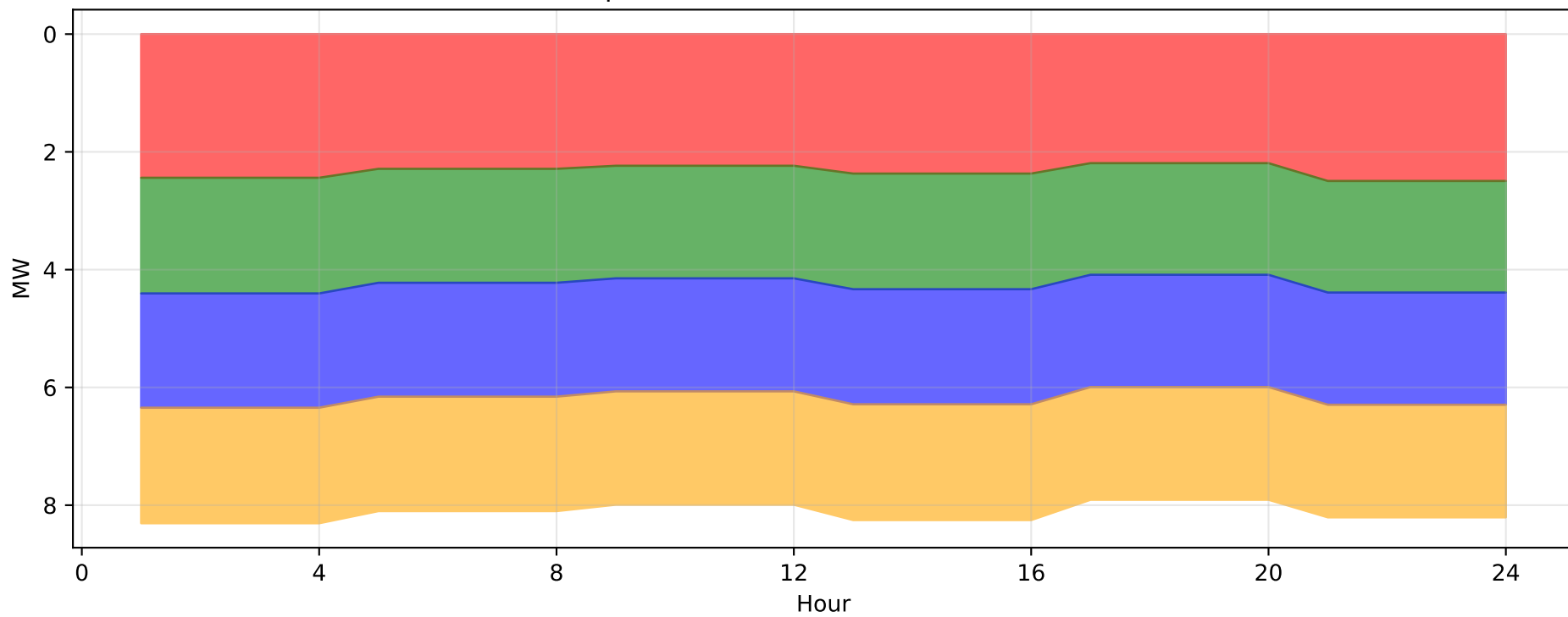
Output: Node N5 aFRR Provision DOWN
