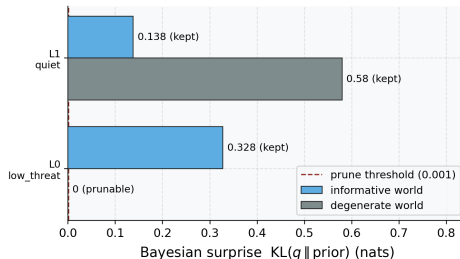
Figure 1: Per-level Bayesian surprise and prune/keep decisions for two hierarchical worlds. Source relation: original project BMR structure-learning diagnostic related to the mechanism in Friston et al. Fig. 9; estimand: per-level Bayesian surprise in nats and the resulting prune/keep decision; uncertainty: deterministic schematic worlds, so no resampling interval is shown. Per-level Bayesian surprise for the two 3-level worlds. y-axis: the non-leaf reduction targets, indexed top-down from the reduction routine as level 0 = the meta-context (the topmost non-leaf level, L3 in the location-first L1/L2/L3 convention used elsewhere) and level 1 = the context (L2); the leaf location level (L1) is never a reduction target. x-axis: Bayesian surprise KL(q \parallel \text{prior}) in nats — the information the leaf observation added at that level. Blue bars: the informative world (top level kept). Grey bars: the degenerate world (top level prunable). The dashed red line is the prune threshold; a level whose surprise falls below it is structurally unnecessary. The degenerate meta-context (grey, level 0) sits at 0.000 nats and is pruned, recovering the two-level model, while the informative meta-context (blue, level 0) at 0.328 nats is retained; both worlds keep the context level (level 1). Deterministic schematic worlds (no resampling), so no error band is applicable.
