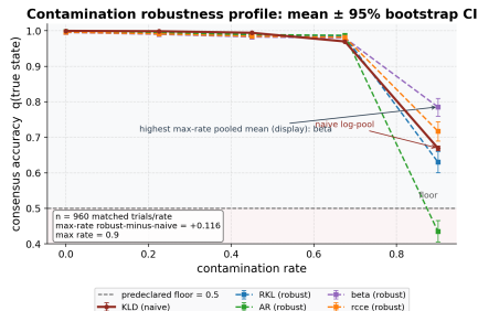
Figure 1: Consensus accuracy: probability mass assigned to the true hidden state. The plotted estimand is q(\text{true state}) . Source relation: original project robustness extension; estimand: true-state probability mass; uncertainty: matched-trial percentile-bootstrap intervals over configured trials. The colony of 7 sentinel agents (acuity 0.55, of which 2 are saboteurs) as a function of contamination rate. x-axis: saboteur convex-mix contamination rate, sampled over \{0, 0.225, 0.45, 0.675, 0.9\} ; y-axis: consensus accuracy q(\text{true state}) (probability mass on the true hidden state). One curve per configured server operating point: standard KLD plus the robust robust_aggregate settings
