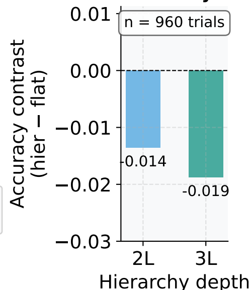
F Final accuracy contrast
