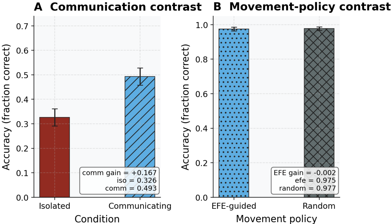
Figure 27: Communication improves the declared disjoint-view condition, whereas the configured movement-policy contrast is near-ceiling and null. This is a source-inspired project extension of the moving-world mechanism, produced from two separately configured reports. Source relation: original project extension of the source-inspired moving-world mechanism. Estimand: condition-level final consensus accuracy. Read left to right. Panel A compares isolated and communicating consensus for 3 agents, each observing a non-overlapping 2-position window of a 6-position world. Panel B compares EFE-guided and random movement for 2 agents in a 4-position world. The x-axis is the condition or movement policy; the y-axis is final consensus accuracy, the fraction of trials whose pooled argmax equals the true state. Direct x-axis labels, distinct hatches, dark keylines, and printed summary boxes duplicate color. Bars are means across independent configured seeds; error bars are across-seed standard deviations, not confidence intervals. Trials and agents are nested within each seed. The paired Wilcoxon results are p = 9.35 \times 10^{-23} for Panel A and p = 0.1046 for Panel B. The first supports only the configured communication contrast; the second records the observed null rather than an EFE benefit. The panels do not establish universal communication necessity, movement-policy superiority, causal mechanism, or generalization beyond the declared worlds and seed schedule.
