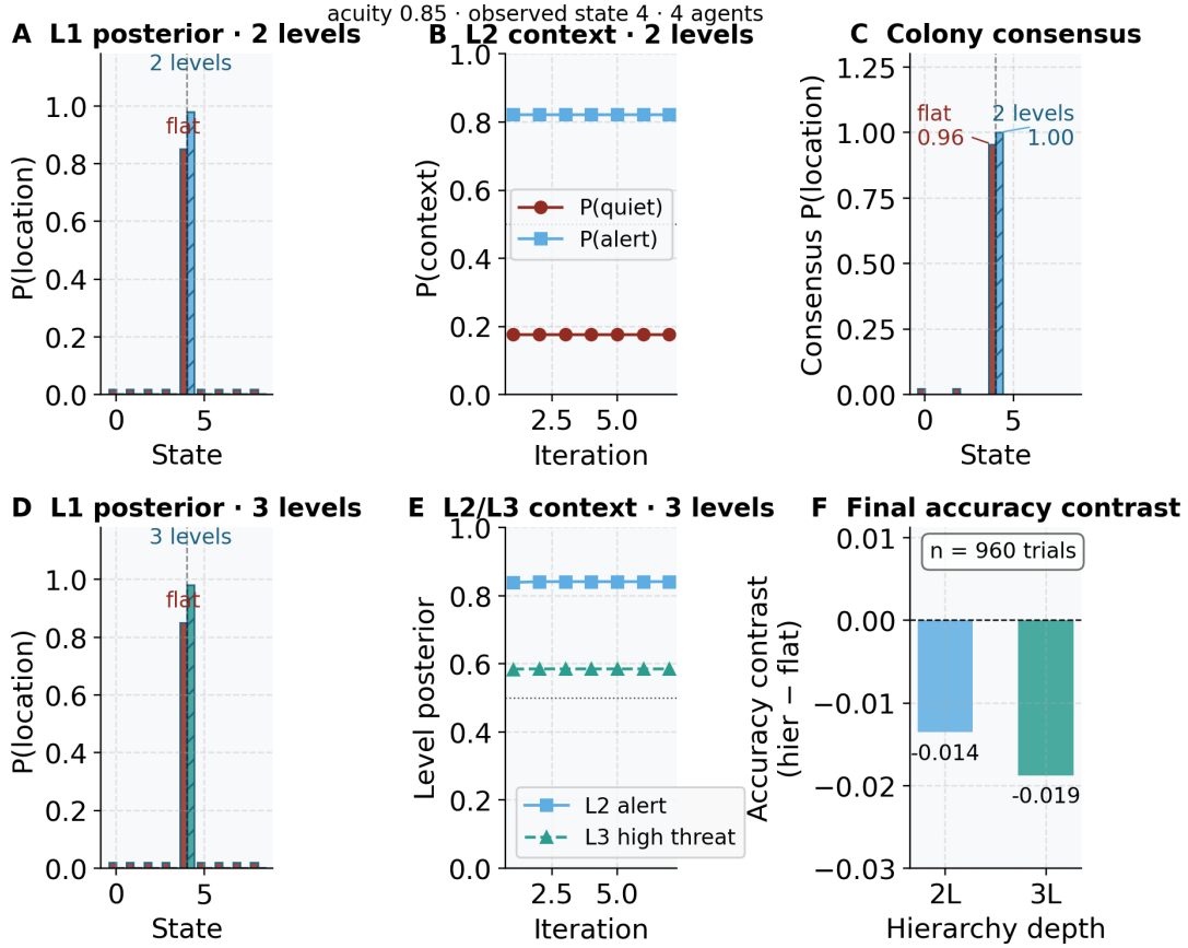
Figure 28: Six-panel hierarchical POMDP belief-dynamics and accuracy diagnostic. Source relation: source-inspired original project diagnostic for a hierarchical extension; estimand: posterior probabilities and final hierarchical-minus-flat location-accuracy gap in the declared seeded protocol. Read the two-level world across the top row and the three-level extension across the bottom. In the left column, the x-axis indexes 9 location states and the y-axis is posterior probability after one center-cell observation; plain left-offset bars are the flat-prior reference and forward-hatched right-offset bars are hierarchical. In the middle column, the x-axis is alternating-minimization iteration and the y-axis is context probability; circles, squares, triangles, and solid or dashed paths identify the displayed levels without color. The top-right panel uses the same plain-versus-hatched bar grammar for L1 consensus after federating 4 agents, with direct peak labels. The bottom-right panel's x-axis is hierarchy depth and its y-axis is the final accuracy-fraction contrast over 960 nested trials, with direct signed values and a zero rule. Units are probability or accuracy fraction. Seed 0 defines one deterministic protocol realization; ordered states, iterations, agents, and trials are nested measurements rather than independent resampling units, so no interval or error band applies. The figure does not establish universal hierarchical benefit, calibrated uncertainty, or source-protocol replication.
