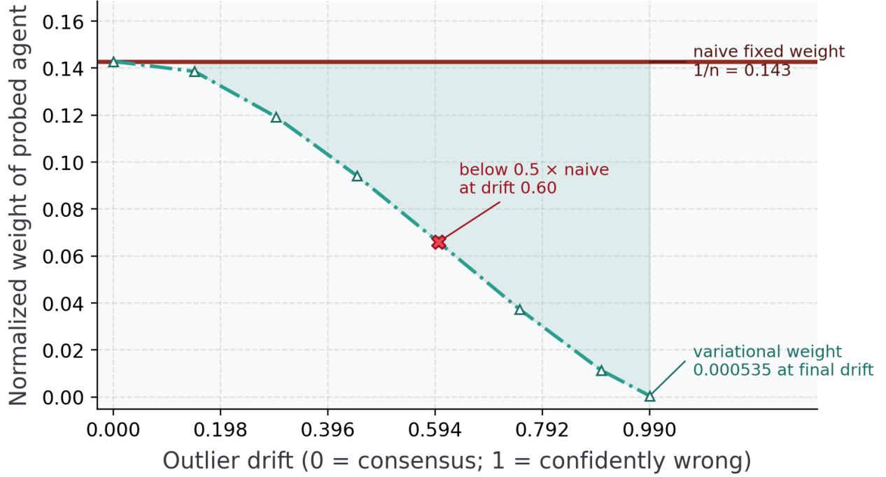
Figure 17: Normalized influence weight of one probed agent. Source relation: original project variational-server diagnostic; estimand: the probed agent’s normalized server weight as its posterior drifts toward a confident-wrong delta. The x-axis is outlier drift from consensus at zero to the wrong-state delta at one; the y-axis is normalized influence weight. The open-triangle dash-dot path is variational_aggregate ; the circle-solid horizontal reference is the naive log-linear pool. Direct endpoint labels name both rules and values, shaded separation shows their tested-path gap, and an adversarial X with an arrow marks the first displayed point below one-half of the naive weight. As drift becomes extreme, the variational weight falls below 0.001, whereas the naive pool remains fixed at 1/n = 0.143 . This deterministic seeded sweep contains n = 7 agents in one configured colony; drift points are ordered evaluations, not independent replications, so no confidence interval or error band applies. The pattern is redescending normalized weight along this path, while the algebraic property bounds raw effective weight; the figure is not an estimator-level B-robustness proof and does not transfer the property to the sharper robust_aggregate heuristic.
