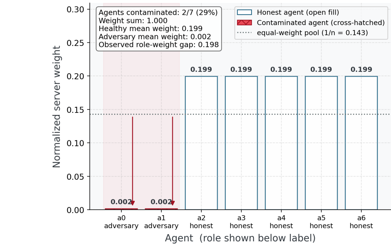
Normalized heuristic server weights by declared agent role
