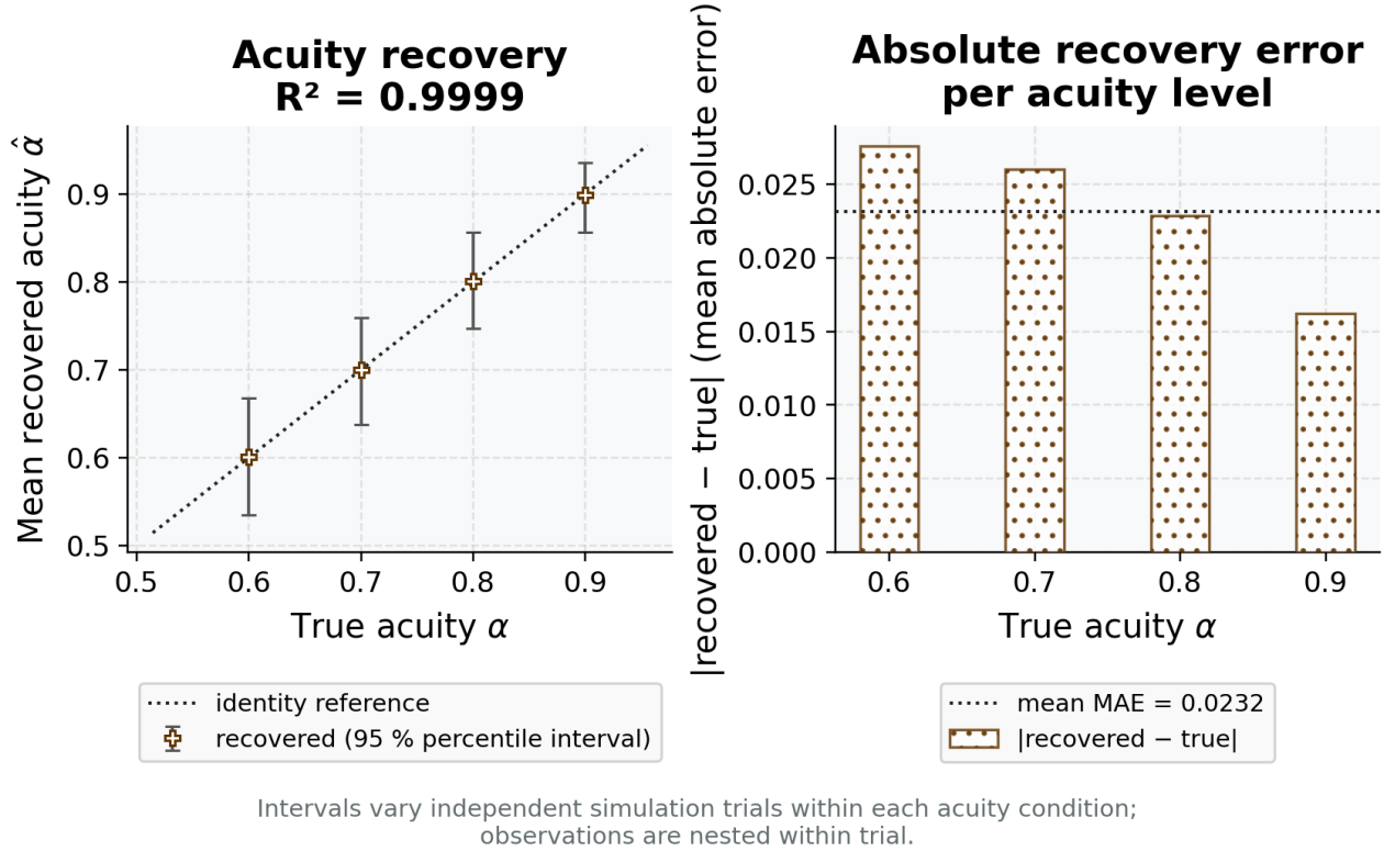
Figure 31: Two-panel parameter-recovery diagnostic. Source relation: original project parameter-recovery study; estimands: recovered acuity and absolute error in probability units, plus the unitless coefficient of determination R^2 for mean recovered versus true acuity. In the left panel, the x-axis is true acuity and the y-axis is mean recovered acuity. Open estimate markers with capped error bars show the 95% empirical percentile interval across 960 independent synthetic trials within each true-acuity grid point; the dark dotted diagonal is identity, and the title reports R^2 = 0.9999 . This interval is a descriptive quantile of independent-trial estimates, not a bootstrap confidence interval or Bayesian credible interval. In the right panel, the x-axis is tested true acuity and the y-axis is absolute acuity error. Open dotted-hatch bars distinguish the errors without color, and a labeled dark dotted rule marks global mean absolute error. Each trial contains 200 nested observations. The configured seed initializes the base RNG stream and is not the independent analysis unit. These finite-grid estimates do not establish global structural identifiability or recovery outside the tested observation model.
