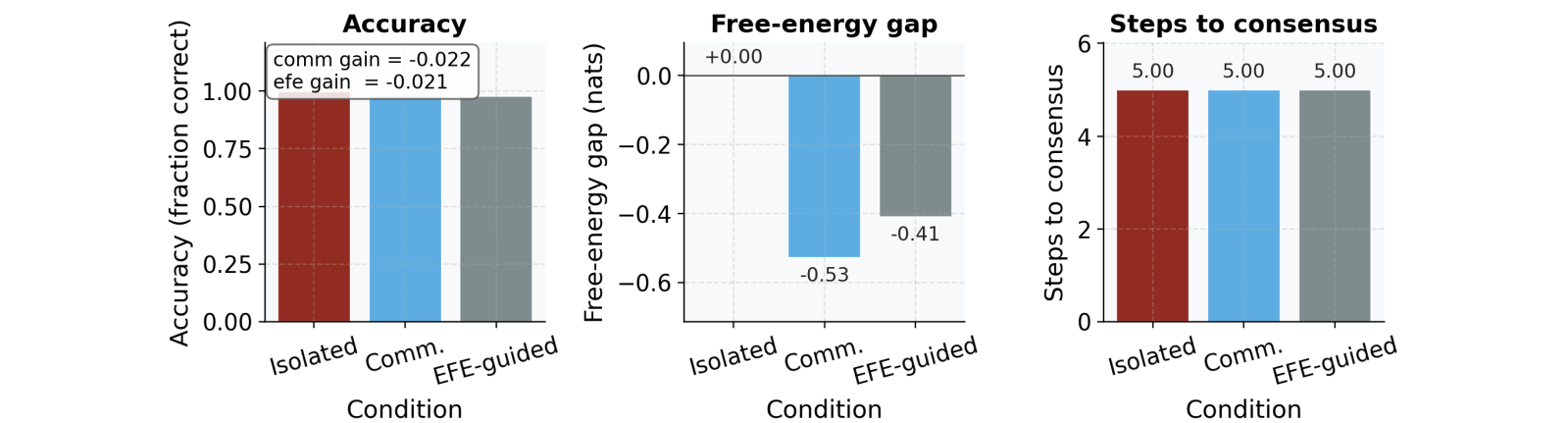
Figure 23: Moving sentinel world across isolated, communicating, and EFE-guided conditions. Source relation: original project schematic for the moving-world protocol; estimand: condition-level consensus accuracy, signed free-energy gap, and steps-to-consensus proxy in the stated native units; uncertainty: deterministic seeded run, so no resampling interval is shown. Moving sentinel world across the three conditions (x-axis is condition: isolated, communicating, EFE-guided). Left panel: y-axis shows consensus accuracy (fraction of 960 trials whose pooled argmax matches the truth). Center panel: y-axis shows the signed free-energy gap in nats (isolated surprise minus the condition’s surprise on the true state, so a positive value would mean lower free energy than isolated; the measured gaps are negative, plotted against a zero reference line and annotated per bar). Right panel: y-axis shows a coarse steps-to-consensus proxy, with per-bar value annotations showing the three conditions are essentially tied. Each colony runs 6 steps over a 4-cell linear grid with 2 disjoint-FOV agents. Deterministic seeded run, so the bars carry no error band.
