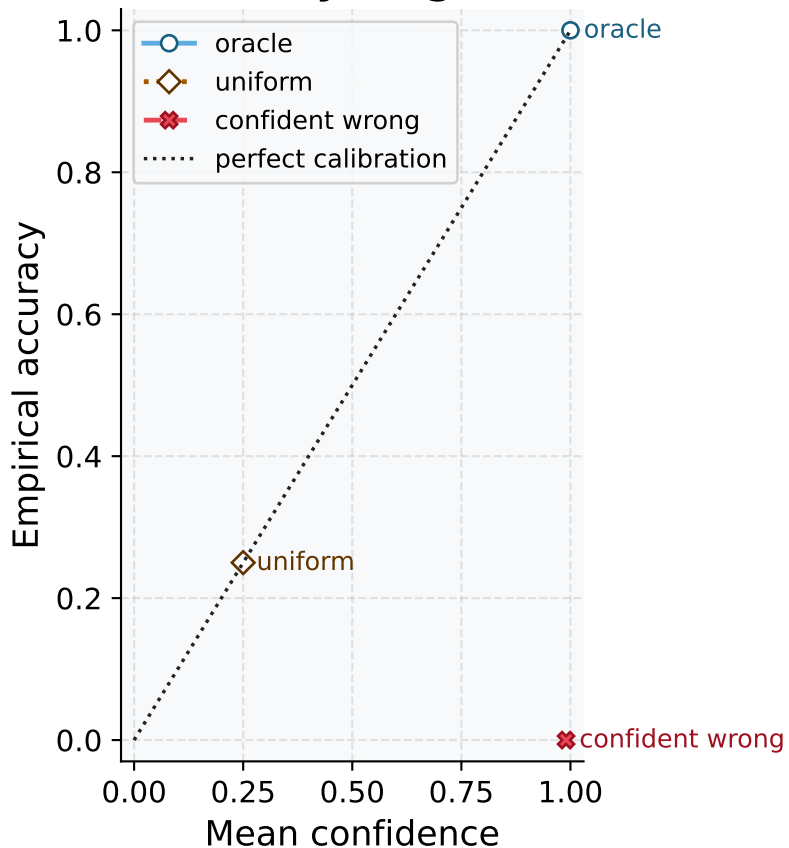
Reliability diagnostic
