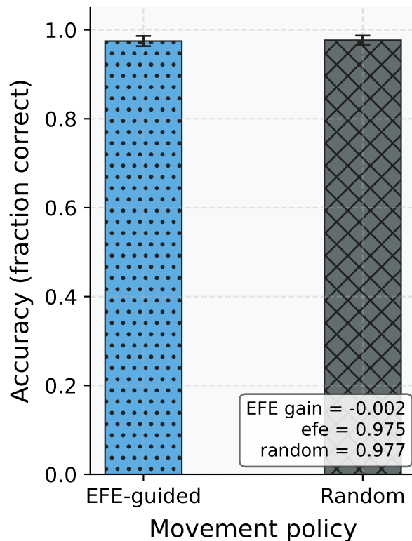
B Movement-policy contrast
