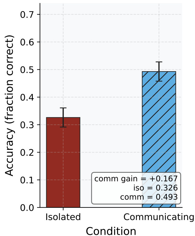
A Communication contrast
