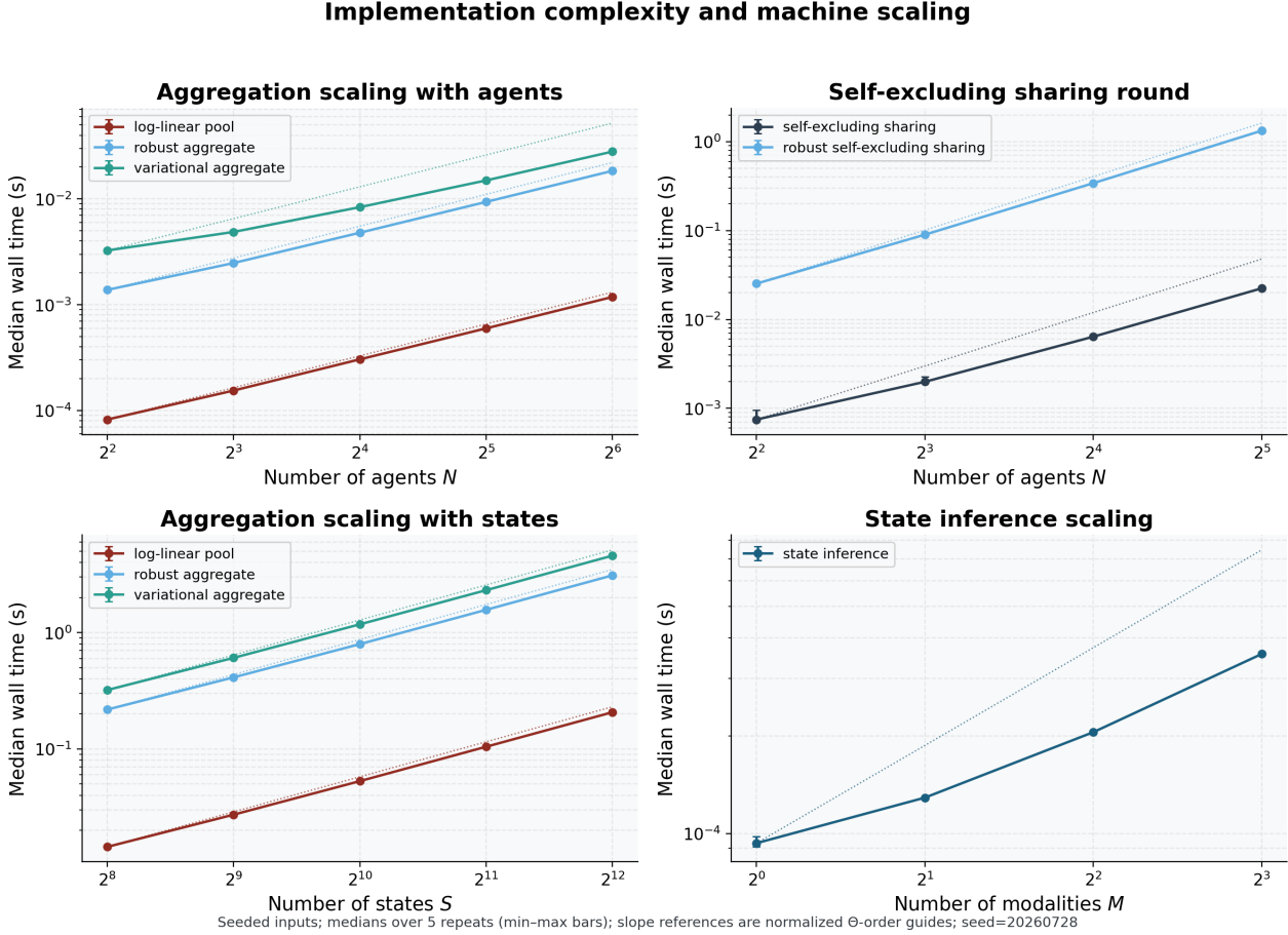
Figure 6: Implementation-derived complexity and seeded machine-scaling diagnostic. Source relation: original project computational-complexity diagnostic; estimand: median wall-clock time of the real categorical aggregation, naive and robust self-excluding sharing, and state-inference call paths as the declared dimension changes; uncertainty: min-max span over the repeated timings, not a confidence interval; replication unit: fixed seeded input at each grid point with the declared timing repeats. The x-axis is the varied agent, state, or modality dimension, and the y-axis is median wall-clock time in seconds. The panels show agent scaling for the aggregation rules, naive and iterative-robust N^2 leave-one-out sharing, state scaling for the aggregators, and modality scaling for one-step inference. Dotted lines are normalized \Theta -order guides from the implementation-derived accounting; they are not fitted claims. The experiment ran on arm64 with Python 3.13.11, NumPy 2.4.2, seed 20260728, and 5 measured repeat(s) after 1 warmup(s).
