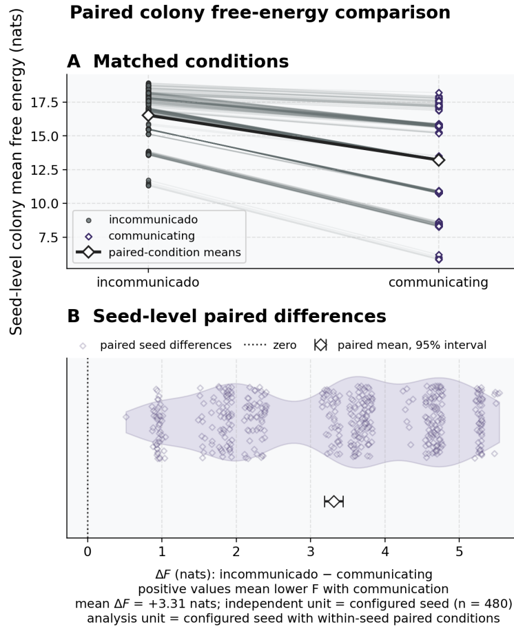
Figure 9: Paired colony-mean variational free energy under communication and isolation. Source relation: reduced categorical source-mechanism analogue of Friston et al. (2024), Fig. 5; estimand: seed-level \Delta\bar{F} = \bar{F}_{\text{solo}} - \bar{F}_{\text{share}} in nats, where positive values indicate lower free energy with communication. In Panel A, the x-axis is communication condition and the y-axis is colony-mean free energy. Filled reference circles mark incommunicado values, open comparison diamonds mark communicating values, fine connecting slopes preserve within-seed pairing, and open diamonds joined by a dark line identify condition means. In Panel B, the x-axis is paired difference and the y-axis is jitter only, with one open diamond per seed, a translucent distribution envelope, a dark dotted zero rule, and an open-diamond mean with its 95% percentile-bootstrap interval. The mean difference is 3.3109 nats across n = 480 independent seeds. Agents and ordered steps remain nested within seed; the interval resamples seeds, not agents, worlds, or deployments. This reduced-protocol result does not establish a general communication benefit or exact source-protocol replication.
