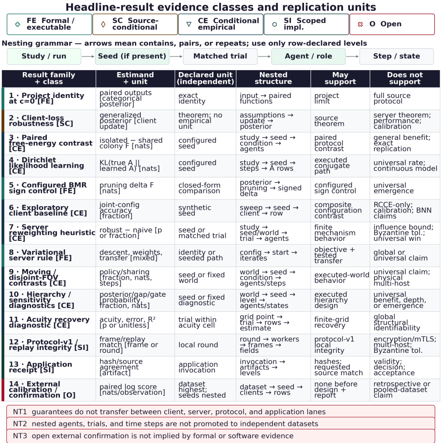
Figure 6: Evidence class and replication remain result-family specific; guarantees do not migrate between client, server, study, protocol, and application evidence. Source relation: source-owned headline-result and claim-owner classification; status: deterministic evidence map, not an empirical result. Fourteen numbered rows align each headline family or public boundary with six fields: class, estimand and unit, independent unit, nesting, permitted support, and prohibited support. The rows retain paired belief-sharing free energy, Dirichlet learning, configured BMR, moving/disjoint-field worlds, hierarchy/sensitivity, acuity recovery, and tempered transfer alongside formal, server, protocol, application, and open-confirmation lanes. A top strip supplies the generic grammar from study or run through seed when present, matched trial or condition, agent or contamination role, and ordered step or posterior state; three bottom boxes state the no-transfer boundaries. The x-axis indexes six evidence fields; the y-axis indexes fourteen result families. Class symbols, keylines, row numbers, and direct labels duplicate color. The estimand and unit are row-specific. No uncertainty belongs to this deterministic map; underlying intervals resample the independent unit named on their row while lower levels remain nested. Exact estimates remain in typed reports and the native-unit cross-study summary. The figure does not establish source-dataset confirmation, isolate an RCCE-only effect, transfer a client theorem to a server rule, promote nested observations to independent datasets, or turn software integrity into scientific validity.
