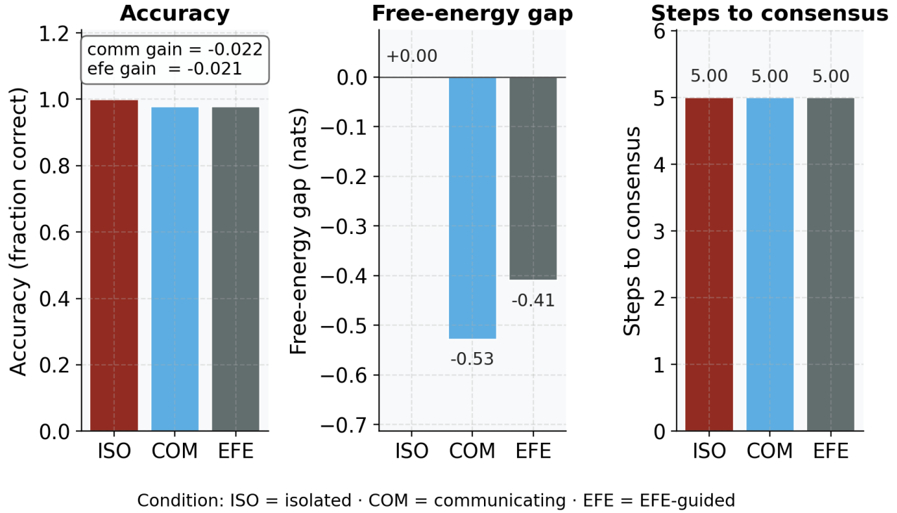
Figure 26: Moving sentinel world across isolated, communicating, and EFE-guided conditions. Source relation: original project schematic for the moving-world protocol; estimand: condition-level consensus accuracy, signed free-energy gap, and steps-to-consensus proxy in the stated native units; uncertainty: deterministic seeded run, so no resampling interval is shown. Moving sentinel world across the three conditions (x-axis is condition: isolated, communicating, EFE-guided). Left panel: y-axis shows consensus accuracy (fraction of 960 trials whose pooled argmax matches the truth). Center panel: y-axis shows the signed free-energy gap in nats (isolated surprise minus the condition's surprise on the true state, so a positive value would mean lower free energy than isolated; the measured gaps are negative, plotted against a zero reference line and annotated per bar). Right panel: y-axis shows a coarse steps-to-consensus proxy, with per-bar value annotations showing the three conditions are essentially tied. Each colony runs 6 steps over a 4-cell linear grid with 2 disjoint-FOV agents. No resampling interval applies to this deterministic seeded run. The finite reduced world does not establish a general communication benefit, an optimal movement policy, or source-protocol replication.
