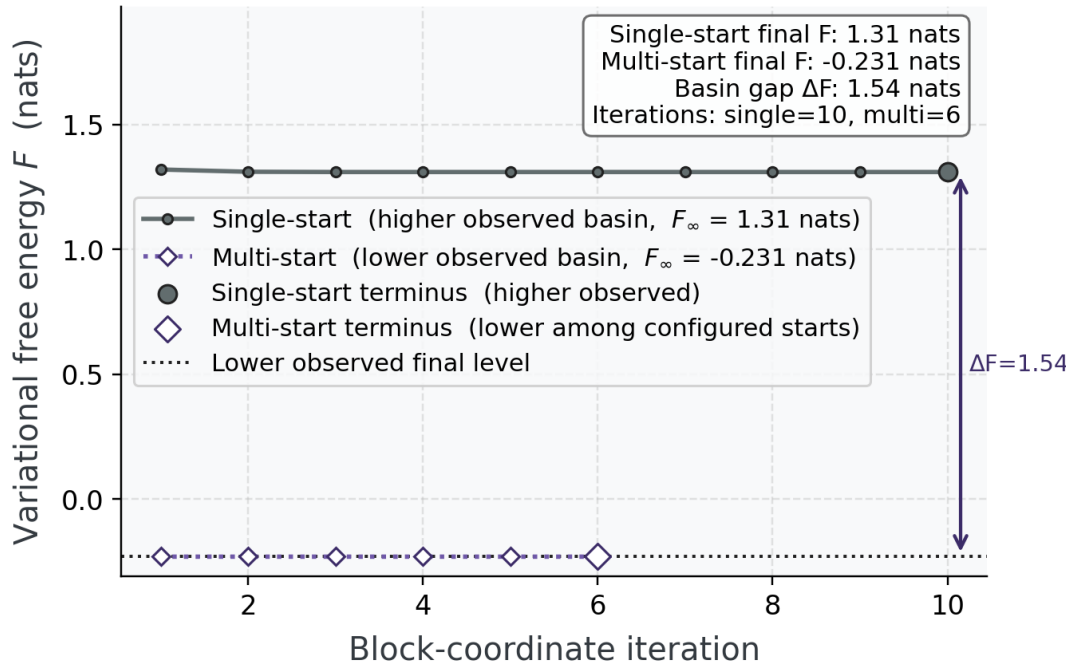
Figure 21: Variational free-energy descent on a near-vertex adversarial colony. Source relation: original project objective-descent diagnostic; estimand: objective value F in nats by block-coordinate iteration and configured initialization. The x-axis is iteration and the y-axis is F . A filled-circle solid path marks the single-start condition and an open-diamond dotted path marks the multistart condition; these neutral condition encodings do not imply different aggregation methods. Directly labeled terminal marks identify the higher and lower observed basins, a dark dotted rule marks the lower observed final level, and a double-ended annotation reports the terminal gap. The log-linear-pool single start settles at F = 1.3092 with retained saboteur weight, whereas the lowest trajectory among the configured alternatives reaches F = -0.2305 , a gap of 1.5397 nats. These are two deterministic traces from one configured colony, not independent stochastic replications, so no error bar, confidence interval, or resampling interval applies. Finite multistart descent does not certify a global optimum, enumerate every basin, or establish universal robustness.
