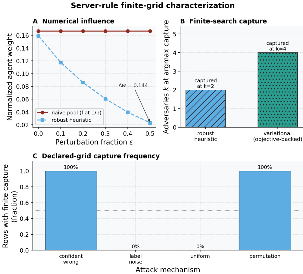
Figure 33: Three-panel empirical characterization of the server-side heuristic. Source relation: original project diagnostic of robust_aggregate ; estimands: numerical influence, finite-search capture count, and declared-grid capture fraction. In Panel A, the x-axis is the perturbation fraction moving one agent toward a confident-wrong belief and the y-axis is its converged normalized pooling weight. Circle-solid and square-dashed paths distinguish the naive pool and robust heuristic; a dark dotted rule marks 1/n , and a direct arrow label gives the terminal gap. In Panel B, the x-axis is aggregator and the y-axis is colluding-adversary count at consensus-argmax capture: k = 2 for the heuristic and k = 4 for the objective-backed variational rule. Forward and dotted hatches, dark keylines, method names, and direct captured at k labels duplicate color. Panel C’s x-axis is declared attack mechanism and its y-axis is the fraction of searched rows with finite capture inside the configured budget; direct percentages identify each bar. Units are normalized weight, adversary count, and finite-grid fraction. This is a deterministic finite grid with no population resampling; each declared seeded scenario row is a computational unit, not an exchangeable population replicate, so no confidence interval is shown. The grid fraction is neither a probability nor a global breakdown bound, and these settings do not establish bounded influence, Byzantine tolerance, or universal robustness.
