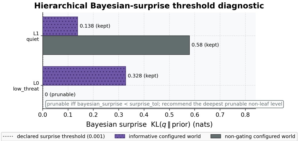
Figure 32: Per-level Bayesian surprise and configured threshold classifications for two hierarchical worlds. Source relation: original project information-gating diagnostic related to, but not an implementation of, the BMR mechanism in Friston et al. Fig. 9; estimand: per-level Bayesian surprise in nats and its thresholded prune/keep label; uncertainty: deterministic schematic worlds, so no resampling interval applies. The x-axis is Bayesian surprise KL(q \parallel \text{prior}) in nats, measuring information added by the leaf observation. The y-axis lists the non-leaf reduction targets top-down: level 0 is the meta-context (L3), level 1 is context (L2), and leaf location L1 is not reduced. Hatches, keylines, direct value-and-status labels, and vertical position distinguish the informative and non-gating worlds without color; the dark dotted rule is the declared classification threshold. The non-gating meta-context has 0.000 nats and is flagged prunable, leaving a two-level stack. The informative meta-context has 0.328 nats and is kept; both worlds keep context. The unit is nats for each configured world-level target, with no independent replication unit, sample size, confidence interval, or error band. Falling below the configured threshold is a sign-control outcome, not proof of structural redundancy. The figure does not report model evidence, posterior refitting, universal depth recovery, structure emergence, or exact source-protocol replication.
