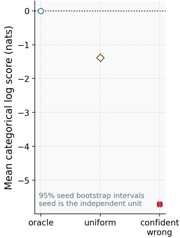
Figure 25: Proper-score and reliability controls. Source relation: original project belief-quality diagnostic; displayed estimands: categorical log score in nats and binned mean-confidence versus empirical-accuracy coordinates in fractions. The x-axis is control type in Panel A and mean confidence in Panel B; the y-axis is mean categorical log score and empirical accuracy, respectively. Open circles identify oracle controls, open diamonds identify uniform controls, and filled crosses identify confidently-wrong controls; the reliability panel retains the same marker-and-dash identities, direct endpoint labels, and a dark dotted perfect-calibration rule. Panel A's capped whiskers are 95% percentile-bootstrap intervals across independent configured seeds. Trials are nested within seed, and the reliability coordinates display no separate interval. Brier score and expected calibration error are retained as report-only secondary diagnostics and are not plotted in this two-panel figure. The ordered controls test score and reliability implementation on the configured finite world; they do not establish decision optimality, calibration under distribution shift, or robustness beyond the tested conditions.
