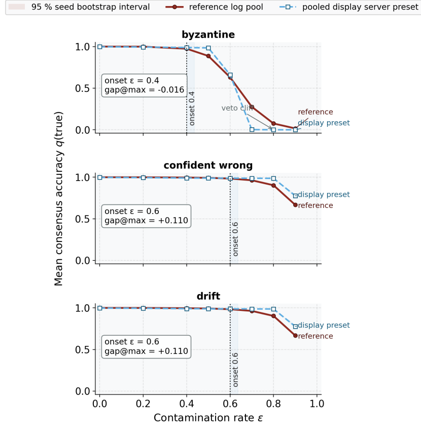
Figure 23: Reference log pool and pooled-selected server preset across attack rates. Source relation: original project robustness-onset diagnostic; estimand: mean consensus accuracy fraction by attack rate; uncertainty: shaded 95% percentile-bootstrap intervals over configured seeds, conditional on the pooled-selected display member. Each panel reads left to right as contamination increases: filled circles with a solid line identify the reference log pool, while open squares with a dashed line identify the pooled display server preset selected once by pooled mean across seeds at each rate. The x-axis is contamination rate and the y-axis is mean consensus accuracy. Each of 64 independent configured seeds contains 24 nested trials per rate; trials are not promoted to independent replicates. A dark dotted vertical rule marks the descriptive onset rate (pooled preset win fraction \geq 0.95 ), and the inset reports that onset plus the terminal preset-minus-reference gap. Confident-wrong and drift retain a displayed contrast after onset; Byzantine contamination produces a transient window before both methods lose consensus accuracy at the largest rates. The companion table gives the displayed onset, terminal values, and selected preset. This pooled-selection figure is descriptive, not selection-free post-selection inference; the all-method review grid supplies the selection-free comparative surface.
