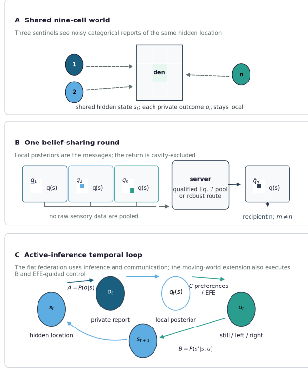
Figure 5: Sentinel-world and active-inference loop. Source relation: source-inspired original schematic related to Friston et al. (2024), Figs. 1 and 4; estimand: the implemented POMDP message-and-action sequence. Read Panels A–C from the shared hidden world, through one recipient-specific sharing round, to the temporal loop. The x-axis is the Panel C sequence from hidden state through private observation, local posterior, action, and next state; the y-axis separates world, federation, and temporal stages. Panel A shows three agents receiving private noisy outcomes from one 9-cell hidden world. Dashed sensing connectors distinguish those private observation relations from the shared state. Panel B sends only local posteriors along solid arrows to the qualified Eq. 7 pool or robust route and returns a cavity-excluded posterior; its dashed recipient connector marks the m \neq n exclusion qualification. Panel C uses solid directed arrows for likelihood update, posterior formation, EFE-guided action, and transition, with direct A , B , and C labels. The flat studies execute inference and sharing; the moving-world extension additionally executes transition and control. Units are categorical states, outcomes, posterior messages, actions, and ordered steps. This deterministic schematic has no fitted effect, replication unit, error band, or confidence interval; it does not demonstrate a complete source protocol, physical multi-host federation, Byzantine tolerance, privacy mechanism, or universally beneficial communication policy.
