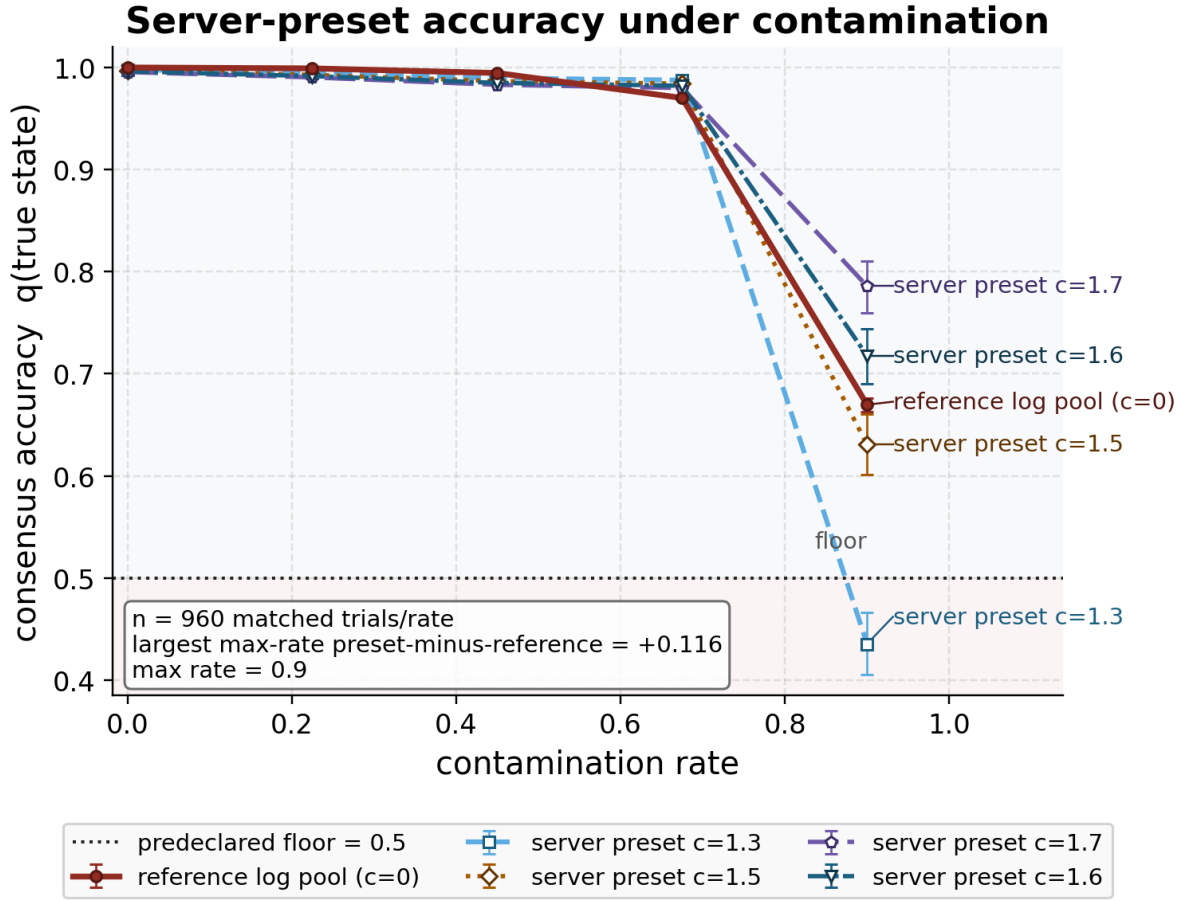
Figure 13: Consensus accuracy: probability mass assigned to the true hidden state. The plotted estimand is q(\text{true state}) . Source relation: original project robustness extension; estimand: true-state probability mass; uncertainty: matched-trial percentile-bootstrap intervals over configured trials. The x-axis is saboteur convex-mix contamination rate over \{0, 0.225, 0.45, 0.675, 0.9\} ; the y-axis is consensus probability mass on the true state. Curves compare the standard KLD log-linear pool with robust_aggregate server presets KLD(c = 0.00) , RKL(c = 1.50) , AR(c = 1.30) , beta(c = 1.70) , rcce(c = 1.60) for 7 agents, including 2 saboteurs; they are not named client losses. Distinct markers, dashes, direct labels, and the dark dotted threshold at 0.50 duplicate color. The independent replication unit is a matched synthetic trial within the fixed seeded true state and attack target, with 960 trials per rate. Curves show trial means with 95% percentile-bootstrap confidence intervals. At the largest rate, the standard pool reaches 0.6697 and the within-sweep highest pooled robust mean reaches 0.7857 . That operating point is a disclosed display selection: low-rate robust means can match or trail the standard pool, and individual presets can fall below the threshold. The truncated linear y-axis enlarges the declared threshold region. This fixed-world sweep does not establish a universal method ranking, alternate-world generalization, a client-loss theorem, bounded influence, or Byzantine tolerance; the selection-free seed-level review is reported separately.
