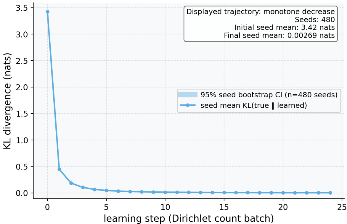
Figure 11: Seed-mean KL divergence from the true likelihood A to the learned likelihood A . The plotted quantity is KL(\text{true } A \parallel \text{learned } A) . Source relation: source-mechanism analogue to Friston et al. (2024), Fig. 7; estimand: seed-mean KL in nats by ordered learning step. The x-axis is the ordered Dirichlet count batch, from the flat prior at zero through all 24 batches (25 points per seed); the y-axis is summed per-column KL divergence between the true likelihood and the current expected likelihood, in nats. The solid line is the mean over 480 independent configured seeds, and the shaded band is the pointwise 95% percentile-bootstrap interval resampling seeds at each learning step. The replication unit is seed, not the ordered trajectory points. The mean curve falls monotonically from 3.4231 nats to 0.0027 nats (total reduction 3.4204 nats, computed from the unrounded endpoints); the computed monotone-decreasing check is Yes. This reduced categorical protocol is related to, but does not exactly reproduce, the richer multi-episode protocol in Friston et al. (2024).
