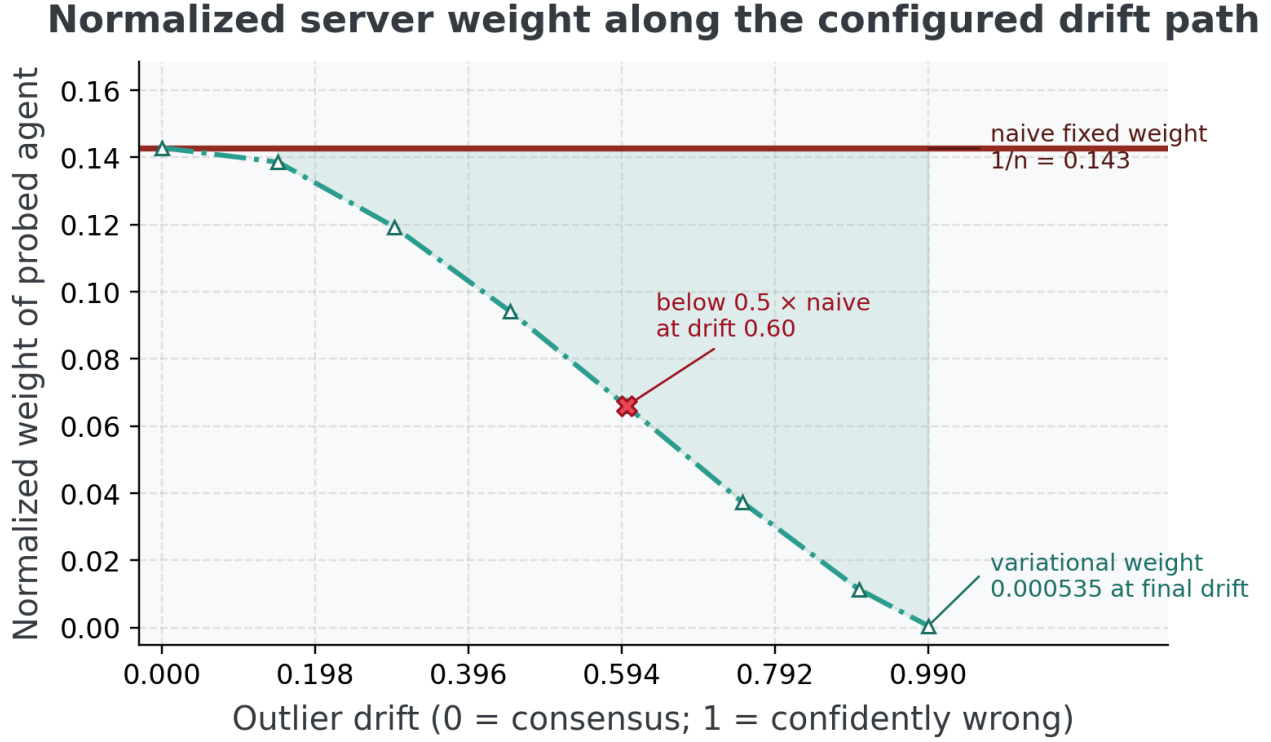
Figure 17: Normalized influence weight of one probed agent. Source relation: original project variational-server diagnostic; estimand: the probed agent’s normalized server weight as its posterior drifts toward a confident-wrong delta. The x-axis is outlier drift from consensus at zero to the wrong-state delta at one; the y-axis is normalized influence weight. The open-triangle dash-dot path is variational_aggregate ; the circle-solid horizontal reference is the naive log-linear pool. Direct endpoint labels name both rules and values, shaded separation shows their tested-path gap, and an adversarial X with an arrow marks the first displayed point below one-half of the naive weight. As drift becomes extreme, the variational weight falls below 0.001, whereas the naive pool remains fixed at 1/n = 0.143 . This deterministic seeded sweep contains n = 7 agents in one configured colony; drift points are ordered evaluations, not independent replications, so no confidence interval or error band applies. The pattern is redescending normalized weight along this path, while the algebraic property bounds raw effective weight; the figure is not an estimator-level B-robustness proof and does not transfer the property to the sharper robust_aggregate heuristic.
