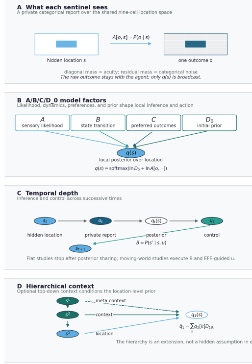
Figure 4: Formal categorical generative-model schema. Source relation: source-inspired original schematic related to Friston et al. (2024), Figs. 1 and 4; estimand: the categorical dependency structure implemented by the applicable studies. Read Panels A–D from private sensing, through local factors, to temporal depth and optional hierarchy. The x-axis is dependency or role order within each panel; the y-axis positions hidden states, observations, model factors, and context levels. Panel A maps a hidden 9-cell location through A[o, s] to one private categorical outcome. Panel B shows likelihood A , transition B , preference C , and initial prior D_0 feeding the local posterior q(s) . Panel C orders state, observation, posterior, action, and next state; Panel D shows conditioned lower-level priors. Solid arrows encode implemented categorical dependencies used by the applicable flat, moving-world, or hierarchical studies; the dashed upper-context edge marks a qualified optional extension. Direct factor and node labels, arrow direction, edge style, and panel order duplicate color. Units are categorical states, outcomes, factors, messages, and ordered steps. This deterministic formal schematic has no fitted value, empirical sample, replication unit, error band, or confidence interval; it does not claim that every source-model component, continuous state, learning rule, or complete multi-agent protocol has been reconstructed.
