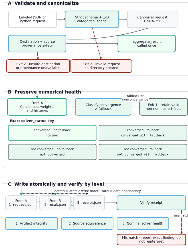
Figure 19: The labeled application path separates fail-closed request and destination checks from retained non-nominal results. Source relation: source-owned labeled-aggregation, solver-health, artifact, and receipt contracts; status: deterministic implementation map, not an experiment. Panel A follows labeled JSON or Python input through strict schema and one-dimensional shape validation, canonical semantic hashing, a destination-and-required-provenance safety gate, and one delegation to the shared aggregation result. Its two dashed rejection branches distinguish an invalid request from an unsafe destination or unavailable required provenance; both exit 2 before directory creation. Panel B classifies convergence and fallback state, then gives the exact two-by-two solver_status key: nominal , converged_with_fallback , not_converged , and not_converged_with_fallback . Panel C carries the canonical request and rich result into request.json and result.json , binds both into receipt.json , and enters verification. Solid arrows encode data dependency; the dotted sequence records atomic write order; dashed paths mark rejection or a retained warning. The x-axis is left-to-right execution within rows; rows order panels and verification levels. The estimand is validation, artifact, and solver state; the unit is one categorical software state per invocation. No sampling uncertainty or independent replication unit applies. Exit 1 retains non-nominal artifacts, and a mismatch reports its exact finding. Receipt integrity, source equivalence, and nominal health do not establish calibration, domain suitability, scientific validity, downstream decision correctness, or acceptance.
