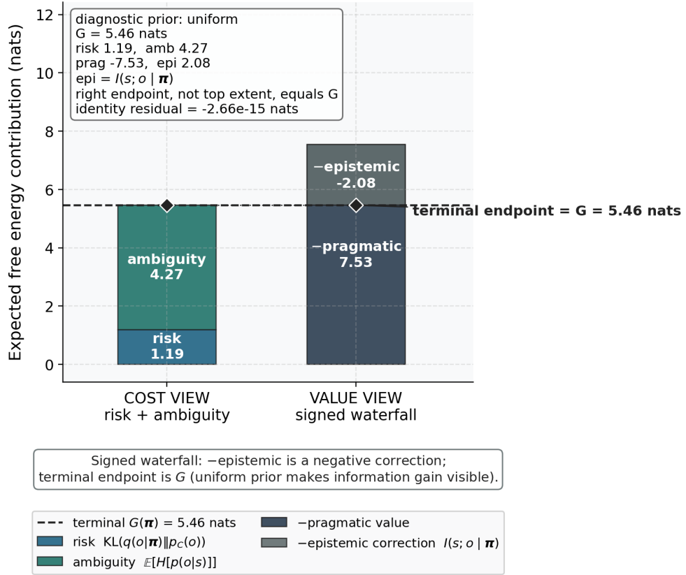
Figure 8: Expected-free-energy decomposition for the categorical generative model (expected_free_energy.py). Source relation: formal specialization of Friston et al. (2024), Eq. 2; estimand: categorical EFE identity in nats. x-axis: two views of the same identity (left, additive cost view: risk + ambiguity; right, signed value waterfall: positive minus-pragmatic contribution followed by a negative epistemic correction). y-axis: EFE contribution in nats. The heavy endpoint marker and connector, rather than the intermediate top extent, identify the terminal G(\pi) value. The epistemic term is state-outcome mutual information I(s; o | \pi) ; it is visible because the diagnostic prior is uniform, whereas the canonical point-mass D_0 is the corresponding zero-information null. The finite terms satisfy the identity at machine precision. This deterministic algebraic check has no error bars or independent sample size, and it does not reproduce every parameter-learning term in the source equation.
