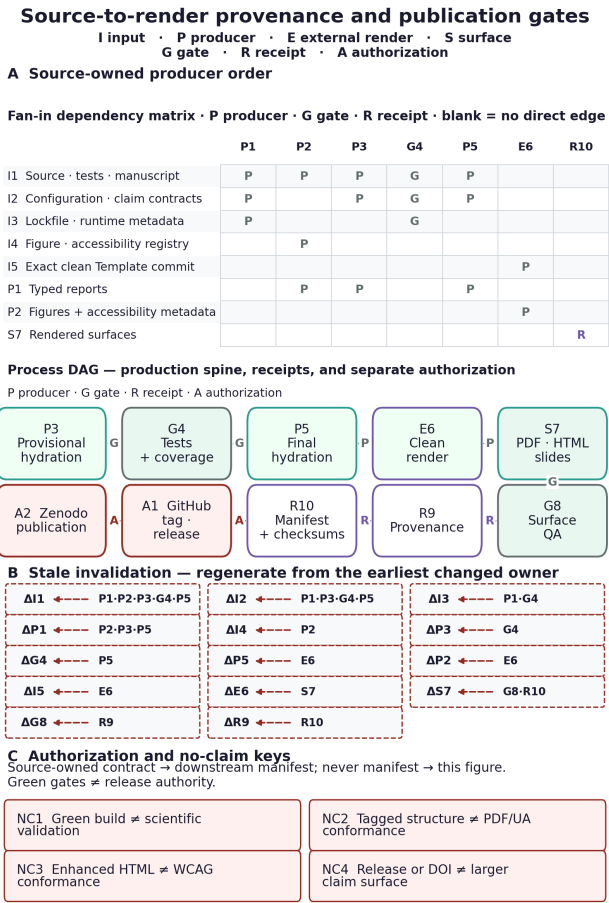
Figure 20: Publication surfaces inherit source state; green gates remain distinct from release authority. Source relation: source-owned explanatory producer and invalidation contract; study status: deterministic provenance map, not an empirical result. Read Panel A first across the dependency matrix and then through the two-band process path. The matrix x-axis indexes seven downstream targets, while its rows name five inputs and three upstream producers; each populated cell carries a producer, gate, or receipt code. The adjacent crossing-free path orders provisional hydration, tests and coverage, final hydration, exact clean Template rendering, reader surfaces, surface checks, provenance, manifests, and the separately authorized GitHub and Zenodo terminals. Panel B groups fourteen changed owners into dashed reverse-dependency cards; each arrow points from immediate stale targets back to its changed owner. Panel C states the non-circular manifest boundary and four no-claim rules. Codes, direct labels, keylines, solid producer or receipt arrows, dashed gate arrows, and dashed reverse arrows duplicate color. The estimand is categorical dependency and authorization state; the unit is one pipeline or publication stage. There is no sampling uncertainty, sample size, or replication unit. The figure never reads the downstream manifest. A green build does not authorize publication, establish scientific validity, PDF/UA or WCAG conformance, or enlarge the claim surface through a release or DOI.
