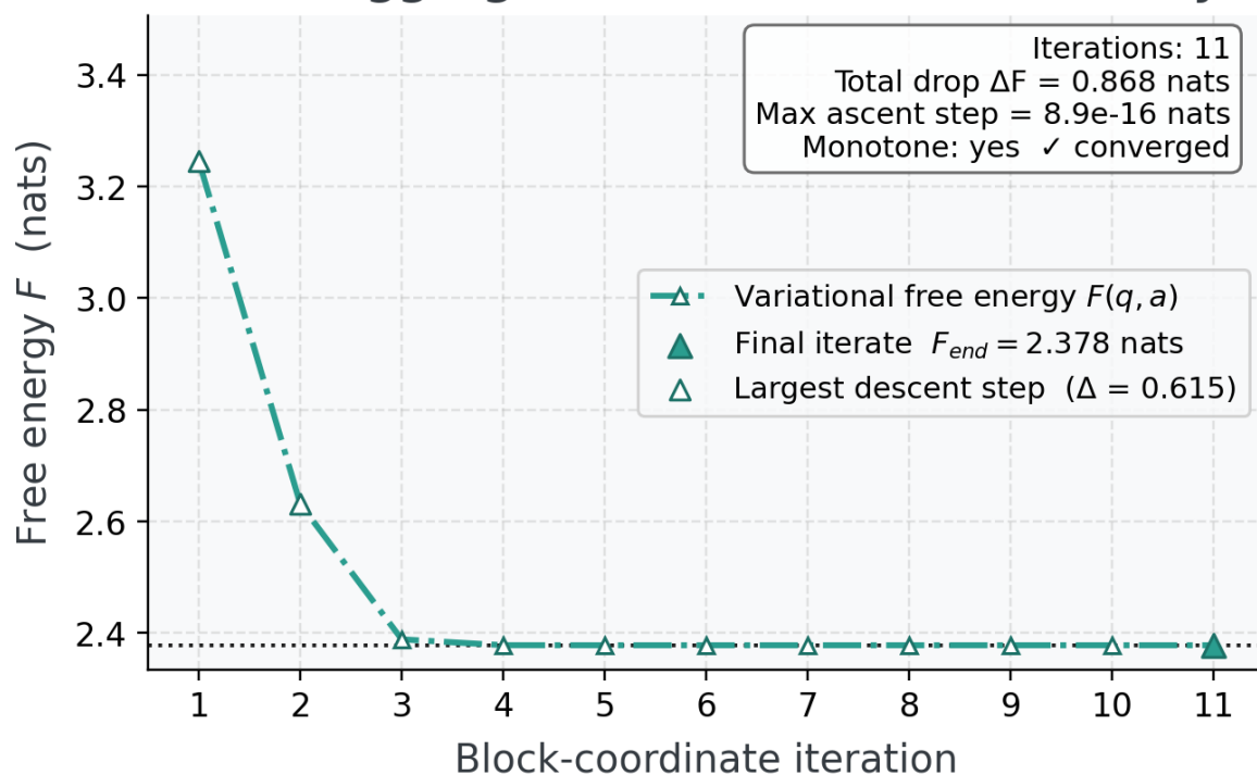
Figure 16: Variational free energy F(q, a) as a function of block-coordinate descent iteration. Source relation: original project objective-descent diagnostic; estimand: free energy in nats by iteration; uncertainty: none for the deterministic seeded run. The trace is a single variational_aggregate fusion of a 7-agent contaminated colony (robustness 1.50). The x-axis is block-coordinate iteration number and the y-axis is F(q, a) in nats. Open triangles joined by a dash-dot path identify the variational trajectory, a filled triangle marks the terminal iterate, enlarged open triangles mark the endpoints of the largest observed descent step, and a dark dotted horizontal rule marks the final stationary level; these shapes and line patterns duplicate color. The curve is monotone non-increasing across all recorded iterations (largest single-step increase: 8.88 \times 10^{-16} nats, at machine precision), and the implementation reports converged status Yes at F = 2.3780 nats. Iterations are ordered states of one deterministic run, not independent replicates, so no resampling interval applies. This trace verifies descent only for the executed path; it does not certify a global optimum, exhaustive basin search, or the separate robust_aggregate heuristic.
