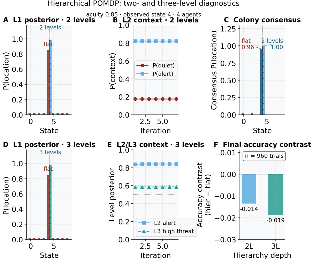
Figure 28: Six-panel hierarchical POMDP belief-dynamics and accuracy diagnostic. Source relation: source-inspired original project diagnostic for a hierarchical extension; estimand: posterior probabilities and final hierarchical-minus-flat location-accuracy gap in the declared seeded protocol. Read the two-level world across the top row and the three-level extension across the bottom. In the left column, the x-axis indexes 9 location states and the y-axis is posterior probability after one center-cell observation; plain left-offset bars are the flat-prior reference and forward-hatched right-offset bars are hierarchical. In the middle column, the x-axis is alternating-minimization iteration and the y-axis is context probability; circles, squares, triangles, and solid or dashed paths identify the displayed levels without color. The top-right panel uses the same plain-versus-hatched bar grammar for L1 consensus after federating 4 agents, with direct peak labels. The bottom-right panel's x-axis is hierarchy depth and its y-axis is the final accuracy-fraction contrast over 960 nested trials, with direct signed values and a zero rule. Units are probability or accuracy fraction. Seed 0 defines one deterministic protocol realization; ordered states, iterations, agents, and trials are nested measurements rather than independent resampling units, so no interval or error band applies. The figure does not establish universal hierarchical benefit, calibrated uncertainty, or source-protocol replication.
