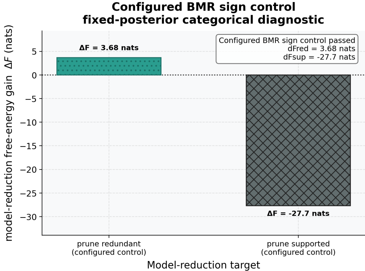
Figure 12: Configured Bayesian-model-reduction sign control. Source relation: source-mechanism analogue to the model-reduction mechanism in Friston et al. (2024), Fig. 9; estimand: BMR \Delta F in nats for two declared pruning candidates. The x-axis is candidate likelihood-column pruning, ordered as the redundant column and supported-column control; the y-axis is \Delta F , where positive values favor the reduced model and negative values reject it. Dotted hatching and a dark teal keyline identify the favored redundant-column control, while cross-hatching and a dark neutral keyline identify rejected supported-column pruning; direct signed value labels and a dark dotted zero rule duplicate color. On the fixed posterior, redundant-column pruning gives \Delta F = 3.68 and supported-column pruning gives \Delta F = -27.67 , so the configured sign control passes (Yes). This is one deterministic closed-form comparison with no independent replication unit, resampling interval, confidence interval, or error bar. The configured signs do not establish universal structure emergence, consistent recovery of true structure, or exact reproduction of the source simulation.
