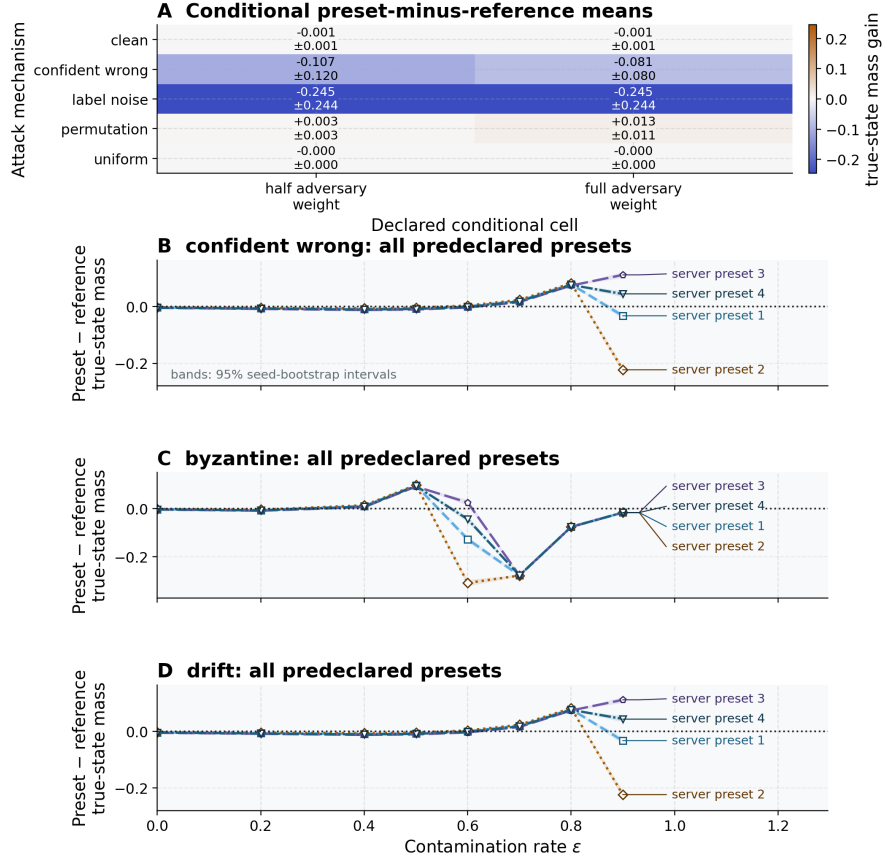
Figure 14: The robustness review retains every server preset and preserves mixed signs across the attack grid. Source relation: original project conditional simulation review joining registered conditional-world and directional-rate reports; study status: selection-free, all-method finite-grid evidence; estimand: seed-level robust-minus-standard true-state probability-mass contrast. Read the portrait figure from top to bottom: Panel A is a full-width heatmap of conditional attack cells by adversarial-weight setting; Panels B–D stack confident-wrong, Byzantine, and drift rate profiles. The x-axis is adversarial weight in Panel A and contamination rate in Panels B–D; the y-axis is contrast in probability units. Printed cell signs, distinct markers and dashes, and elbow leaders into reserved right-side endpoint-label lanes duplicate color; the dark dotted rule marks zero. The independent replication unit is the configured seed ( n = 160 ), with 24 trials plus agents and conditions nested within each cell. Rate-profile bands are 95% percentile-bootstrap intervals over seeds. The second heatmap line is half the finite-grid min–max span, not a confidence interval. No curve is selected by pooled mean. The figure supports only mechanism- and grid-conditional contrasts; it does not establish a universal winner, bounded influence, Byzantine tolerance, a causal effect, independent shared-design cells, or generalization beyond the registered worlds.
