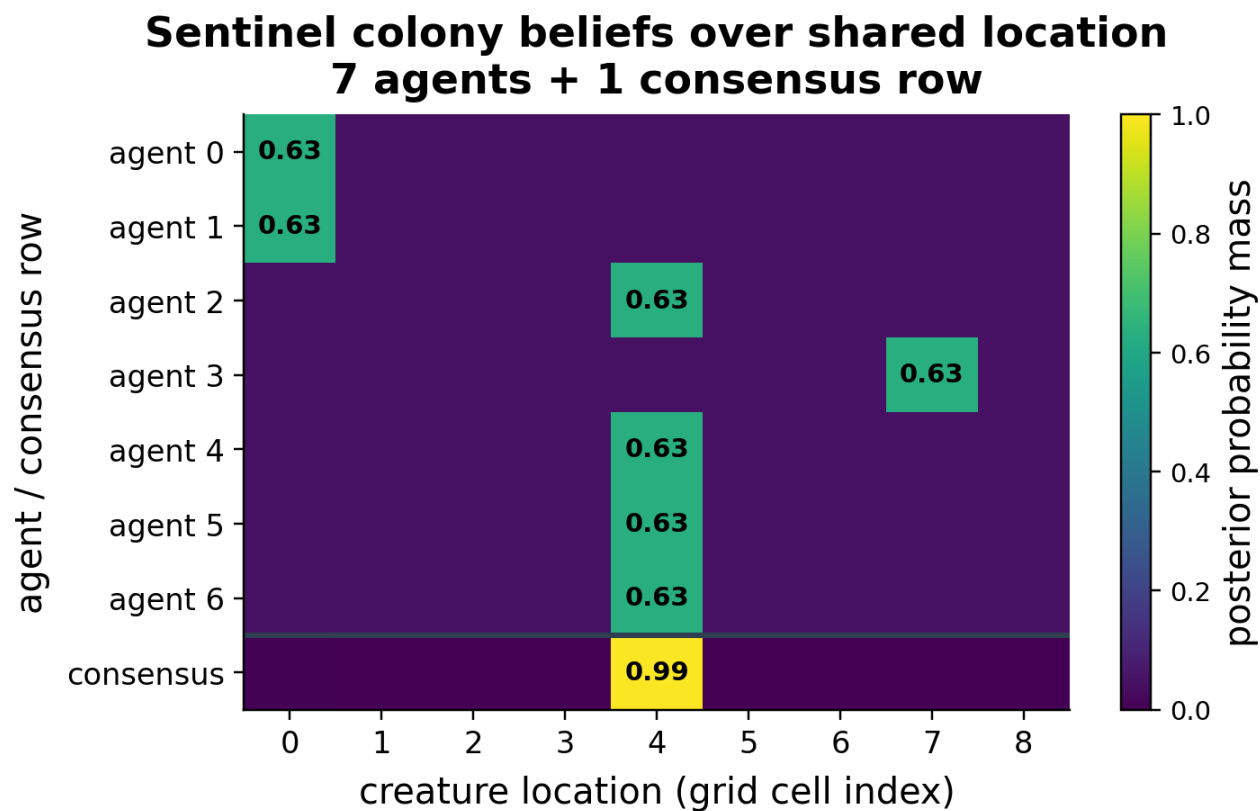
Figure 10: Single-panel belief heatmap over the hidden creature location. Source relation: original project diagnostic supporting the Study 1 analogue; estimand: posterior probability mass by hidden state; uncertainty: deterministic single-seed display. The hidden creature location (7 sentinels, acuity 0.55, seed 0). x-axis: hidden-state grid cell (creature location, 9 cells); rows: the 7 individual agents' private posteriors (one row per agent, dominant cell annotated), plus a bottom consensus row — separated by the divider line — holding the federated consensus fused from those posteriors by the cavity-exclusion round defined in the methods. Each private posterior concentrates only moderately on the cell its noisy observation suggests; the consensus row concentrates more sharply on the true location. All cell values are deterministic posterior probabilities for the single displayed seed, so no error band applies. This mechanism display does not establish calibration, a general communication benefit, or exact source-protocol replication.
