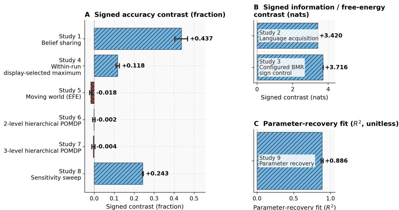
Figure 30: Native-unit cross-study summary of the headline signed contrasts. Source relation: original-project synthesis from a separate harmonized seed-level rerun; status: conditional overview, not a pooled meta-analysis. Panel A, read down the left column, shows six signed accuracy contrasts in fractions. Panel B at upper right shows two information or free-energy contrasts in nats. Panel C at lower right shows one parameter-recovery fit in unitless R^2 . Each x-axis reports the signed study-level mean in its panel's native unit; each y-axis lists only that panel's studies. Horizontal bars are means, whiskers are 95% percentile-bootstrap intervals, and direct signed labels give the means. Forward, cross, and dotted hatches distinguish positive, negative, and near-zero estimands; the dark dotted rule marks zero without color. The independent and resampling unit is the seed ( n = 128 ) within each configured study, with observations, agents, trials, and ordered steps nested. These intervals belong only to the harmonized rerun, including rows whose primary figure is a deterministic single-posterior diagnostic; they do not retrofit uncertainty to those primary figures. The Study 4 row is the within-run display-selected maximum across non-reference server presets at the declared worst rate, neither a preselected method nor an inferential winner. Native units are preserved: the figure neither ranks nor pools studies nor implies a shared effect or universal benefit.
