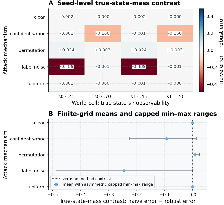
Figure 24: Conditional-world robustness grid. Source relation: original project finite-grid generalization of the MAJ-1 characterization; estimand: naive true-state error minus robust true-state error in probability-mass units. In Panel A, the x-axis indexes hidden-state and observability cells and the y-axis indexes attack mechanisms; every heatmap cell prints its signed seed-level mean, so sign and magnitude remain available without colour. The source report retains a 95% seed-bootstrap interval for each cell. In Panel B, the x-axis is the signed contrast and the y-axis again lists attacks. Its point is the mean over all declared finite-grid cells for that attack, and the asymmetric capped whiskers extend to the observed cell minimum and maximum. These capped min/max spans are finite-grid ranges, not confidence intervals and not symmetric mean-plus-or-minus errors. A dark-neutral dotted zero rule marks no method contrast. Positive values favour robust true-state mass; negative values favour naive pooling. The independent unit is the seeded world/scenario row, with 24 trials nested within each row. This is conditional evidence over a declared finite grid, not a theorem, breakdown bound, universal attack result, or estimate of performance beyond the registered worlds.
