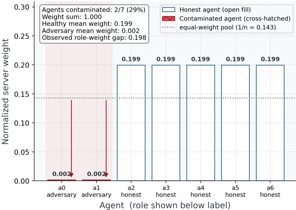
Normalized heuristic server weights by declared agent role
