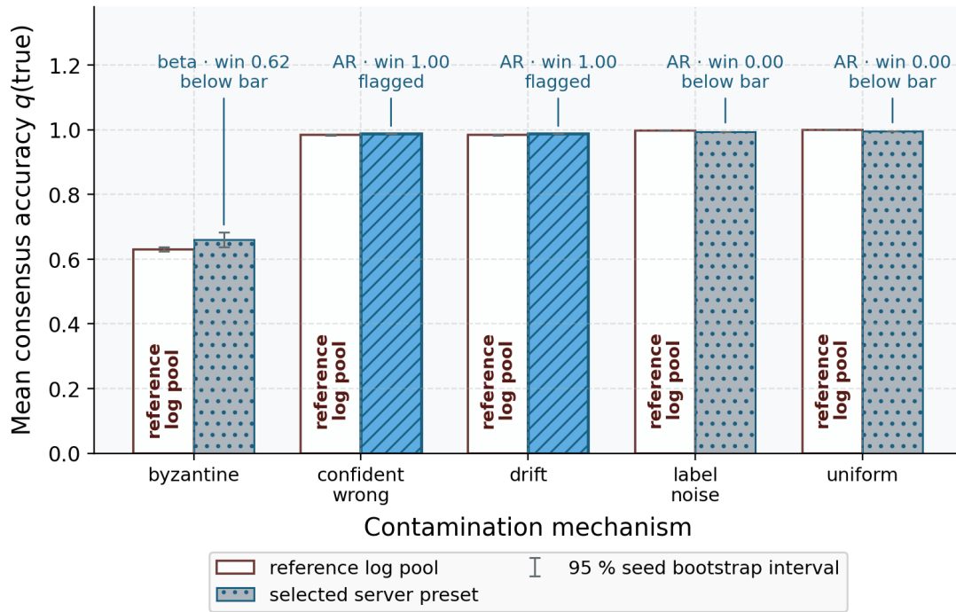
Figure 22: Seed-aggregated mean consensus accuracy. Source relation: original project contamination diagnostic; estimand: true-state accuracy fraction by attack mechanism; uncertainty: the bars show 95% seed-level bootstrap confidence intervals for the pooled-selected display member, while the adjacent table reports its conditional paired difference interval. q(\text{true state}) for the reference log-linear pool versus the server preset selected once by pooled mean under each contamination mechanism ( n = 24 \text{ trials} \times 64 \text{ seeds} at strength 0.60). The x-axis is the contamination mechanism; the y-axis is mean consensus accuracy. Each group has two bars: an open, directly labeled reference-log-pool bar and a hatched selected-server-preset bar whose direct annotation names the preset and its across-seed win fraction. The preset bar is drawn in full color only where that win fraction clears the 0.95 display bar — confident wrong, drift; the byzantine mechanism and entropy attacks are muted because they do not clear that descriptive screen. The in-figure summary gives the display-flag count across mechanisms and reminds readers that the labels are win fractions, not p-values. Bars are means over 64 independent configured seeds, with 24 matched trials nested within each seed. This is a descriptive pooled-selection graphic, not selection-free post-selection inference; the all-method review grid supplies the latter surface.
