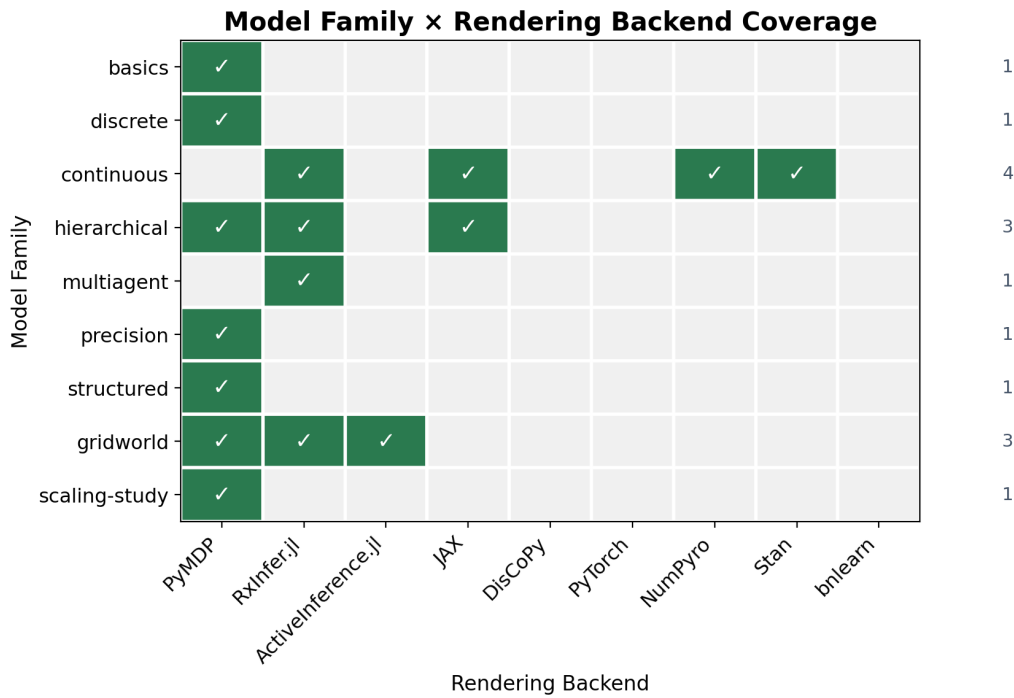
Figure 6: Model-family coverage across the registered rendering backends: one row per family from input/model_family_manifest.json , one column per backend from src/gnn/render/framework_registry.py , and a green cell wherever the family declares that backend in its frameworks field. The right-hand count states how many backends each family declares; the grid is deliberately sparse — most families declare a single backend, and only continuous, hierarchical, and gridworld declare several. Read it as declared intent, not as profiled outcomes: the gates described below supply the outcomes. The matrix is generated from the two registries at commit a28701d0c.
