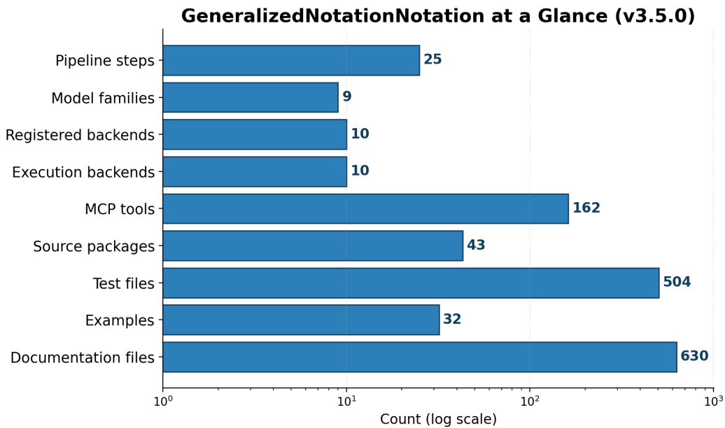
Figure 7: Repository-scale counts on a logarithmic axis: pipeline steps, model families, registered backends, execution backends, Model Context Protocol tools, source packages, test files, example models, and documentation files. Every bar is annotated with its exact value, and every value is a producer token read from output/data/manuscript_variables.json at commit 13141e9f7 — the same token map that substitutes the prose counts, so the figure cannot disagree with the text without failing the figure-freshness suite. The two backend bars are deliberately distinct: registered backends (10) counts render targets, execution backends (10) counts the subset that runs at Step 12. Read the chart as the scale of the surface the pipeline maintains, not as a quality measure.
