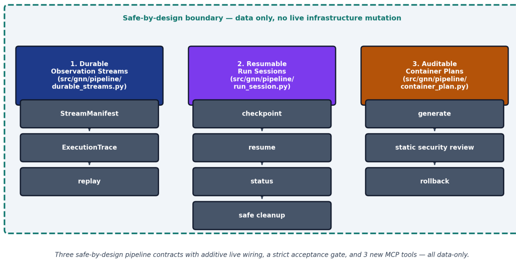
Figure 4: The GNN 3.0.0 long-running orchestration contracts: durable observation streams, resumable run sessions, and auditable container plans.
