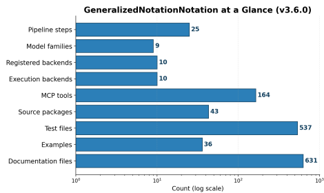
Figure 2: Repository-scale counts on a logarithmic axis: pipeline steps, model families, registered backends, execution backends, Model Context Protocol tools, source packages, test files, example models, and documentation files. Every bar is annotated with its exact value, and every value is a producer token read from output/data/manuscript_variables.json at commit 459287940 — the same token map that substitutes the prose counts, so the figure cannot disagree with the text without failing the figure-freshness suite. The two backend bars are deliberately distinct: registered backends (10) counts render targets, execution backends (10) counts the subset that runs at Step 12. Read the chart as the scale of the surface the pipeline maintains, not as a quality measure.
