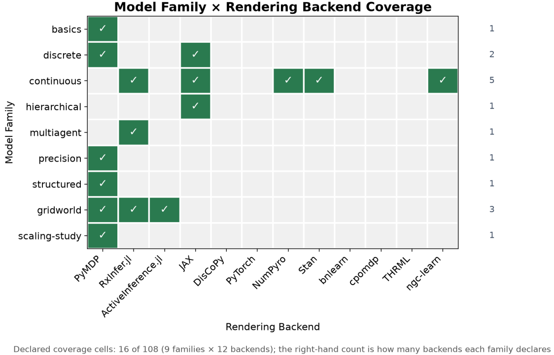
Figure 6: Model-family coverage across the registered rendering backends: one row per family from input/model_family_manifest.json , one column per backend from src/gnn/render/framework_registry.py , and a green cell wherever the family declares that backend in its frameworks field. The right-hand count states how many backends each family declares; the grid is deliberately sparse — most families declare a single backend, and only continuous, discrete, and gridworld declare several. Read it as declared intent, not as profiled outcomes: the gates described below supply the outcomes. The matrix is generated from the two registries at commit b99695547.
