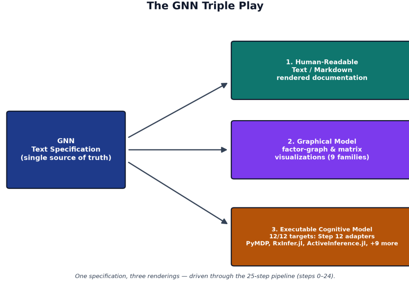
Figure 3: The Triple Play: one GNN text specification (left) and its three coordinated projections (right) — the human-readable text form, graphical model visualizations, and executable simulation code. All three arrows originate at the same source box to show their shared parsed input. Source binding, parameter validation, and semantic-fidelity checks provide evidence of agreement among the projections. The executable node summarizes 12 of 12 registered render targets with implemented Step 12 execution adapters and previews three by name; execution depends on runtime readiness, admitted model kind, and a successful source-bound run receipt. Counts are producer tokens at commit b99695547, and the panel is generated by scripts/manuscript_fig_triple_play.py . Take-away: a model is authored once and then read, seen, and run from that single source.
