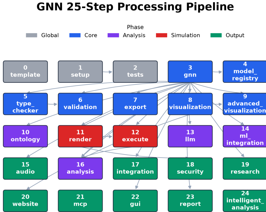
25 steps (0–24) · 25 required step prerequisites · rowwise topological order; colored by execution phase
