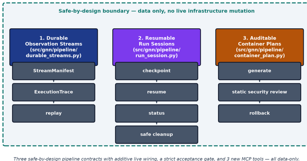
Figure 5: The three safe-by-design orchestration contracts introduced in GNN 3.0.0, side by side inside the dashed boundary that states their shared invariant: generate and validate data only, never mutate live infrastructure. Each column names the contract’s source module under src/gnn/pipeline/ and chains its stages top to bottom — StreamManifest, ExecutionTrace, and replay for durable observation streams; checkpoint, resume, status, and safe cleanup for resumable run sessions; generate, static security review, and rollback for container plans. Arrows give the order the stages run in, and nothing exits the boundary. The panel is a fixed-layout drawing of the three contracts; the acceptance gates and the Model Context Protocol tools that exercise them are described in the text above. Take-away: long-running orchestration gains capability only as fast as it becomes inspectable.
