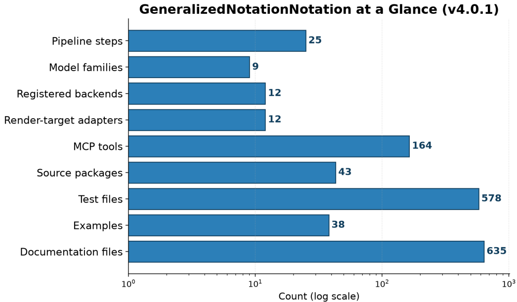
Figure 7: Repository-scale counts on a logarithmic axis: pipeline steps, model families, registered backends, render-target execution adapters, Model Context Protocol tools, source packages, test files, example models, and documentation files. Every bar is annotated with its exact value, and every value is a producer token read from output/data/manuscript_variables.json at commit b99695547 — the same token map that substitutes the prose counts. The figure-freshness suite binds the committed image digest and its recorded producer inputs and counts; semantic content and visual correctness require their own review. The two backend bars are deliberately distinct: registered backends (12) counts render targets, render-target adapters (12) counts the render-target subset with implemented Step 12 execution adapters. It excludes the separate execution-only Lean bridge and is not a count of observed native runs. Read the chart as the scale of the surface the pipeline maintains, not as a quality measure.
