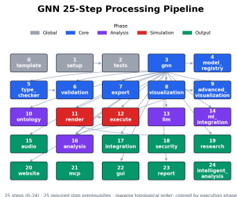
Figure 1: The 25-step GNN processing pipeline as a directed acyclic graph, arranged in rowwise topological order and colored by execution phase (legend above the nodes). Each node is the thin step orchestrator under src/gnn/ named in tbl. 2; each arrow is a required orchestration prerequisite parsed from the Data Dependency Graph block of src/gnn/STEP_INDEX.md , which mirrors the live step registry. Parsing (Step 3) precedes many later steps. Optional artifact enrichments are documented separately and are not shown as required edges. The figure is generated from src/gnn/STEP_INDEX.md at commit a57e17d86 ; its footer restates the step count, the number of required prerequisites, and the layout rule.
