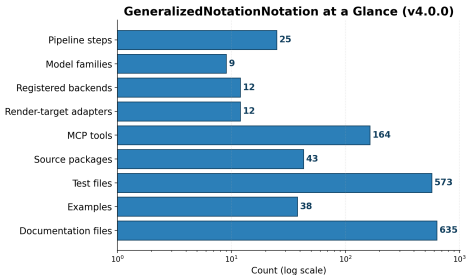
Figure 2: Repository-scale counts on a logarithmic axis: pipeline steps, model families, registered backends, render-target execution adapters, Model Context Protocol tools, source packages, test files, example models, and documentation files. Every bar is annotated with its exact value, and every value is a producer token read from out/put/data/manuscript_variables.json at commit 8d202439e — the same token map that substitutes the prose counts. The figure-freshness suite binds the committed image digest and its recorded producer inputs and counts; semantic content and visual correctness require their own review. The two backend bars are deliberately distinct: registered backends (12) counts render targets, render-target adapters (12) counts the render-target subset with implemented Step 12 execution adapters. It excludes the separate execution-only Lean bridge and is not a count of observed native runs. Read the chart as the scale of the surface the pipeline maintains, not as a quality measure.
