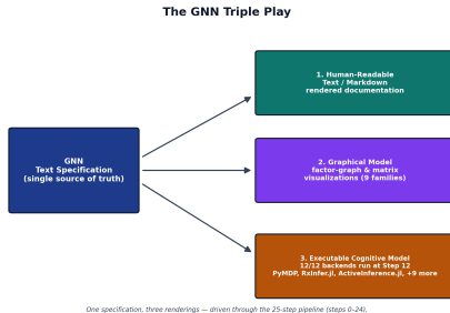
Figure 2: The Triple Play: one GNN text specification (left) and its three coordinated projections (right) — the human-readable text form, graphical model visualizations, and executable simulation code. All three arrows originate at the same source box because all three projections are generated from one parsed document, which is why they cannot drift apart; the executable node states that 12 of 12 registered backends run at Step 12 and previews three of them by name. Counts are producer tokens at commit 399a3618b, and the panel is generated by scripts/manuscript_fig_triple_play.py . Take-away: a model is authored once and then read, seen, and run from that single source.
