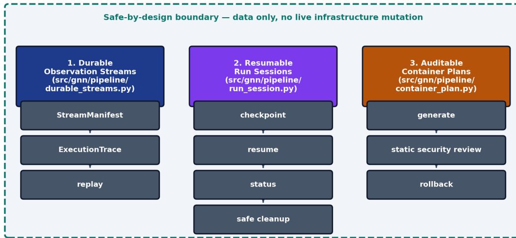
Three safe-by-design pipeline contracts with additive live wiring, a strict acceptance gate, and 3 new MCP tools — all data-only.
