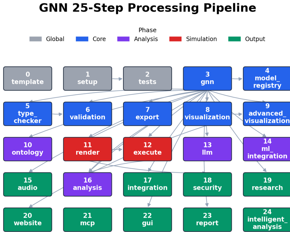
25 steps (0–24) · 25 required step prerequisites · rowwise topological order; colored by execution phase
