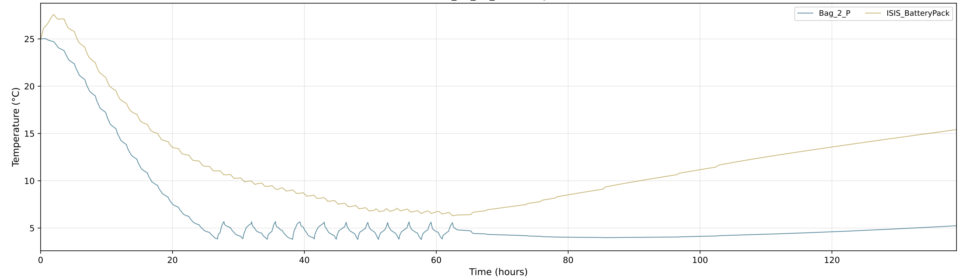
Acubesat_10_12_25 - Temperatures
