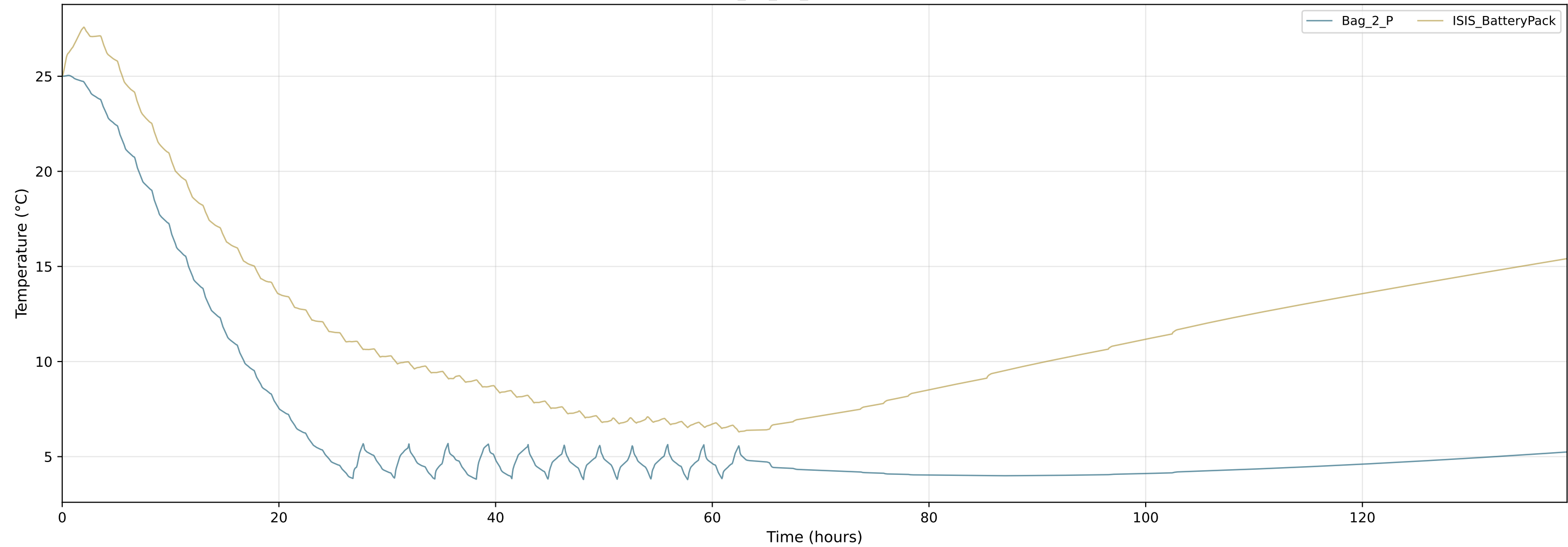
Acubesat_10_12_25 - Temperatures
