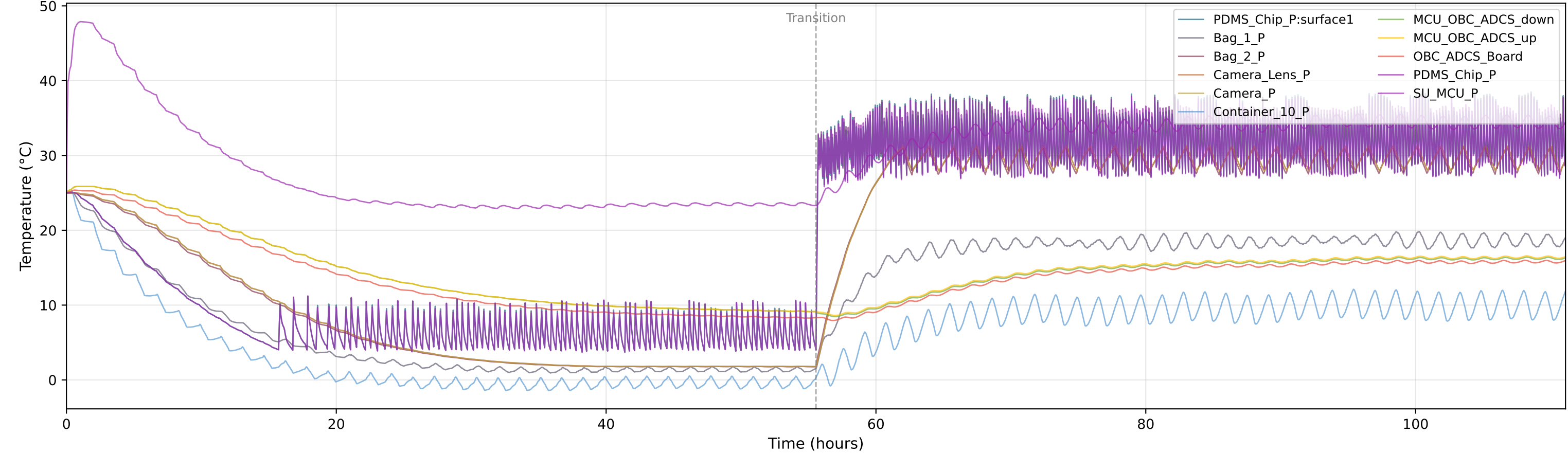
Acubesat_7_12_25 - Temperatures (Sequential)
