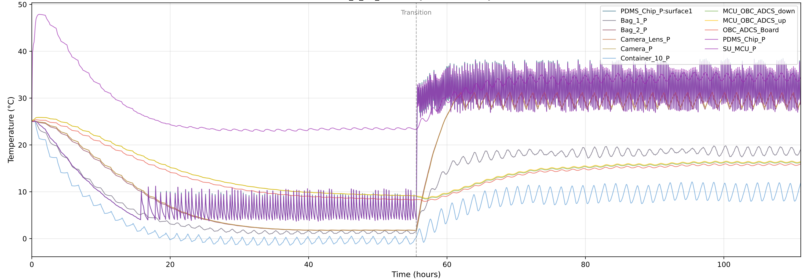
Acubesat_7_12_25 - Temperatures (Sequential)
