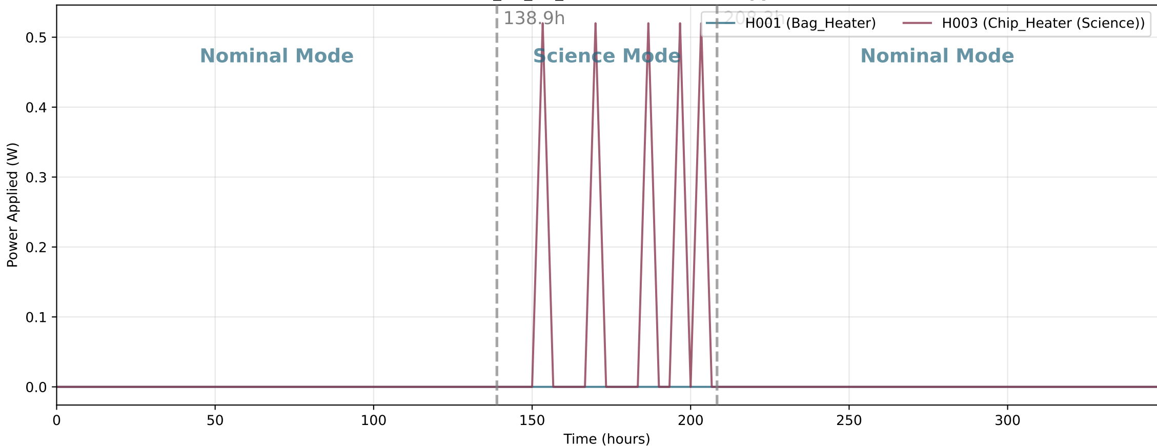
Acubesat_11_12_25 - Heater Power Applied
