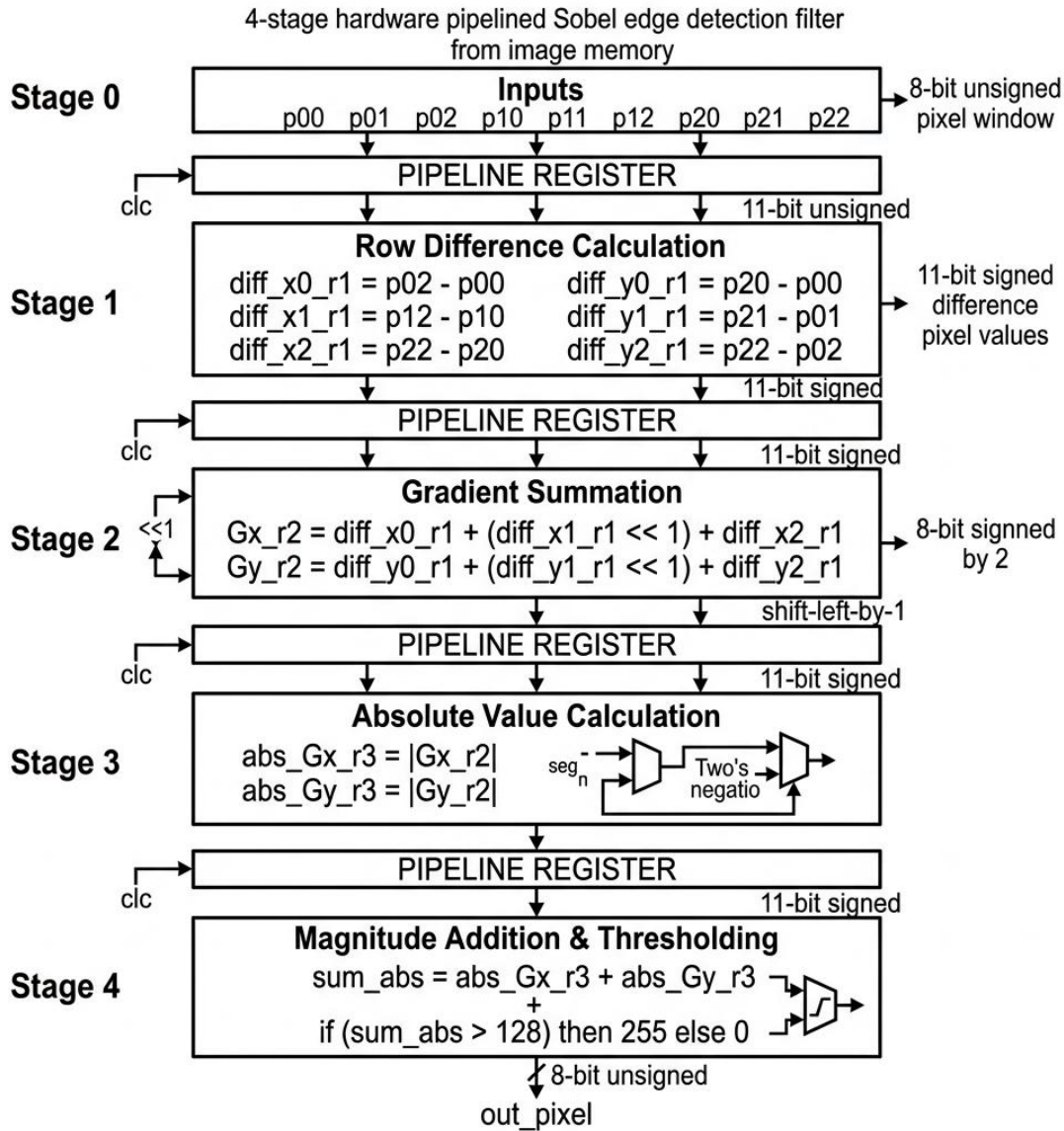
Figure: 4-Stage Pipeline Block Diagram
