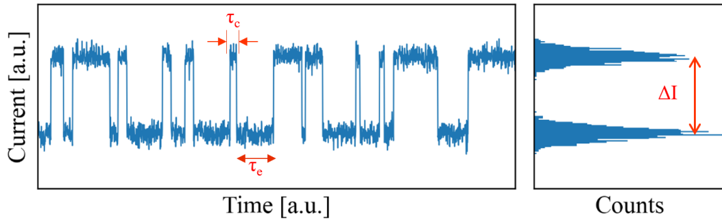
Figure 4: A classic example of (RTN) switching, illustrating the stochastic capture and emission times of charge carriers. The corresponding histogram reveals a characteristic bimodal current distribution.
