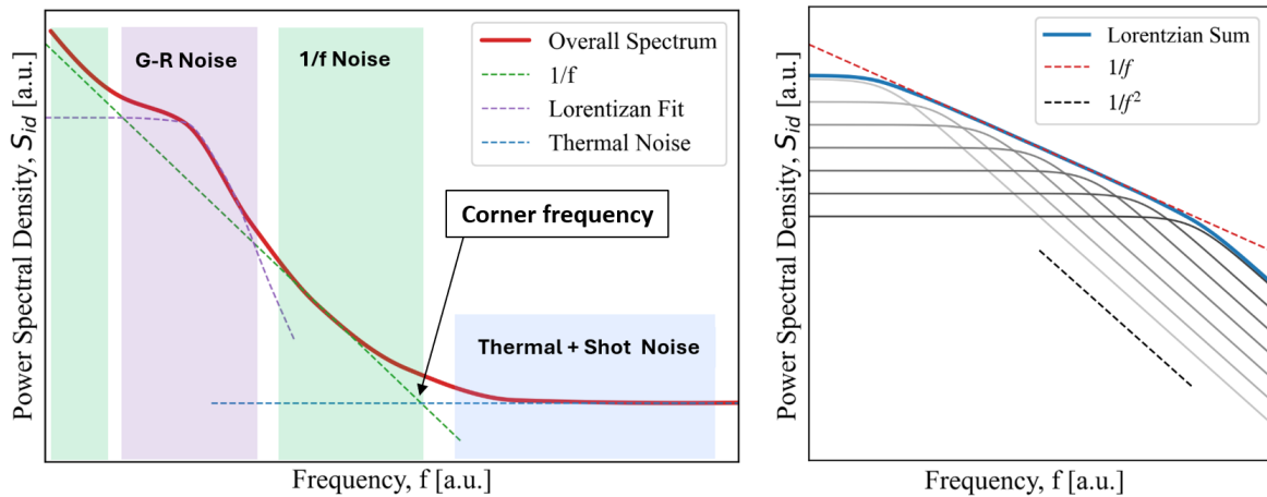
Figure 3: (a) Typical noise spectrum observed in semiconductor devices illustrating the dominant noise mechanisms across different frequency regimes. (b) Superposition of multiple Lorentzian spectra results in a 1/f -like behavior.
