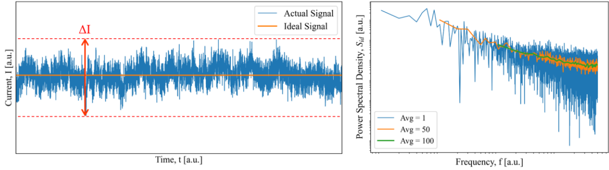
Figure 2: (a) Fluctuations in a transistor current in the time domain. (b) Power spectral density obtained from FFT with different averaging windows.
