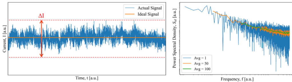
Figure 2: (a) Fluctuations in a transistor current in the time domain. (b) Power spectral density obtained from FFT with different averaging windows.
