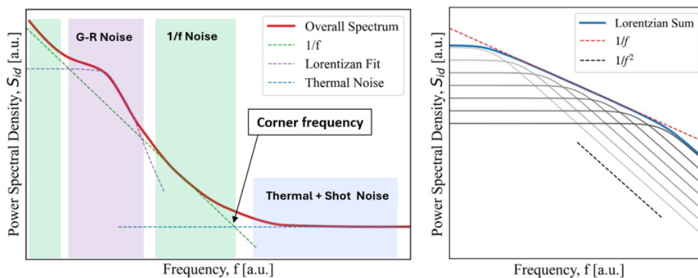
Figure 3: (a) Typical noise spectrum observed in semiconductor devices illustrating the dominant noise mechanisms across different frequency regimes. (b) Superposition of multiple Lorentzian spectra results in a 1/f -like behavior.
