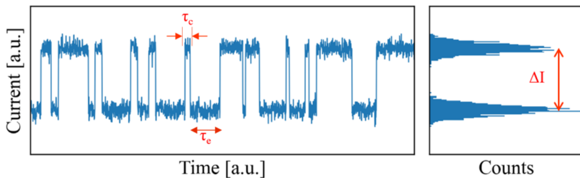
Figure 4: A classic example of RTN switching, illustrating the stochastic capture and emission times of charge carriers. The corresponding histogram reveals a characteristic bimodal current distribution.
